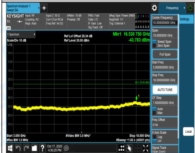
Band41(2555-2655)-20MHz-16QAM-40740-1RB#99-0.009-0.15-PASS
