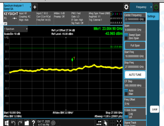
Band41(2555-2655)-20MHz-16QAM-40340-1RB#99-0.15-30-PASS
