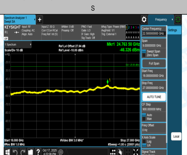
Band41(2555-2655)-20MHz-16QAM-40340-1RB#99-18000~27000-PAS
