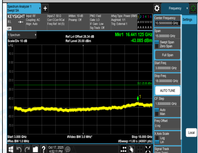
Band41(2555-2655)-20MHz-16QAM-41140-100RB#0-3000~18000-PA
