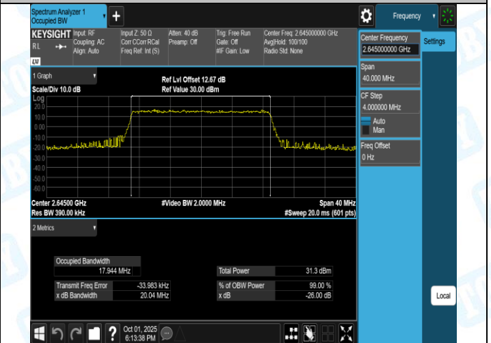
Band41(2555-2655)-20MHz-16QAM-41140-100RB#0-PASS
