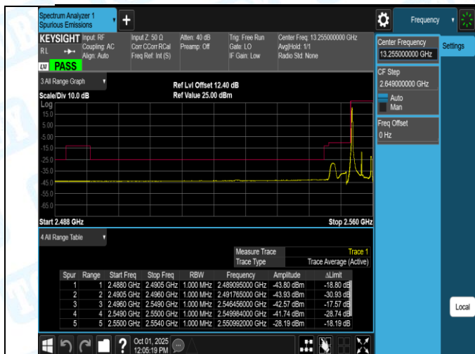
Band41(2555-2655)-5MHz-16QAM-40265-25RB#0-PASS
