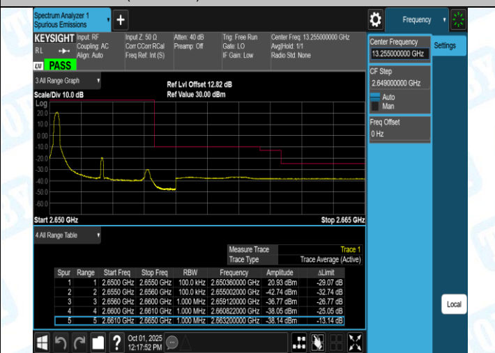
Band41(2555-2655)-5MHz-16QAM-41215-25RB#0-PASS
