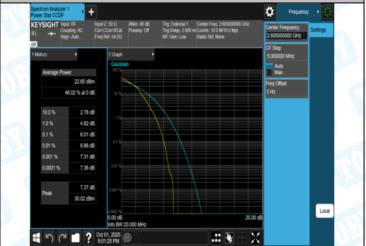
Band41(2555-2655)-20MHz-16QAM-41140-100RB#0-PASS
