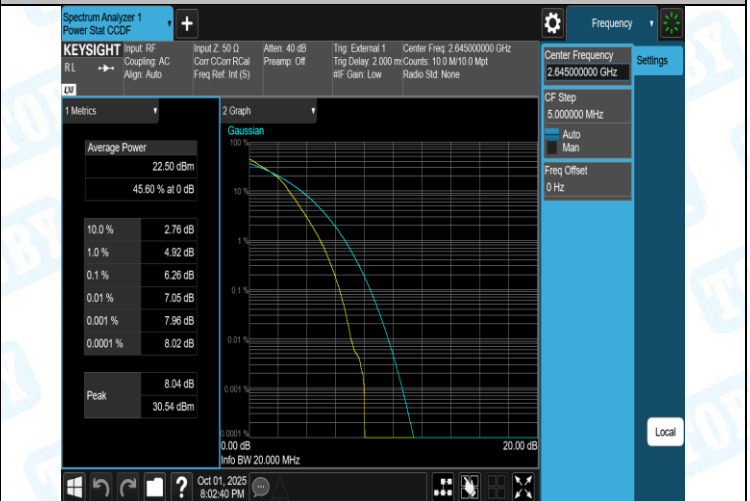
Band41(2555-2655)-20MHz-16QAM-41140-100RB#0-PASS
