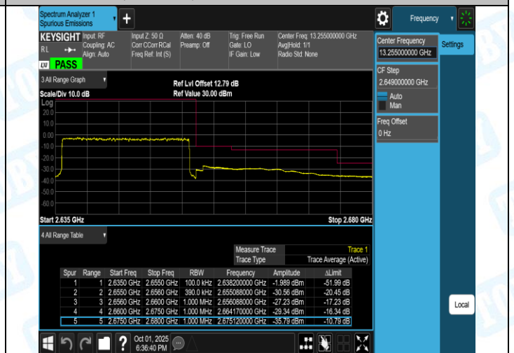
Band41(2555-2655)-20MHz-16QAM-41140-100RB#0-PASS
