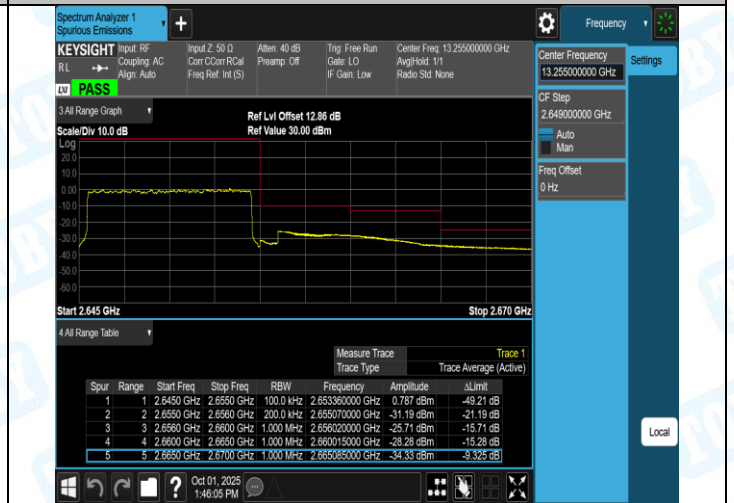
Band41(2555-2655)-15MHz-QPSK-40315-1RB#74-PASS
