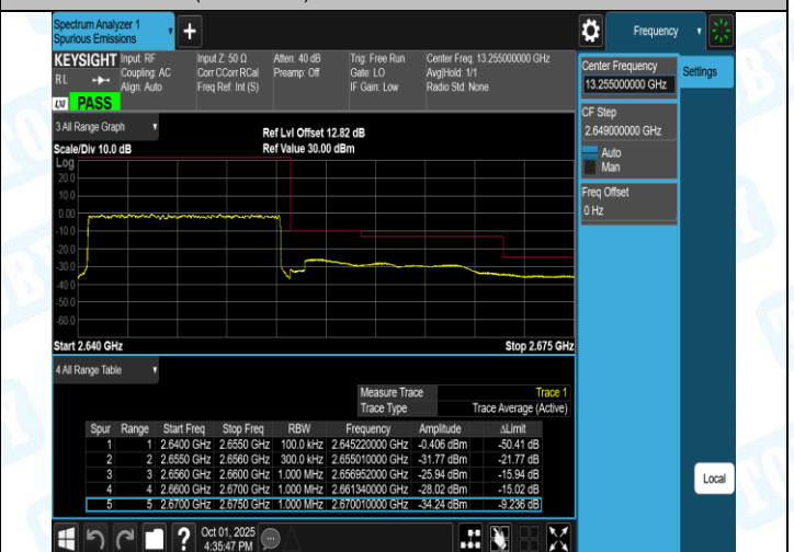
Band41(2555-2655)-15MHz-16QAM-40315-1RB#74-PASS
