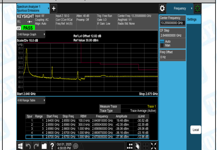
Band41(2555-2655)-15MHz-16QAM-41165-75RB#0-PASS
