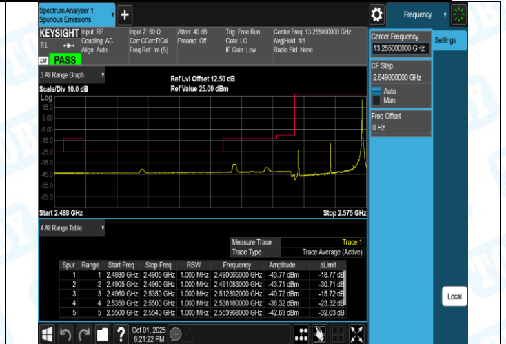
Band41(2555-2655)-20MHz-16QAM-41140-1RB#0-PASS
