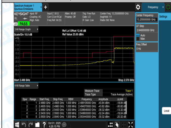
Band41(2555-2655)-15MHz-16QAM-41165-1RB#74-PASS
