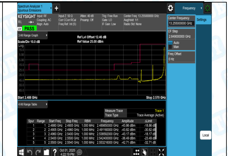
Band41(2555-2655)-15MHz-16QAM-41165-1RB#0-PASS
