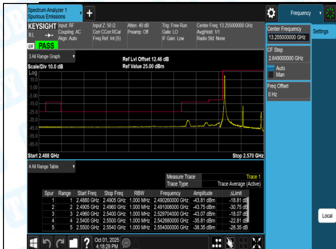
Band41(2555-2655)-15MHz-16QAM-40315-75RB#0-PASS
