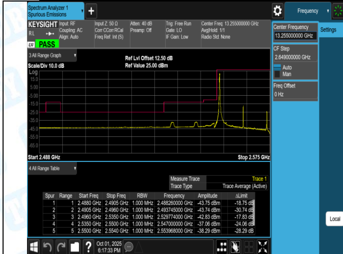
Band41(2555-2655)-20MHz-16QAM-40340-100RB#0-PASS
