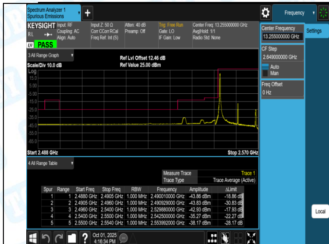
Band41(2555-2655)-15MHz-QPSK-40315-75RB#0-PASS
