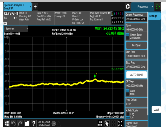
Band41(2555-2655)-5MHz-QPSK-40265-25RB#0-0.15~30-PASS
