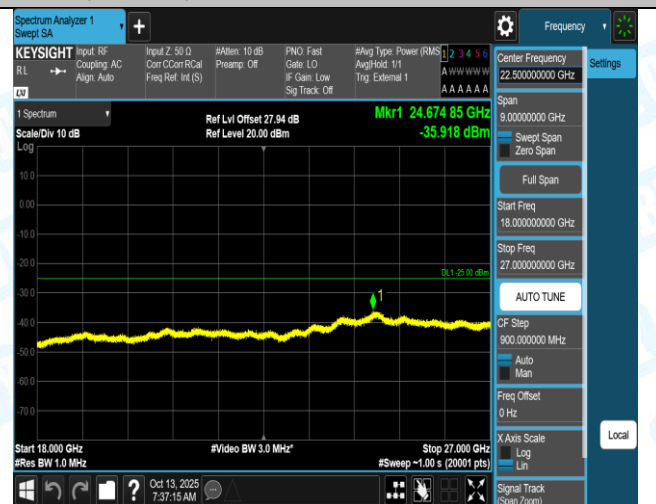
Band41(2555-2655)-5MHz-QPSK-40740-1RB#0-0.15~30-PASS
