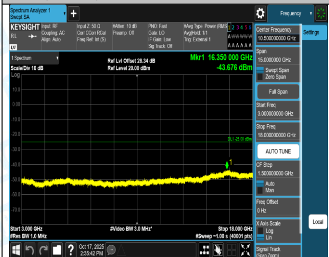
Band41(2555-2655)-5MHz-16QAM-40740-1RB#0-0.009-0.15-PASS
