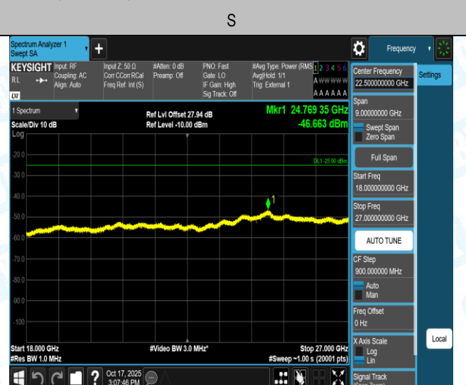
Band41(2555-2655)-10MHz-16QAM-40740-1RB#0-0.15~30-PASS
