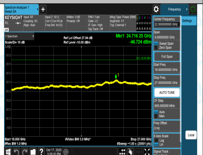
Band41(2555-2655)-10MHz-16QAM-41190-50RB#0-0.15~30-PASS
