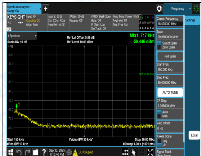
Band5-10MHz-QPSK-20450-1RB#49-1000~3000-PASS
