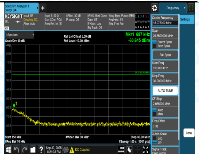
Band5-10MHz-16QAM-20525-1RB#0-1000~3000-PASS
