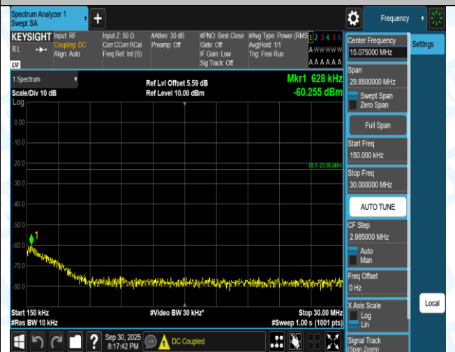
Band5-10MHz-16QAM-20450-1RB#49-1000~3000-PASS
