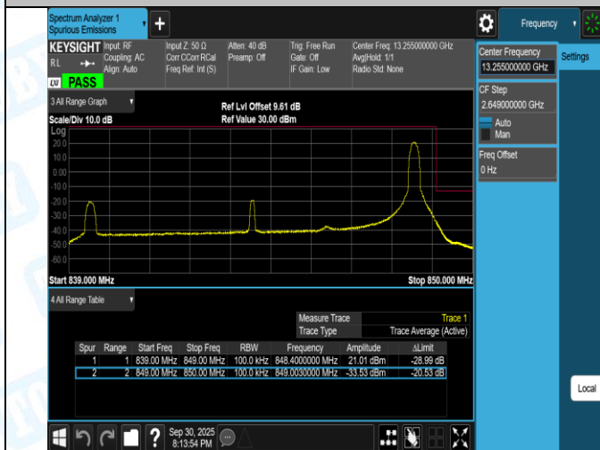
Band5-10MHz-16QAM-20600-1RB#49-PASS
