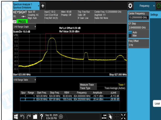
Band5-3MHz-16QAM-20415-15RB#0-PASS
