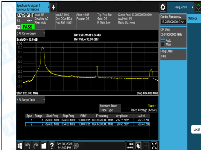
Band5-10MHz-16QAM-20450-50RB#0-PASS
