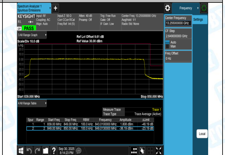
Band5-10MHz-16QAM-20600-50RB#0-PASS
