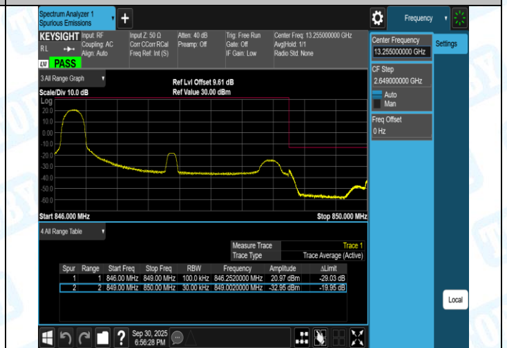
Band5-3MHz-16QAM-20635-15RB#0-PASS
