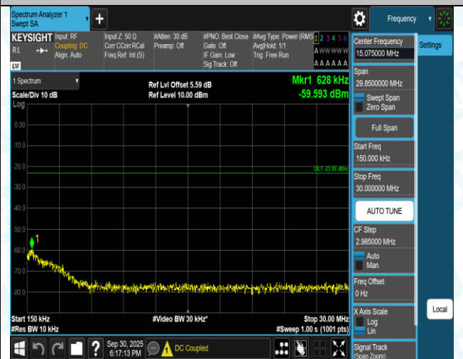
Band5-1.4MHz-16QAM-20407-1RB#5-1000~3000-PASS
