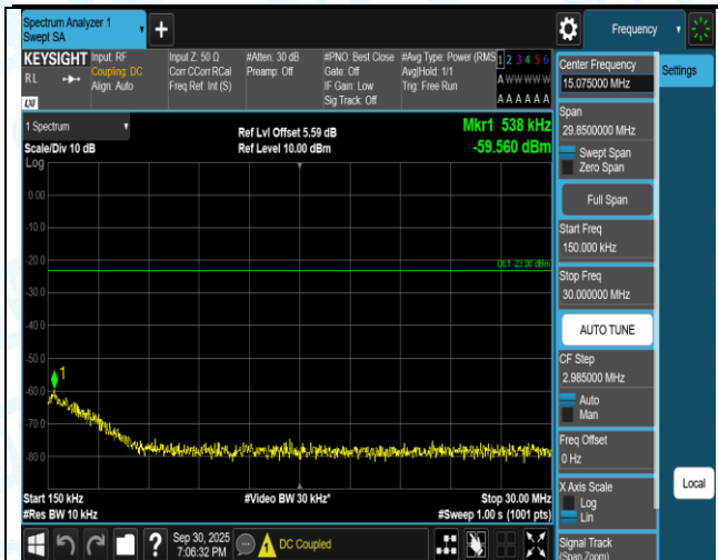
Band5-3MHz-16QAM-20525-1RB#14-1000-3000-PASS
