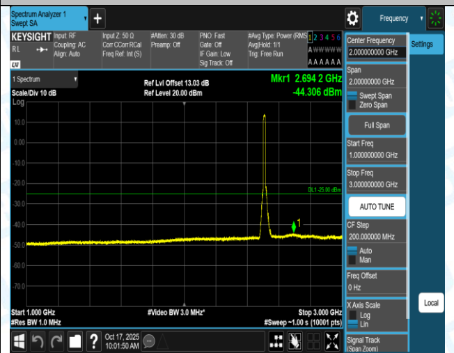
Band7-15MHz-16QAM-20825-75RB#0-18000~27000-PASS
