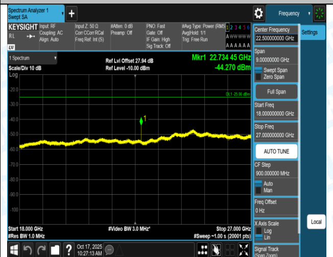
Band7-20MHz-16QAM-21100-1RB#99-0.15~30-PASS
