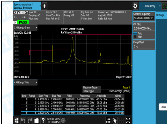
Band7-15MHz-16QAM-20825-75RB#0-PASS
