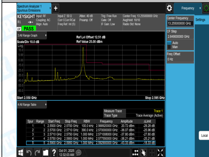
Band7-20MHz-16QAM-21350-1RB#99-PASS
