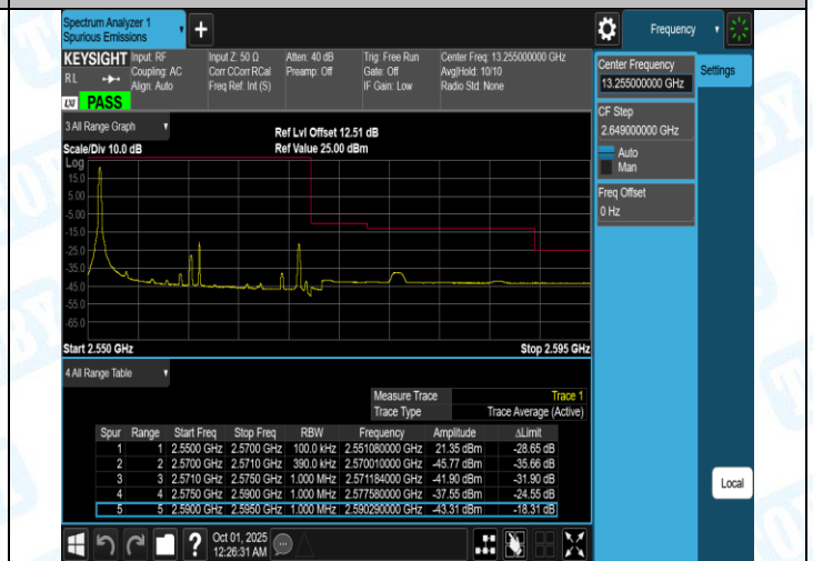
Band7-20MHz-QPSK-21350-100RB#0-PASS
