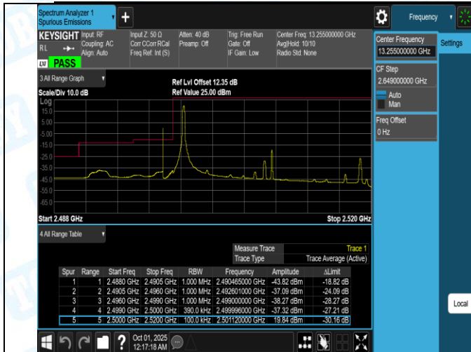
Band7-20MHz-16QAM-20850-100RB#0-PASS
