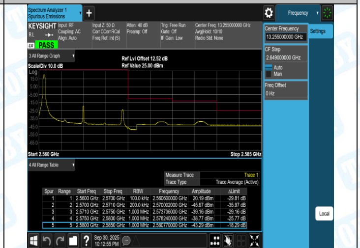
Band7-10MHz-16QAM-21400-50RB#0-PASS
