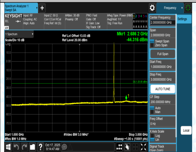
Band7-5MHz-QPSK-20775-1RB#24-18000~27000-PASS
