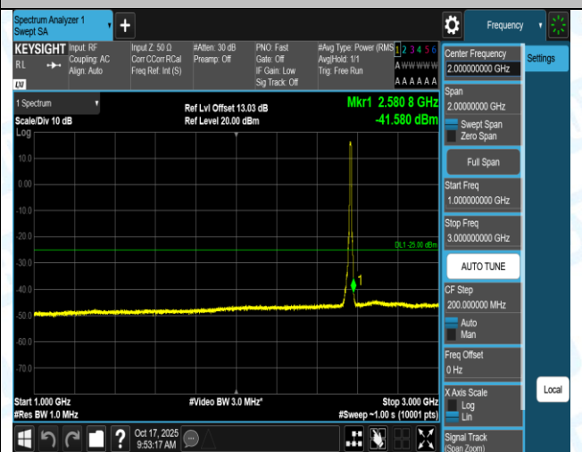
Band7-10MHz-QPSK-21400-50RB#0-18000~27000-PASS
