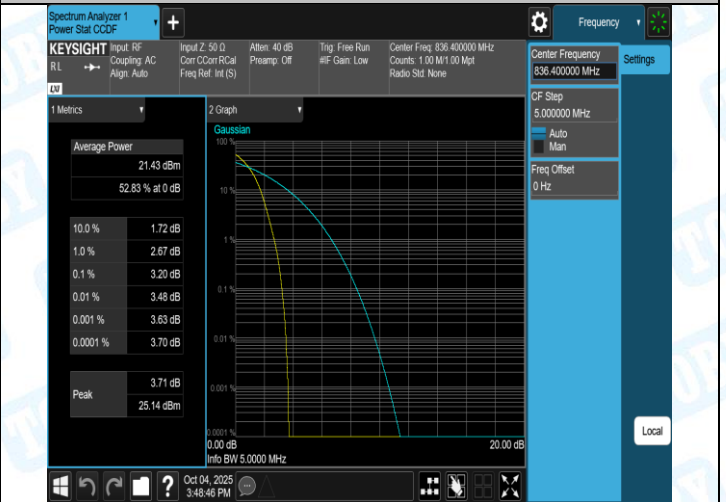
Band5-4182-PASS
