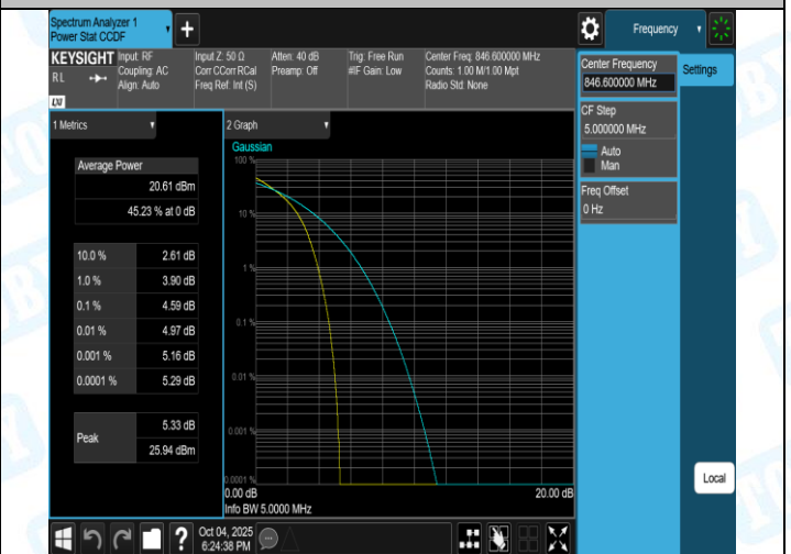
Band5-4233-4-PASS
