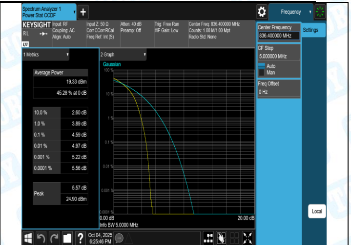
Band5-4182-5-PASS
