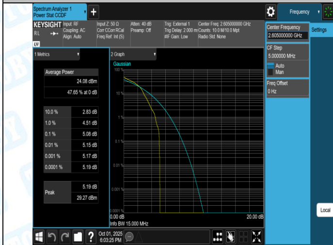
Band41(2555-2655)-15MHz-16QAM-41165-1RB#0-PASS
