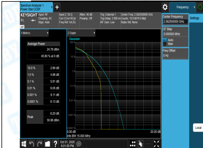
Band41(2555-2655)-15MHz-16QAM-40740-1RB#0-PASS
