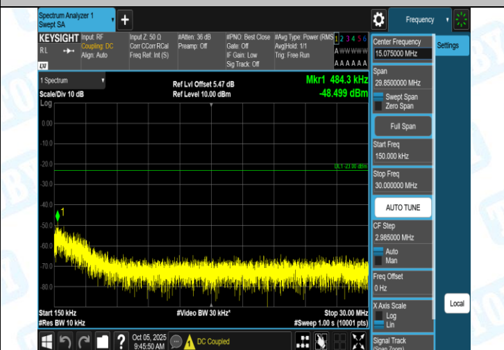
Band5-4233-5-0.15~30MHz-PASS
