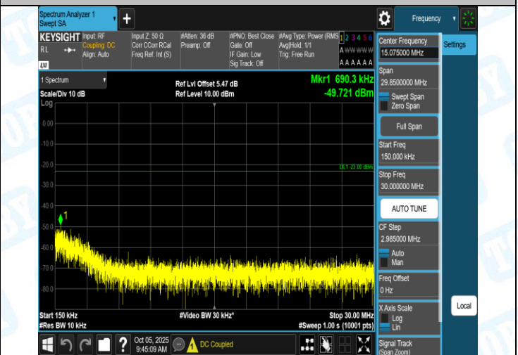
Band5-4182-5-0.15~30MHz-PASS
