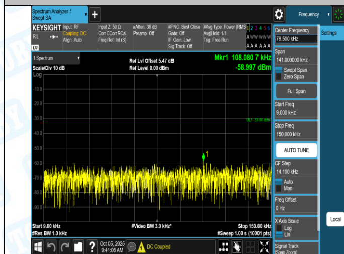
Band5-4233-3-0.009~0.15MHz-PASS
