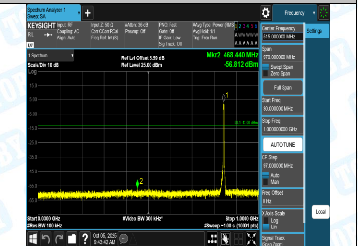
Band5-4233-4-30~1000MHz-PASS
