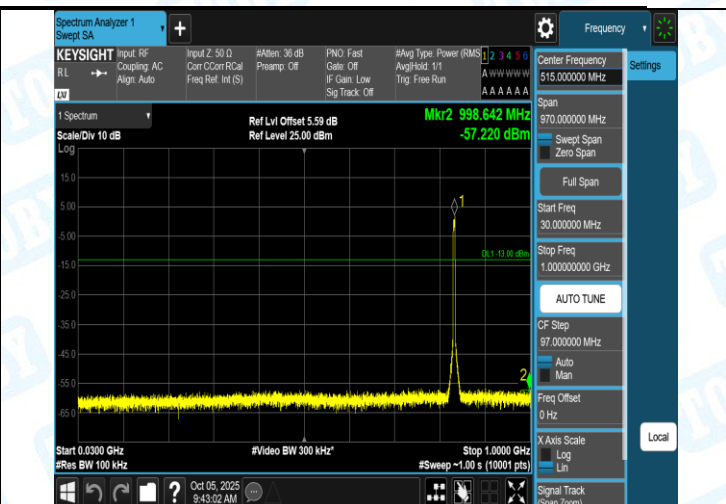
Band5-4182-4-30~1000MHz-PASS
