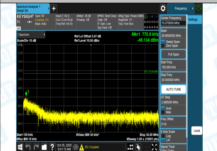
Band5-4233-3-0.15~30MHz-PASS
