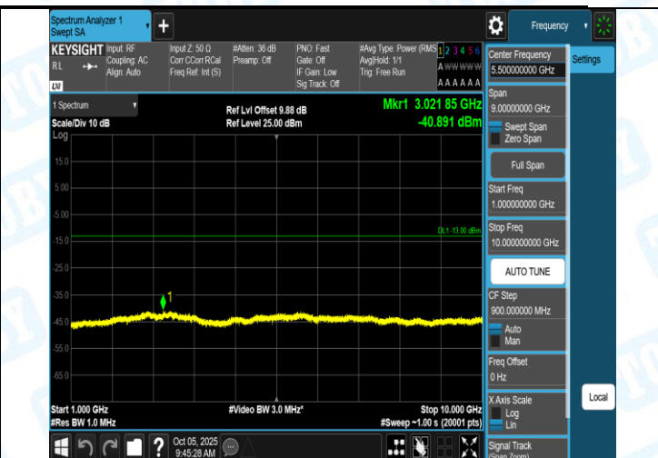
Band5-4182-5-1000~10000MHz-PASS
