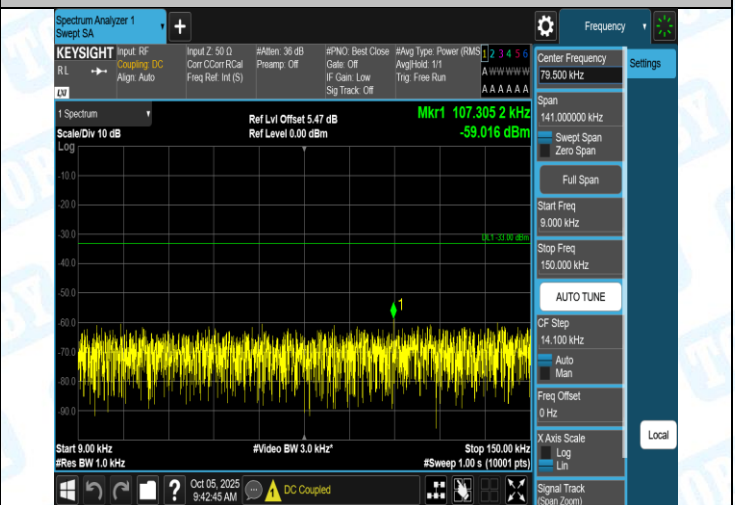
Band5-4182-4-0.009~0.15MHz-PASS
