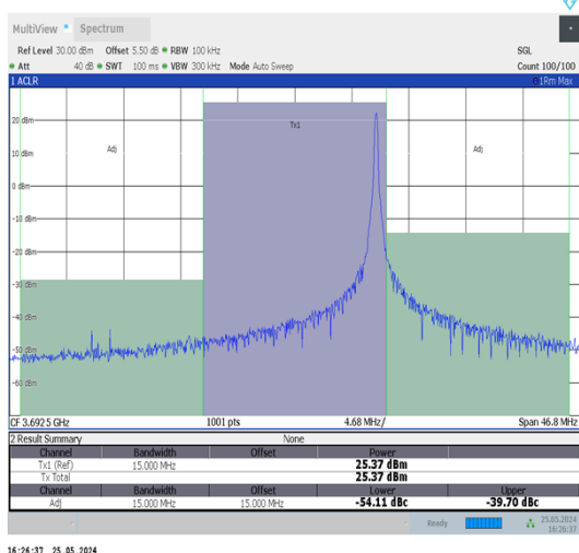
Band48-15MHz-QPSK-56665-1RB#74-PASS
