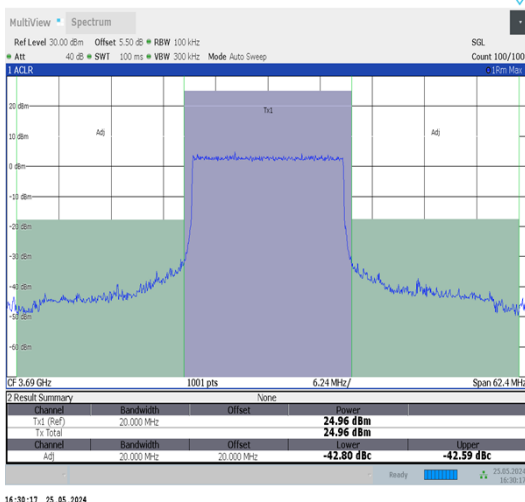
Band48-20MHz-QPSK-56640-100RB#0-PASS
