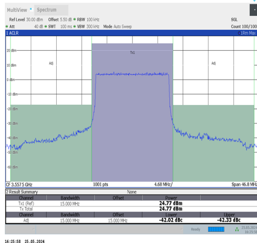
Band48-15MHz-QPSK-55315-75RB#0-PASS
