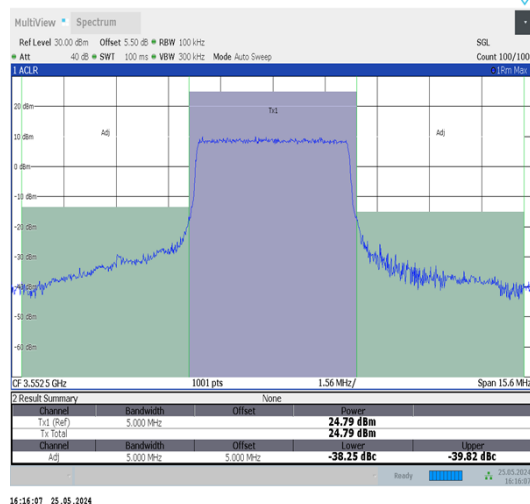
Band48-5MHz-QPSK-55265-25RB#0-PASS
