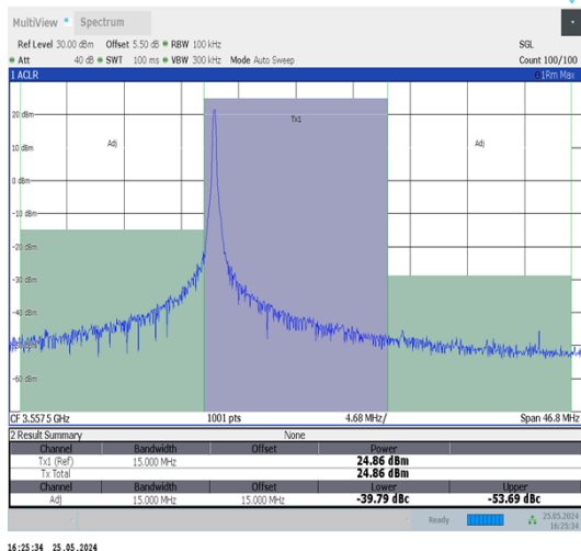
Band48-15MHz-QPSK-55315-1RB#0-PASS
