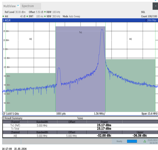
Band48-5MHz-QPSK-56715-1RB#24-PASS
