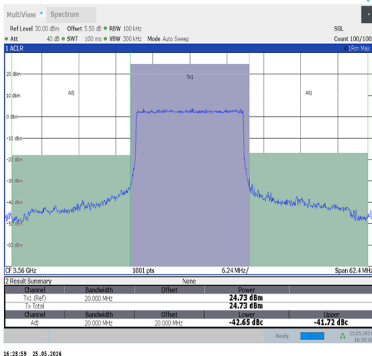
Band48-20MHz-QPSK-55340-100RB#0-PASS
