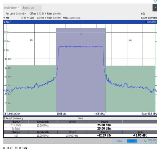
Band48-15MHz-QPSK-56665-75RB#0-PASS
