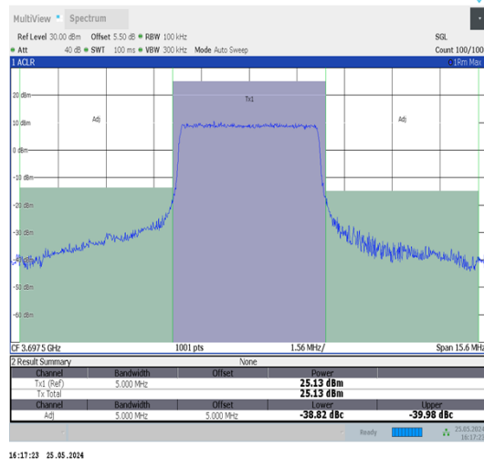
Band48-5MHz-QPSK-56715-25RB#0-PASS
