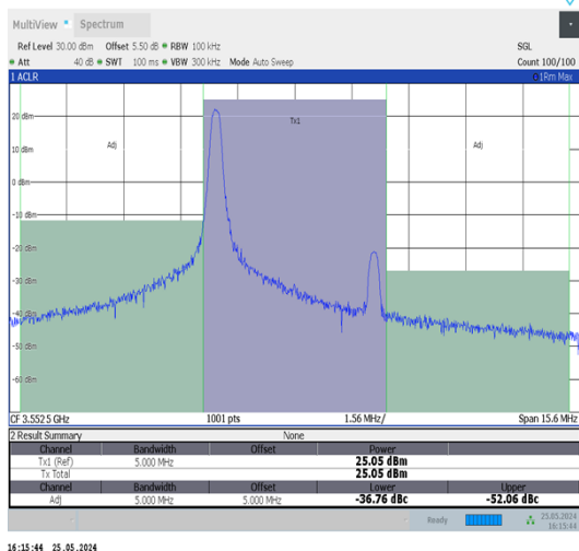
Band48-5MHz-QPSK-55265-1RB#0-PASS
