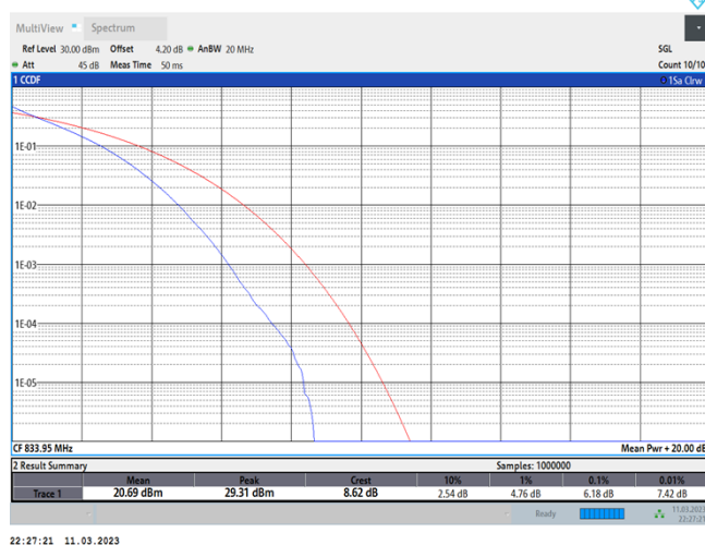
5-5-10MHz-10MHz-QPSK-QPSK-20476-20575-50RB#0-50RB#0
