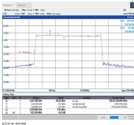
NTNV_CA_n41C_PC3_30+30_60+80_M+M_Ant1_TID8_1_#1
