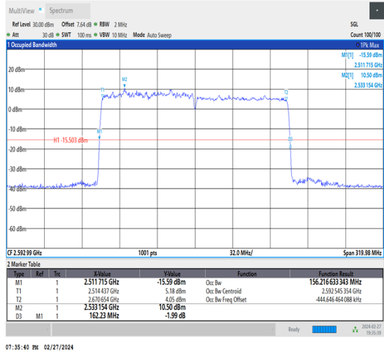
NTNV_CA_n41C_PC3_30+30_80+80_M+M_Ant1_TID8_1_#1
