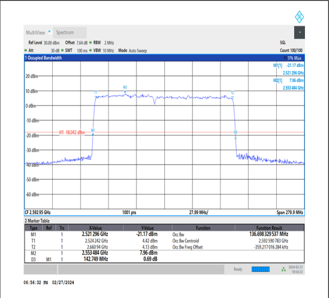
NTVN_CA_n41C_PC3_30+30_60+80_M+M_Ant1_TID4_1_#1
