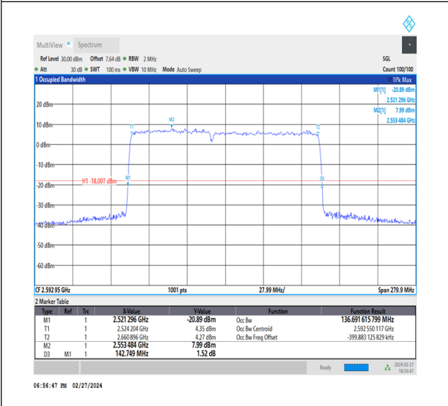
NTVN_CA_n41C_PC3_30+30_60+80_M+M_Ant1_TID5_1_#1
