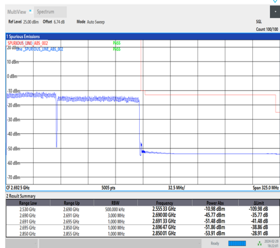
NTNV_CA_n41C_PC3_30+30_60+100_H+H_TID3_1_#1
