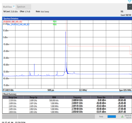
NTNV_CA_n41C_PC3_30+30_60+100_H+H_TID5_1_#1
