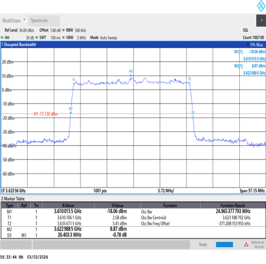
NTNV_CA_n48B_PC3_30+30_15+15_M+M_Ant0_TID3_1_#1
