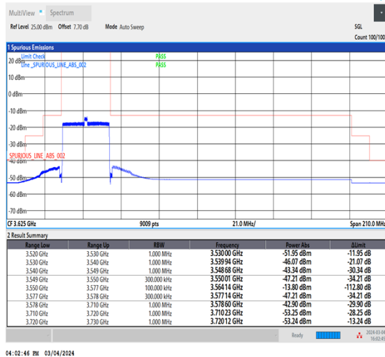
NTNV_CA_n48B_PC3_30+30_15+15_L+L_TID6_1_#1
