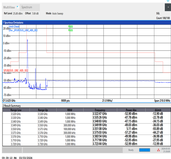
NTNV_CA_n48B_PC3_30+30_10+15_L+L_TID1_1_#1
