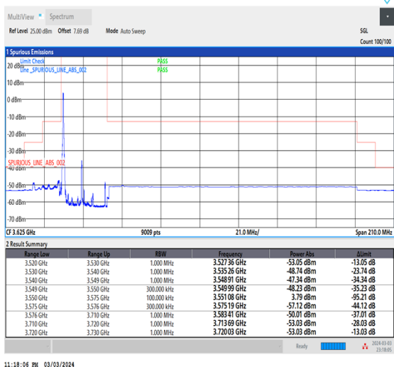
NTNV_CA_n48B_PC3_30+30_10+15_L+L_TID4_1_#1
