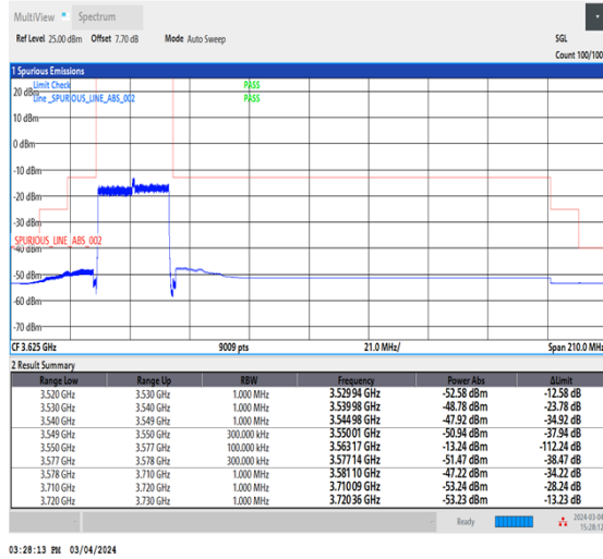
NTNV_CA_n48B_PC3_30+30_15+15_L+L_TID3_1_#1
