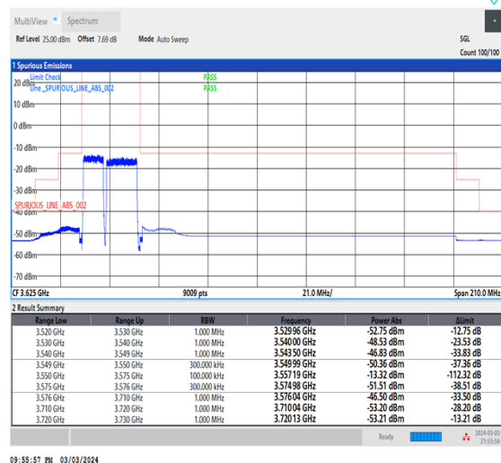
NTNV_CA_n48B_PC3_30+30_10+15_L+L_TID3_1_#1
