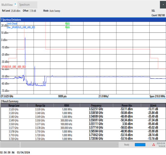
NTNV_CA_n48B_PC3_30+30_15+15_L+L_TID1_1_#1
