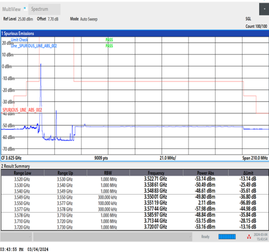
NTNV_CA_n48B_PC3_30+30_15+15_L+L_TID4_1_#1
