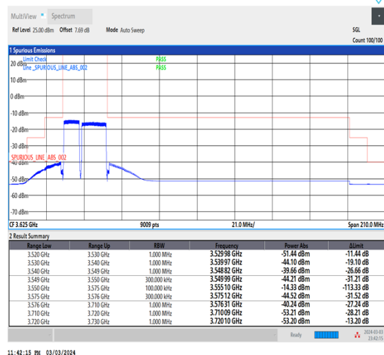
NTNV_CA_n48B_PC3_30+30_10+15_L+L_TID6_1_#1
