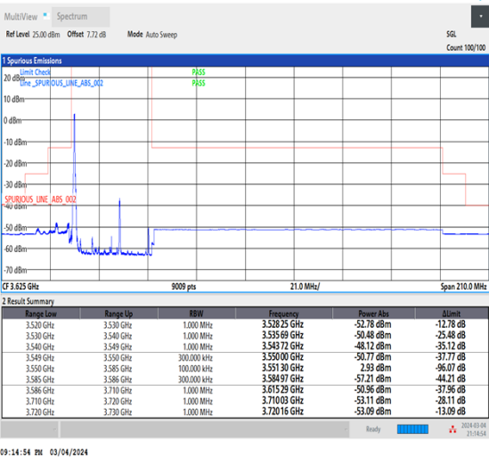
NTNV_CA_n48B_PC3_30+30_20+15_L+L_TID4_1_#1
