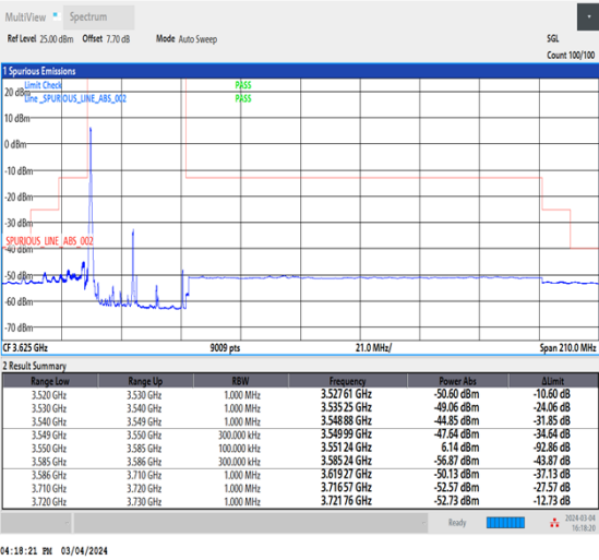
NTNV_CA_n48B_PC3_30+30_15+20_L+L_TID1_1_#1
