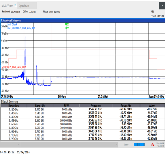
NTNV_CA_n48B_PC3_30+30_15+20_L+L_TID4_1_#1
