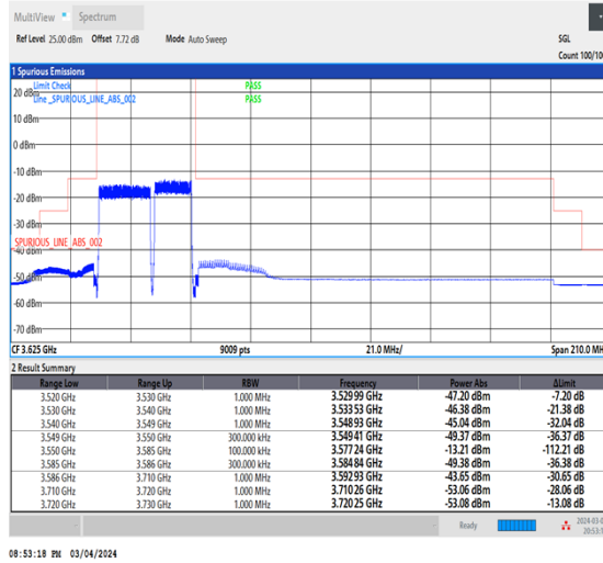
NTNV_CA_n48B_PC3_30+30_20+15_L+L_TID3_1_#1
