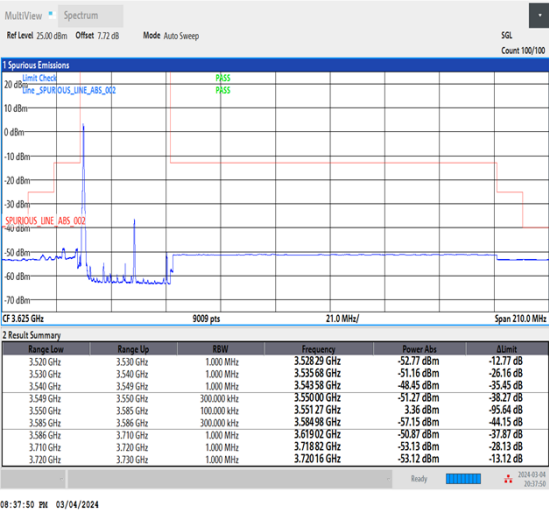
NTNV_CA_n48B_PC3_30+30_20+15_L+L_TID1_1_#1
