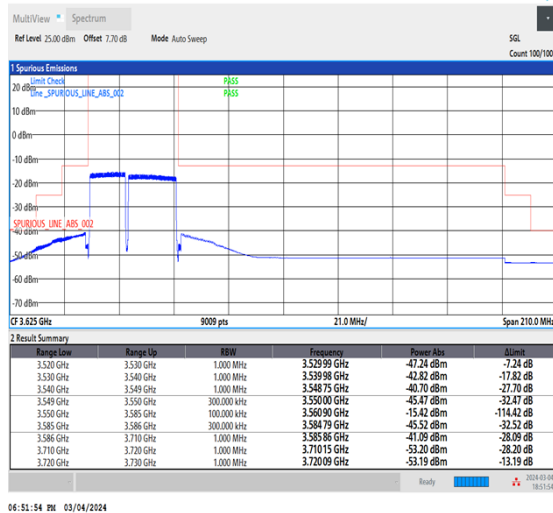
NTNV_CA_n48B_PC3_30+30_15+20_L+L_TID6_1_#1
