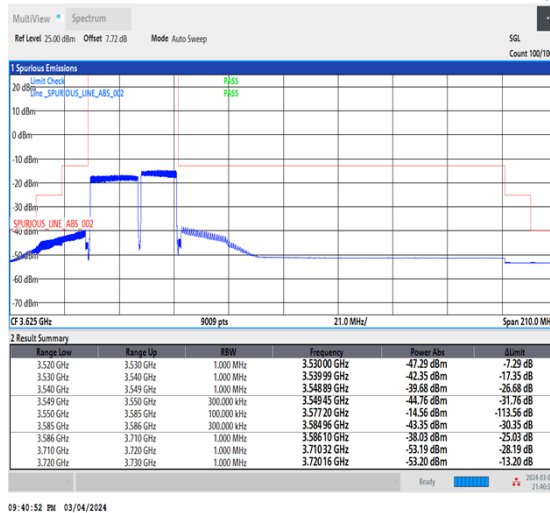
NTNV_CA_n48B_PC3_30+30_20+15_L+L_TID6_1_#1
