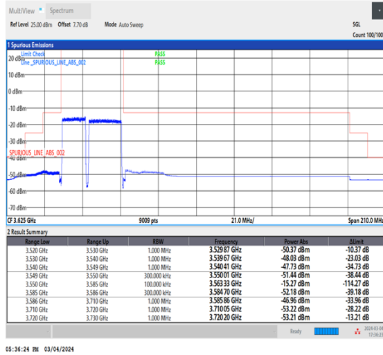
NTNV_CA_n48B_PC3_30+30_15+20_L+L_TID3_1_#1
