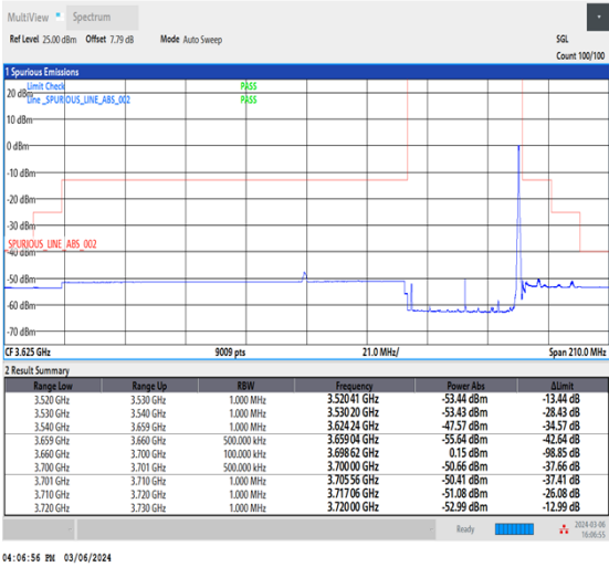
NTNV_CA_n48B_PC3_30+30_20+20_H+H_TID2_1_#1
