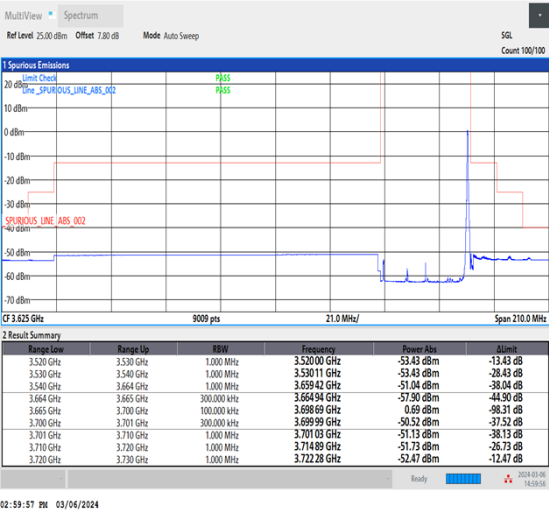
NTNV_CA_n48B_PC3_30+30_20+15_H+H_TID2_1_#1
