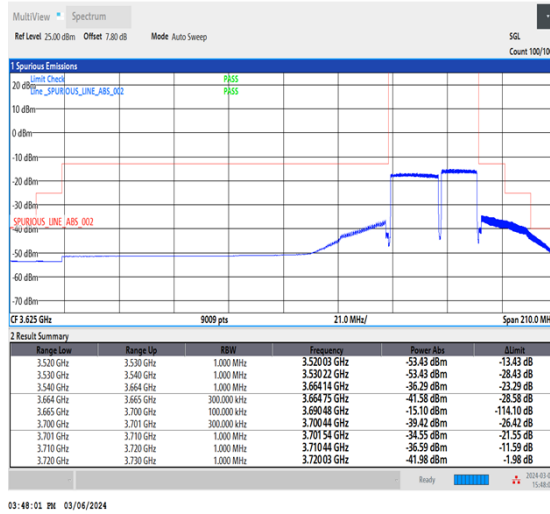
NTNV_CA_n48B_PC3_30+30_20+15_H+H_TID6_1_#1
