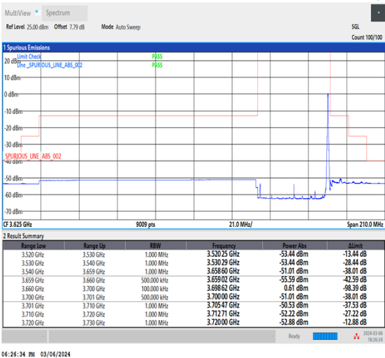
NTNV_CA_n48B_PC3_30+30_20+20_H+H_TID5_1_#1
