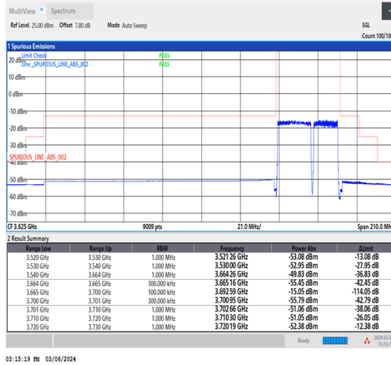
NTNV_CA_n48B_PC3_30+30_20+15_H+H_TID3_1_#1
