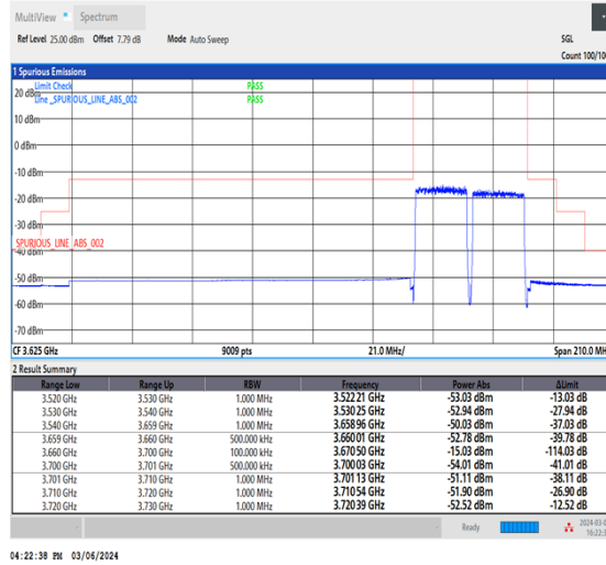
NTNV_CA_n48B_PC3_30+30_20+20_H+H_TID3_1_#1
