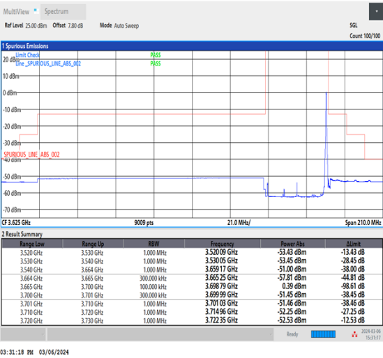
NTNV_CA_n48B_PC3_30+30_20+15_H+H_TID5_1_#1
