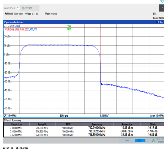
1-N12-PC3-15-5-H-6-CP-QPSK-Outer_Full-25@0-Ant7-1--PASS-see graph
