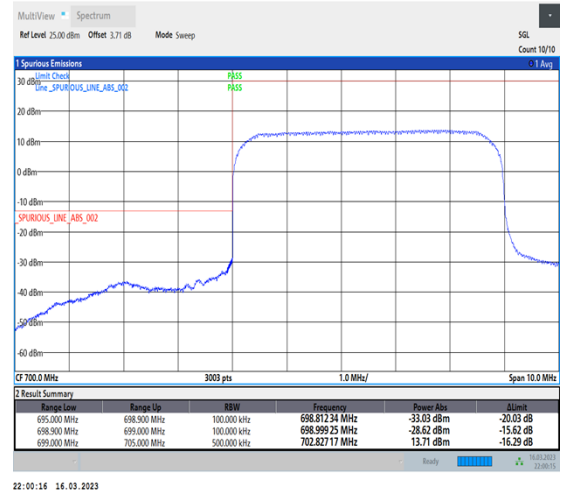
1-N12-PC3-15-5-L-3-DFT-PI2BPSK-Outer_Full-25@0-Ant7-1--PASS-see graph
