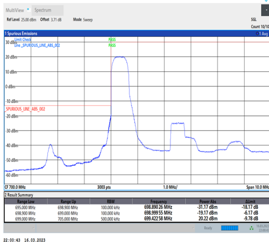
1-N12-PC3-15-5-L-4-CP-QPSK-Edge_1RB_Left-1@0-Ant7-1--PASS-see graph
