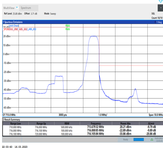
1-N12-PC3-15-5-H-5-CP-QPSK-Edge_1RB_Right-1@24-Ant7-1--PASS-see graph
