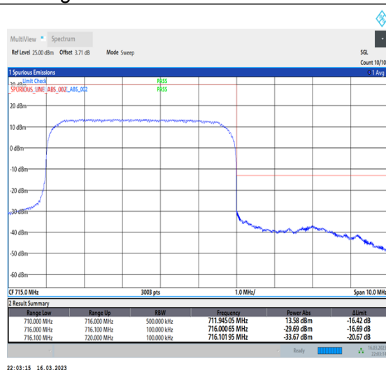
1-N12-PC3-15-5-H-3-DFT-PI2BPSK-Outer_Full-25@0-Ant7-1--PASS-see graph
