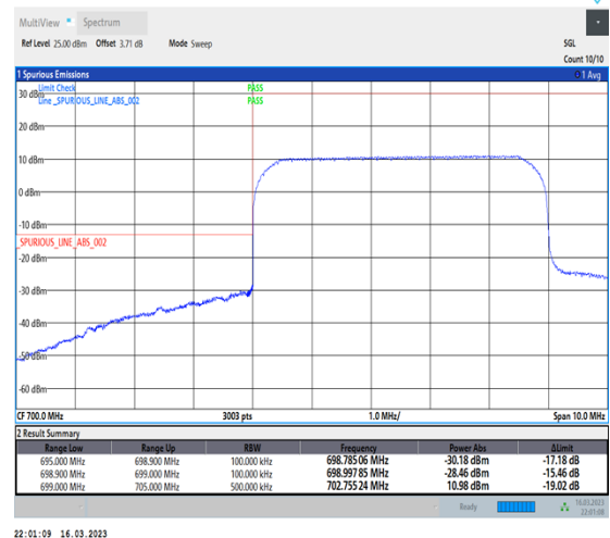
1-N12-PC3-15-5-L-6-CP-QPSK-Outer_Full-25@0-Ant7-1--PASS-see graph
