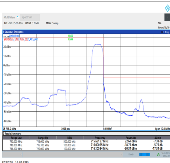
1-N12-PC3-15-5-H-2-DFT-PI2BPSK-Edge_1RB_Right-1@24-Ant7-1--PASS-see graph
