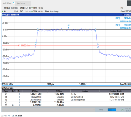
1-N2-PC3-15-5-L-1-DFT-QPSK-Outer_Full-25@0-Ant1-4.45-4.770-≤5-PASS
