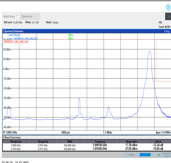
1-N2-PC3-15-10-H-5-CP-QPSK-Edge_1RB_Right-1@51-Ant1-1-seegraph-PASS-see graph
