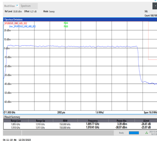
1-N2-15-15-H-3-DFT-PI2BPSK-Outer_Full-75@0-Ant1-1-seegraph-PASS-see graph
