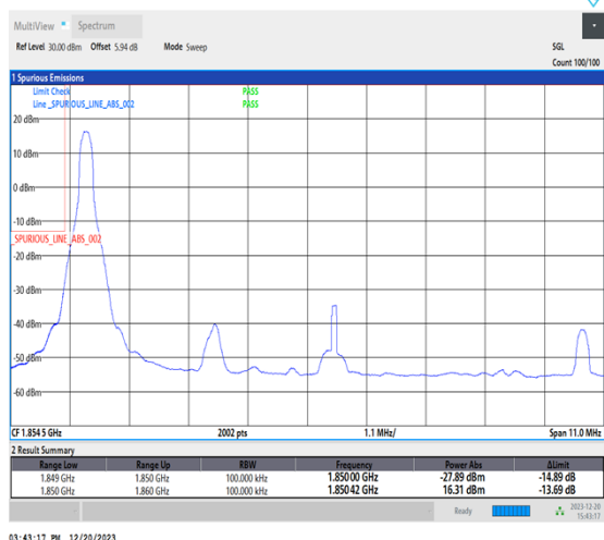
1-N2-15-10-L-4-CP-QPSK-Edge_1RB_Left-1@0-Ant1-1-seegraph-PASS-see graph
