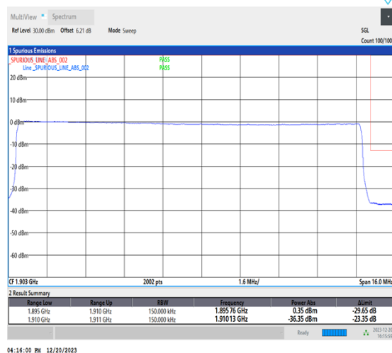
1-N2-15-15-H-6-CP-QPSK-Outer_Full-79@0-Ant1-1-seegraph-PASS-see graph
