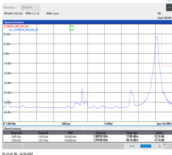
1-N2-15-15-H-5-CP-QPSK-Edge_1RB_Right-1@78-Ant1-1-seegraph-PASS-see graph
