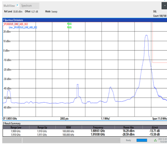
1-N2-15-10-H-5-CP-QPSK-Edge_1RB_Right-1@51-Ant1-1-seegraph-PASS-see graph
