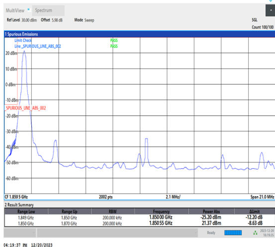
1-N2-15-20-L-1-DFT-PI2BPSK-Edge_1RB_Left-1@0-Ant1-1-seegraph-PASS-see graph
