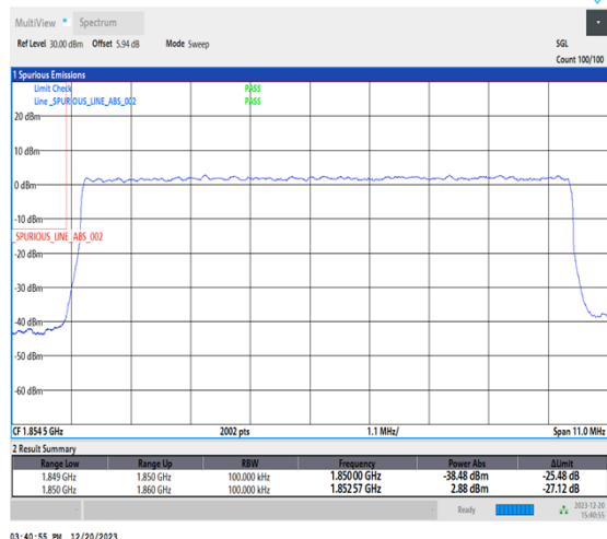
1-N2-15-10-L-3-DFT-PI2BPSK-Outer_Full-50@0-Ant1-1-seegraph-PASS-see graph
