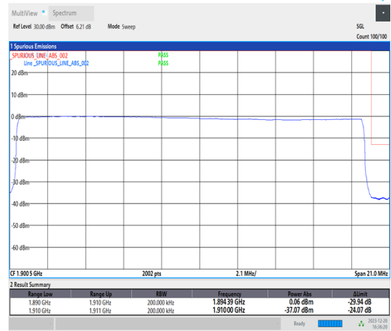
1-N2-15-20-H-6-CP-QPSK-Outer_Full-106@0-Ant1-1-seegraph-PASS-see graph
