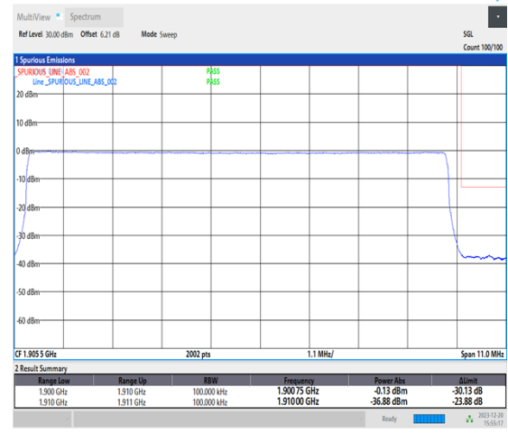
1-N2-15-10-H-6-CP-QPSK-Outer_Full-52@0-Ant1-1-seegraph-PASS-see graph
