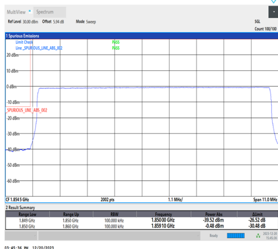
1-N2-15-10-L-6-CP-QPSK-Outer_Full-52@0-Ant1-1-seegraph-PASS-see graph
