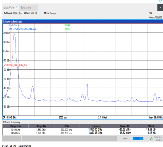
1-N2-15-20-L-4-CP-QPSK-Edge_1RB_Left-1@0-Ant1-1-seegraph-PASS-see graph
