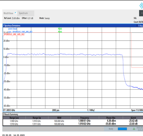
1-N2-PC3-15-10-H-3-DFT-PI2BPSK-Outer_Full-50@0-Ant1-1-seegraph-PASS-see graph
