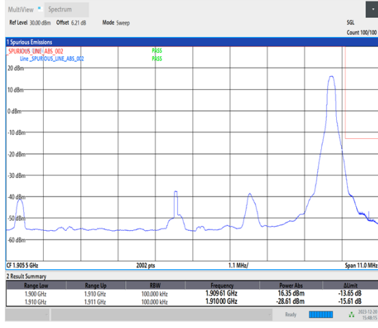
1-N2-15-10-H-2-DFT-PI2BPSK-Edge_1RB_Right-1@51-Ant1-1-seegraph-PASS-see graph
