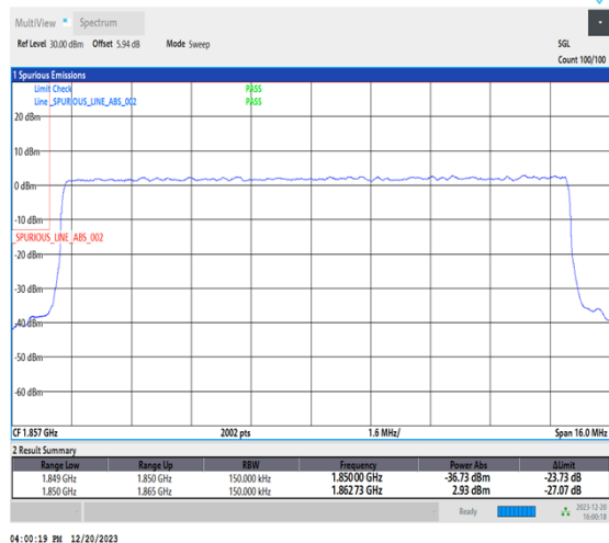
1-N2-15-15-L-3-DFT-PI2BPSK-Outer_Full-75@0-Ant1-1-seegraph-PASS-see graph
