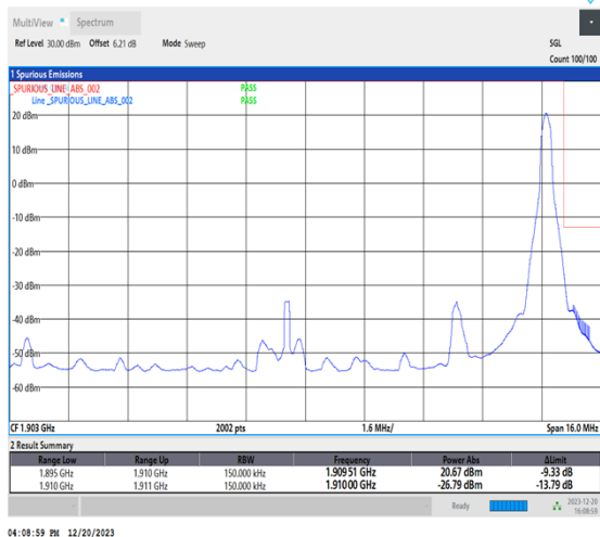
1-N2-15-15-H-2-DFT-PI2BPSK-Edge_1RB_Right-1@78-Ant1-1-seegraph-PASS-see graph
