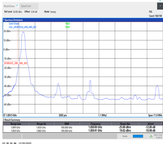
1-N2-15-10-L-1-DFT-PI2BPSK-Edge_1RB_Left-1@0-Ant1-1-seegraph-PASS-see graph
