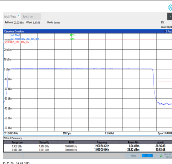
1-N2-PC3-15-10-H-6-CP-QPSK-Outer_Full-52@0-Ant1-1-seegraph-PASS-see graph
