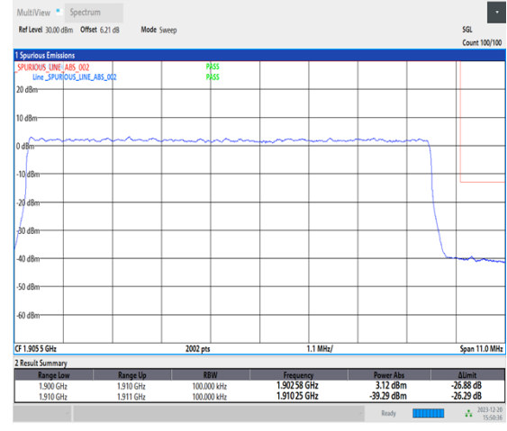
1-N2-15-10-H-3-DFT-PI2BPSK-Outer_Full-50@0-Ant1-1-seegraph-PASS-see graph
