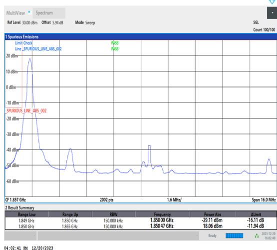
1-N2-15-15-L-4-CP-QPSK-Edge_1RB_Left-1@0-Ant1-1-seegraph-PASS-see graph
