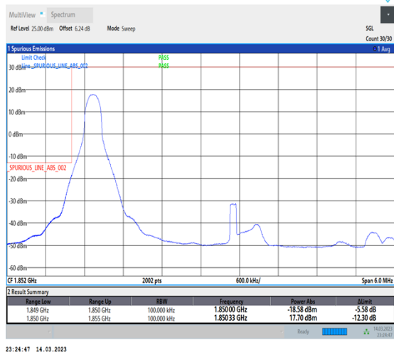
1-N2-PC3-15-5-L-4-CP-QPSK-Edge_1RB_Left-1@0-Ant1-1-seegraph-PASS-see graph
