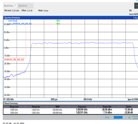
1-N2-PC3-15-5-L-3-DFT-PI2BPSK-Outer_Full-25@0-Ant1-1-seegraph-PASS-see graph
