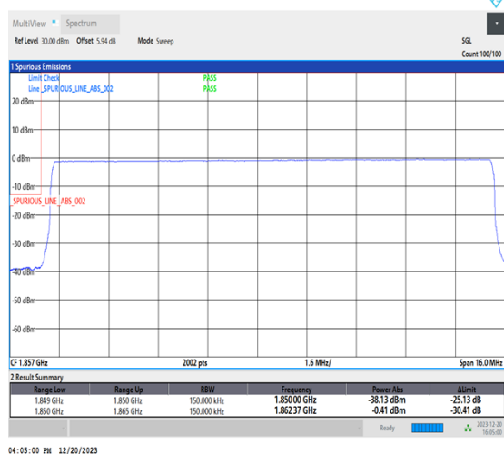
1-N2-15-15-L-6-CP-QPSK-Outer_Full-79@0-Ant1-1-seegraph-PASS-see graph
