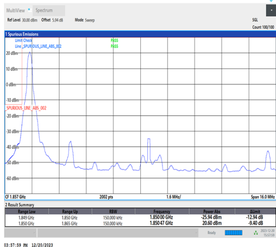
1-N2-15-15-L-1-DFT-PI2BPSK-Edge_1RB_Left-1@0-Ant1-1-seegraph-PASS-see graph
