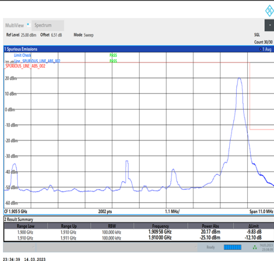
1-N2-PC3-15-10-H-2-DFT-PI2BPSK-Edge_1RB_Right-1@51-Ant1-1-seegraph-PASS-see graph
