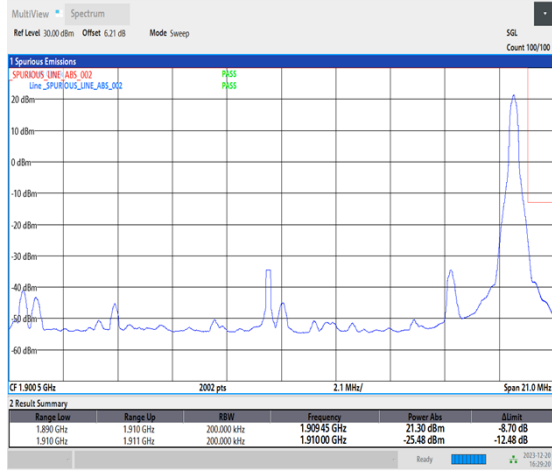
1-N2-15-20-H-2-DFT-PI2BPSK-Edge_1RB_Right-1@105-Ant1-1-seegraph-PASS-see graph
