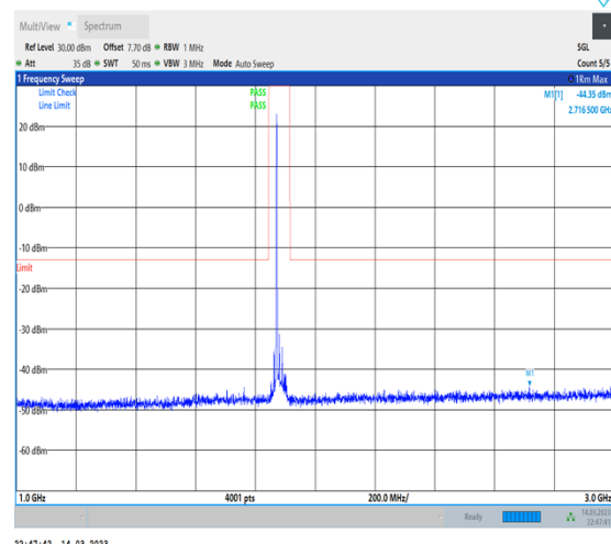
1-N2-PC3-15-20-M-1-DFT-PI2BPSK-Inner_1RB_Left- 1@1-1000-3000-Ant1-2716.50--44.35--13-PASS
