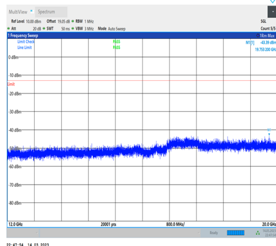
1-N2-PC3-15-20-M-1-DFT-PI2BPSK-Inner_1RB_Left- 1@1-12000-20000-Ant1-19753.20--43.39--13-PASS
