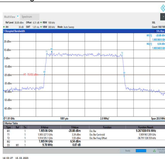
1-N25-PC3-15-10-H-9-CP-256QAM-Outer_Full- 52@0-Ant1-9.268-9.780-≤10-PASS
