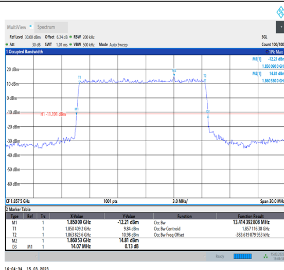
1-N25-PC3-15-15-L-2-DFT-PI2BPSK-Outer_Full- 75@0-Ant1-13.414-14.070-≤15-PASS
