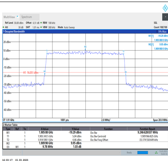
1-N25-PC3-15-10-H-8-CP-64QAM-Outer_Full- 52@0-Ant1-9.247-9.780-≤10-PASS
