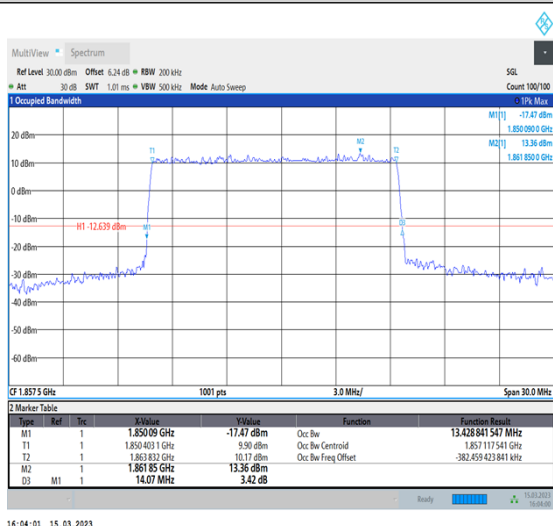
1-N25-PC3-15-15-L-1-DFT-QPSK-Outer_Full-75@0- Ant1-13.429-14.070-≤15-PASS
