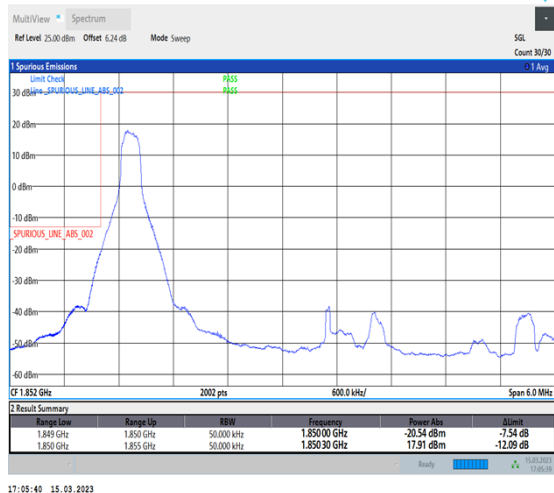
1-N25-PC3-15-5-L-1-DFT-PI2BPSK-Edge_1RB_Left-1@0-Ant1-1-seegraph-PASS-see graph
