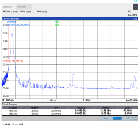
1-N25-PC3-15-20-L-4-CP-QPSK-Edge_1RB_Left-1@0-Ant1-1-seegraph-PASS-see graph
