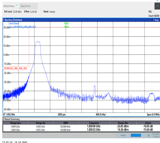
1-N25-PC3-15-5-L-4-CP-QPSK-Edge_1RB_Left-1@0-Ant1-1-seegraph-PASS-see graph
