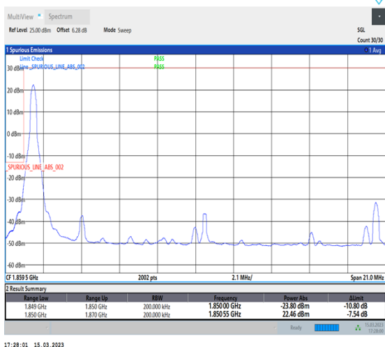
1-N25-PC3-15-20-L-1-DFT-PI2BPSK-Edge_1RB_Left-1@0-Ant1-1-seegraph-PASS-see graph
