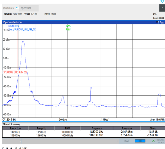
1-N25-PC3-15-10-L-4-CP-QPSK-Edge_1RB_Left-1@0-Ant1-1-seegraph-PASS-see graph
