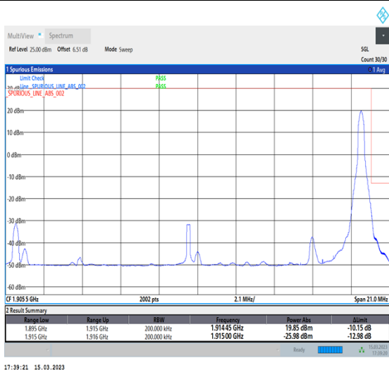
1-N25-PC3-15-20-H-5-CP-QPSK-Edge_1RB_Right-1@105-Ant1-1-seegraph-PASS-see graph
