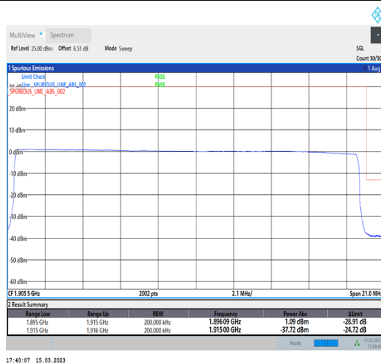
1-N25-PC3-15-20-H-6-CP-QPSK-Outer_Full-106@0-Ant1-1-seegraph-PASS-see graph
