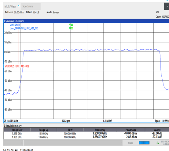
1-N25-15-10-L-3-DFT-PI2BPSK-Outer_Full-50@0-Ant1-1-seegraph-PASS-see graph
