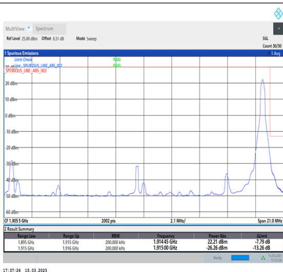
1-N25-PC3-15-20-H-2-DFT-PI2BPSK-Edge_1RB_Right-1@105-Ant1-1-seegraph-PASS-see graph
