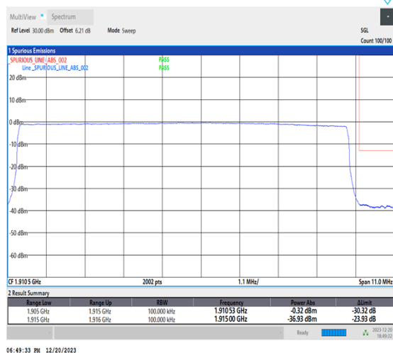
1-N25-15-10-H-6-CP-QPSK-Outer_Full-52@0-Ant1-1-seegraph-PASS-see graph
