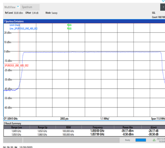
1-N25-15-10-L-6-CP-QPSK-Outer_Full-52@0-Ant1-1-seegraph-PASS-see graph
