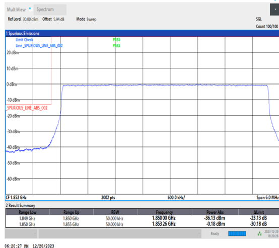
1-N25-15-5-L-6-CP-QPSK-Outer_Full-25@0-Ant1-1-seegraph-PASS-see graph
