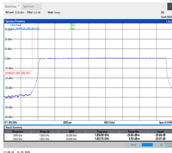
1-N25-PC3-15-5-L-6-CP-QPSK-Outer_Full-25@0-Ant1-1-seegraph-PASS-see graph
