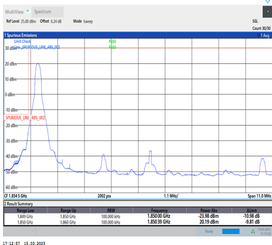
1-N25-PC3-15-10-L-1-DFT-PI2BPSK-Edge_1RB_Left-1@0-Ant1-1-seegraph-PASS-see graph
