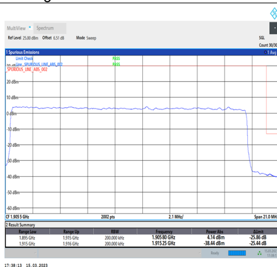
1-N25-PC3-15-20-H-3-DFT-PI2BPSK-Outer_Full-100@0-Ant1-1-seegraph-PASS-see graph
