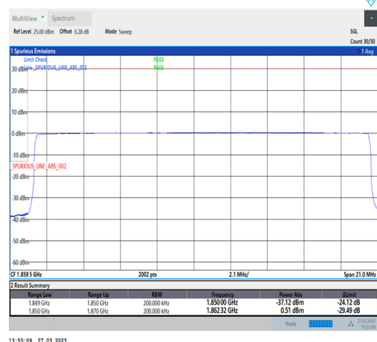
1-N25-PC3-15-20-L-6-CP-QPSK-Outer_Full-106@0-Ant1-1-seegraph-PASS-see graph
