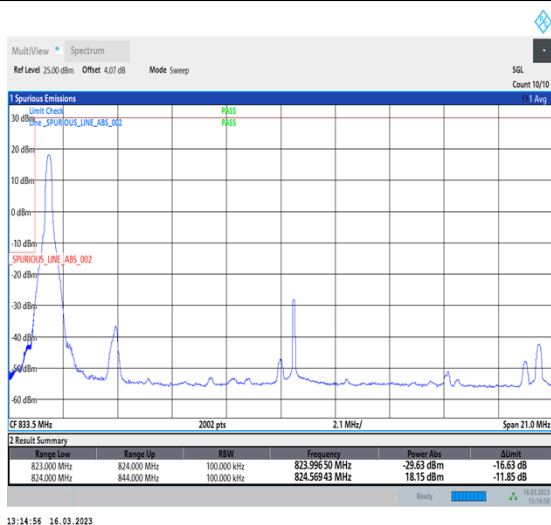
1-N26-824-849-PC3-15-20-L-4-CP-QPSK-Edge_1RB_Left-1@0-Ant1-1-seegraph-PASS-see graph
