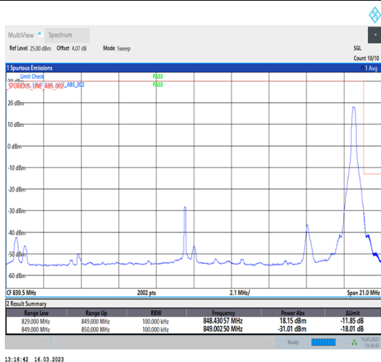
1-N26-824-849-PC3-15-20-H-5-CP-QPSK-Edge_1RB_Right-1@105-Ant1-1-seegraph-PASS-see graph
