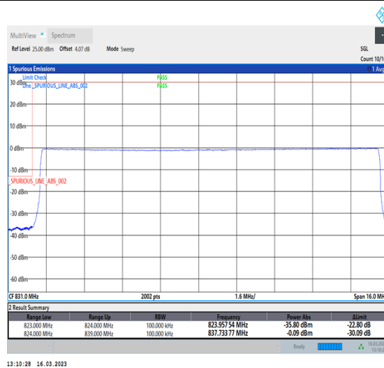
1-N26-824-849-PC3-15-15-L-6-CP-QPSK-Outer_Full-79@0-Ant1-1-seegraph-PASS-see graph
