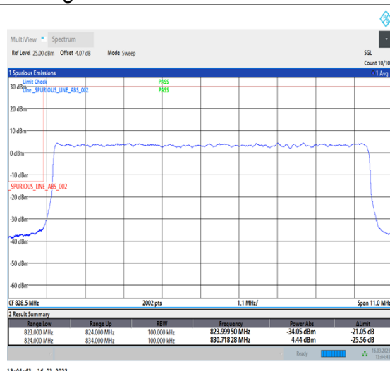
1-N26-824-849-PC3-15-10-L-3-DFT-PI2BPSK-Outer_Full-50@0-Ant1-1-seegraph-PASS-see graph
