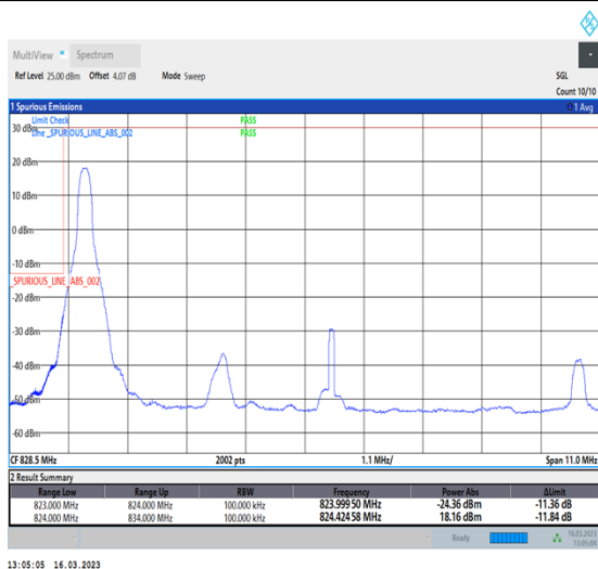
1-N26-824-849-PC3-15-10-L-4-CP-QPSK-Edge_1RB_Left-1@0-Ant1-1-seegraph-PASS-see graph
