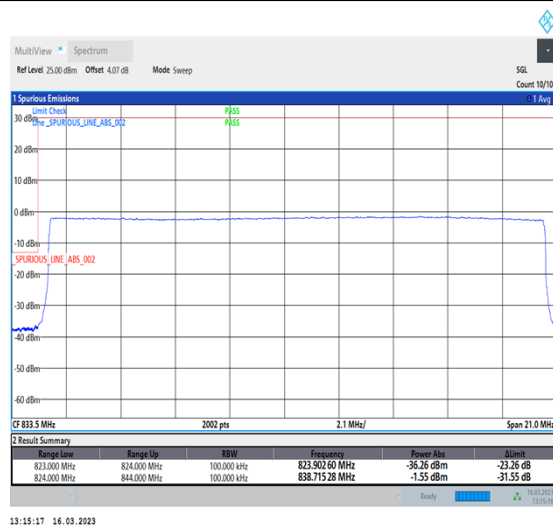
1-N26-824-849-PC3-15-20-L-6-CP-QPSK-Outer_Full-106@0-Ant1-1-seegraph-PASS-see graph
