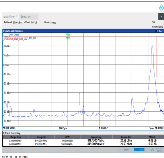
1-N26-824-849-PC3-15-20-H-2-DFT-PI2BPSK-Edge_1RB_Right-1@105-Ant1-1-seegraph-PASS-see graph
