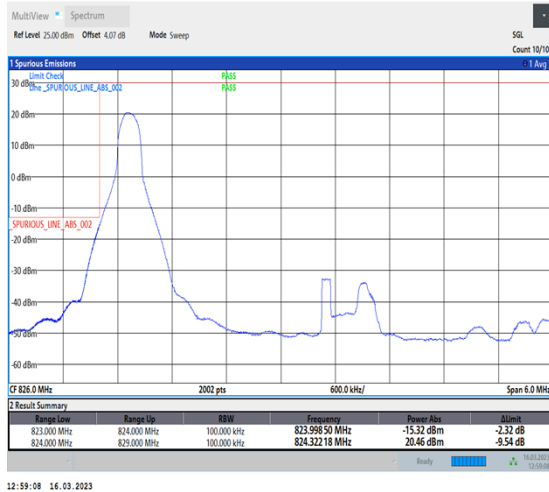
1-N26-824-849-PC3-15-5-L-1-DFT-PI2BPSK-Edge_1RB_Left-1@0-Ant1-1-seegraph-PASS-see graph
