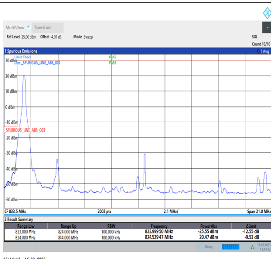
1-N26-824-849-PC3-15-20-L-1-DFT-PI2BPSK-Edge_1RB_Left-1@0-Ant1-1-seegraph-PASS-see graph
