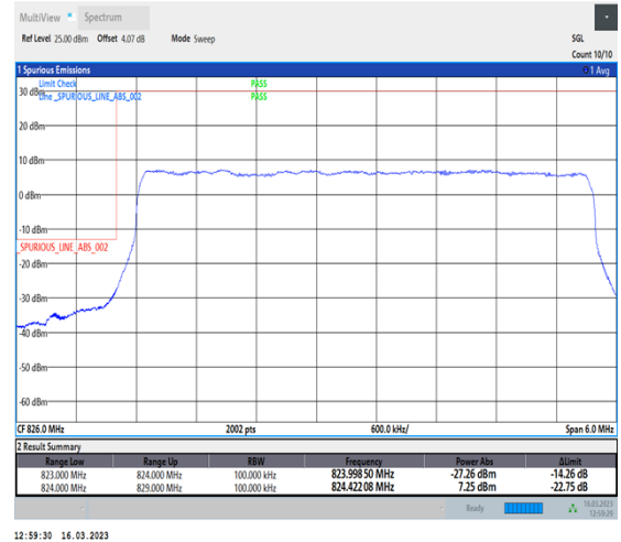
1-N26-824-849-PC3-15-5-L-3-DFT-PI2BPSK-Outer_Full-25@0-Ant1-1-seegraph-PASS-see graph
