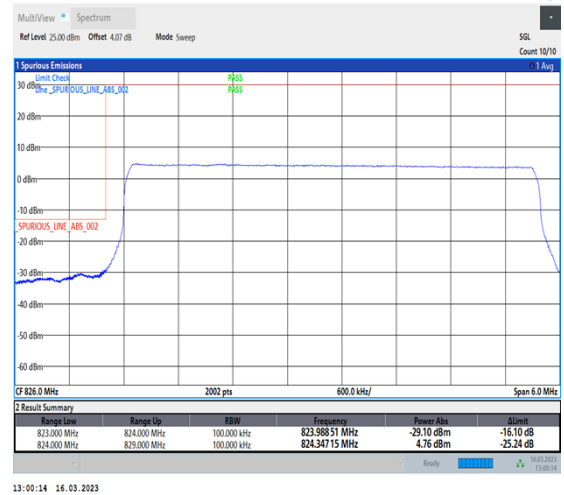
1-N26-824-849-PC3-15-5-L-6-CP-QPSK-Outer_Full-25@0-Ant1-1-seegraph-PASS-see graph
