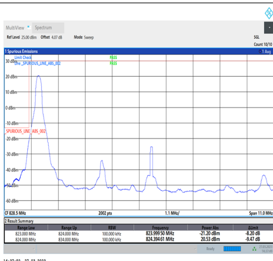
1-N26-824-849-PC3-15-10-L-1-DFT-PI2BPSK-Edge_1RB_Left-1@0-Ant1-1-seegraph-PASS-see graph
