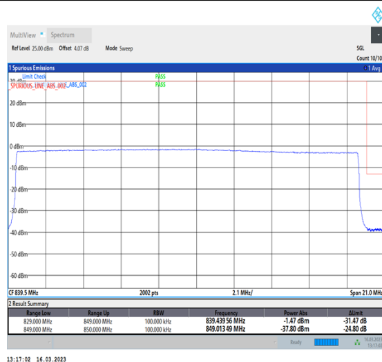
1-N26-824-849-PC3-15-20-H-6-CP-QPSK-Outer_Full-106@0-Ant1-1-seegraph-PASS-see graph
