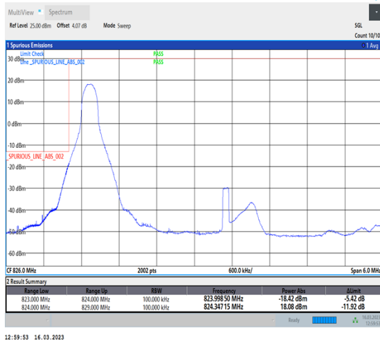
1-N26-824-849-PC3-15-5-L-4-CP-QPSK-Edge_1RB_Left-1@0-Ant1-1-seegraph-PASS-see graph
