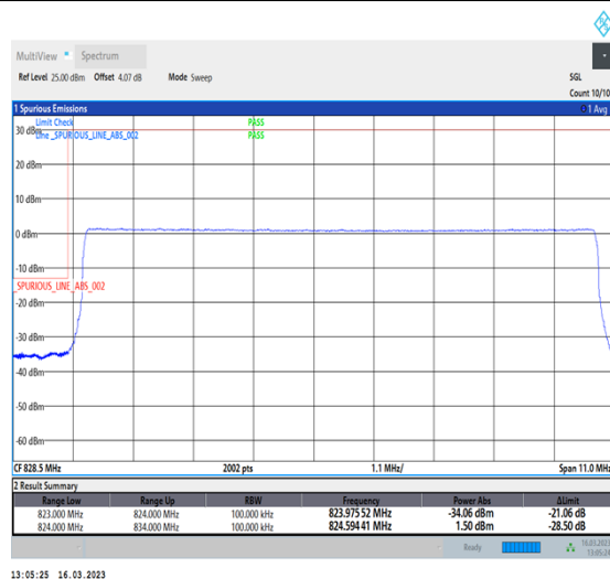
1-N26-824-849-PC3-15-10-L-6-CP-QPSK-Outer_Full-52@0-Ant1-1-seegraph-PASS-see graph
