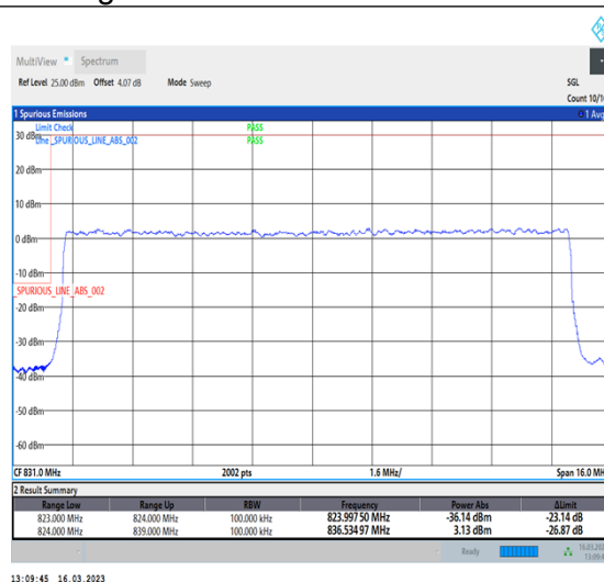
1-N26-824-849-PC3-15-15-L-3-DFT-PI2BPSK-Outer_Full-75@0-Ant1-1-seegraph-PASS-see graph
