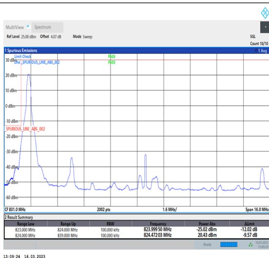
1-N26-824-849-PC3-15-15-L-1-DFT-PI2BPSK-Edge_1RB_Left-1@0-Ant1-1-seegraph-PASS-see graph
