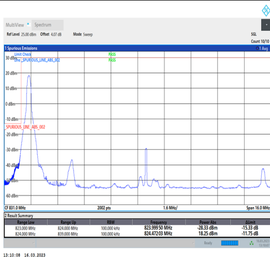
1-N26-824-849-PC3-15-15-L-4-CP-QPSK-Edge_1RB_Left-1@0-Ant1-1-seegraph-PASS-see graph
