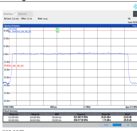
1-N26-824-849-PC3-15-20-L-3-DFT-PI2BPSK-Outer_Full-100@0-Ant1-1-seegraph-PASS-see graph
