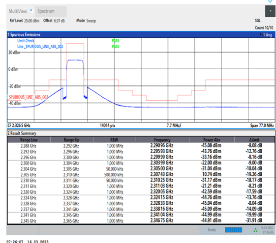
1-N30-PC3-15-5-L-6-CP-QPSK-Outer_Full-25@0-Ant1-1--PASS-see graph
