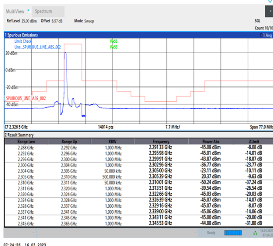
1-N30-PC3-15-5-L-4-CP-QPSK-Edge_1RB_Left-1@0-Ant1-1--PASS-see graph
