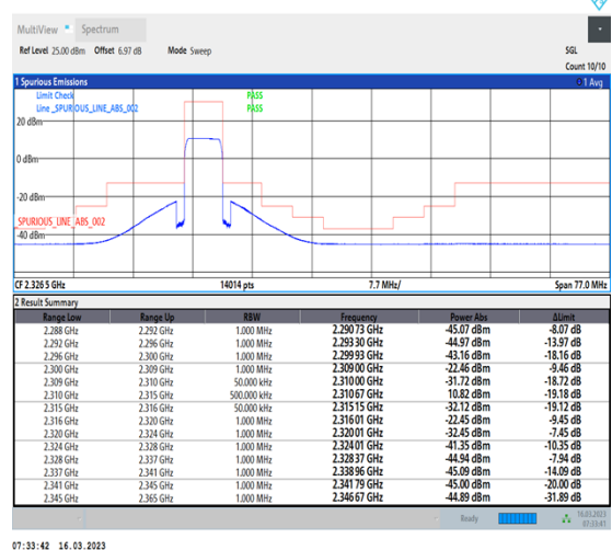
1-N30-PC3-15-5-H-6-CP-QPSK-Outer_Full-25@0-Ant1-1--PASS-see graph
