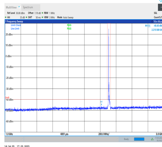
1-N30-PC3-15-10-M-1-DFT-PI2BPSK- Inner_1RB_Left-1@1-1000-3000-Ant1-2938.00-- 45.43--40-PASS
