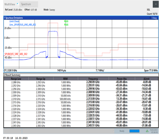
1-N30-PC3-15-5-H-3-DFT-PI2BPSK-Outer_Full-25@0-Ant1-1--PASS-see graph
