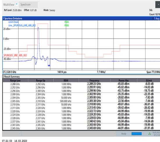
1-N30-PC3-15-5-L-1-DFT-PI2BPSK-Edge_1RB_Left-1@0-Ant1-1--PASS-see graph
