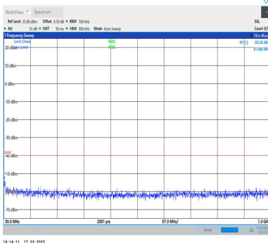
1-N30-PC3-15-10-M-1-DFT-PI2BPSK- Inner_1RB_Left-1@1-30-1000-Ant1-34.85--53.26-- 40-PASS
