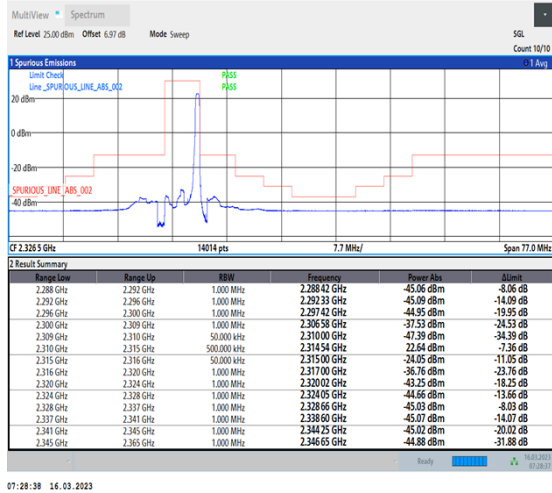
1-N30-PC3-15-5-H-2-DFT-PI2BPSK-Edge_1RB_Right-1@24-Ant1-1--PASS-see graph
