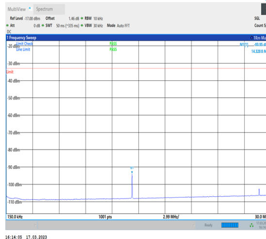
1-N30-PC3-15-10-M-1-DFT-PI2BPSK- Inner_1RB_Left-1@1-0.15-30-Ant1-13.97--93.95--33- PASS
