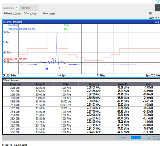
1-N30-PC3-15-5-H-5-CP-QPSK-Edge_1RB_Right-1@24-Ant1-1--PASS-see graph
