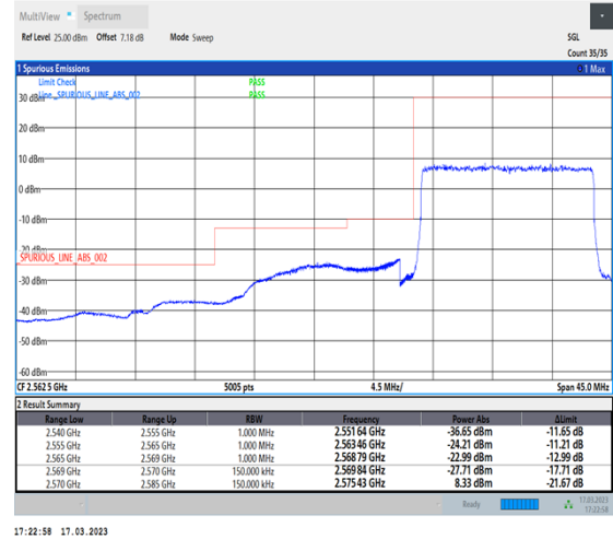
1-N38-30-15-L-3-DFT-PI2BPSK-Outer_Full-36@0-Ant1-1--PASS-see graph
