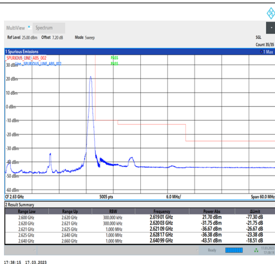
1-N38-30-20-H-2-DFT-PI2BPSK-Edge_1RB_Right-1@50-Ant1-1--PASS-see graph
