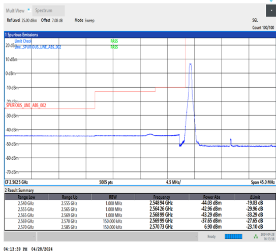
1-N38-30-15-L-1-DFT-PI2BPSK-Edge_1RB_Left-1@0-Ant1-1--PASS-see graph
