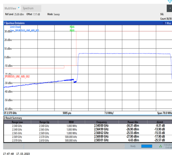
1-N38-30-40-L-6-CP-QPSK-Outer_Full-106@0-Ant1-1--PASS-see graph
