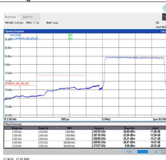
1-N38-30-20-L-3-DFT-PI2BPSK-Outer_Full-50@0-Ant1-1--PASS-see graph
