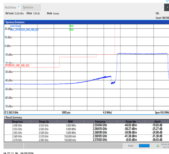
1-N38-30-15-L-6-CP-QPSK-Outer_Full-38@0-Ant1-1--PASS-see graph
