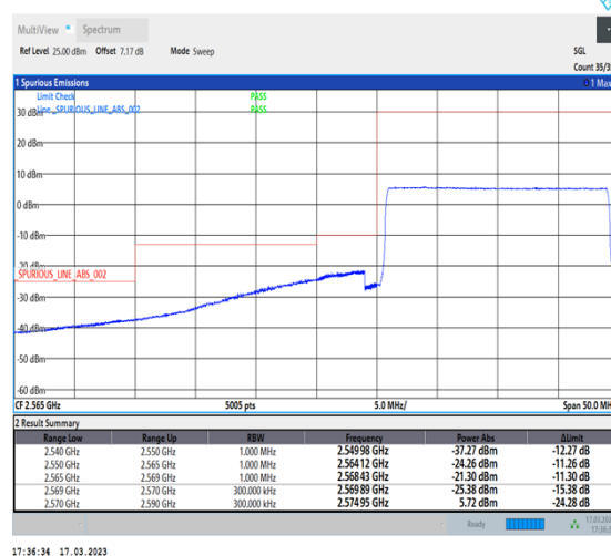
1-N38-30-20-L-6-CP-QPSK-Outer_Full-51@0-Ant1-1--PASS-see graph
