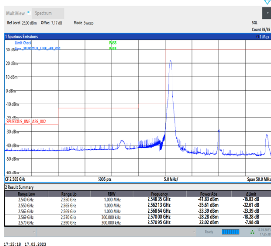
1-N38-30-20-L-4-CP-QPSK-Edge_1RB_Left-1@0-Ant1-1--PASS-see graph
