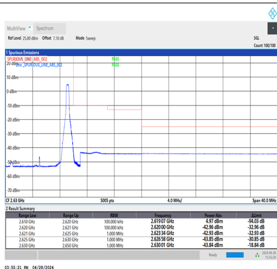
1-N38-30-10-H-2-DFT-PI2BPSK-Edge_1RB_Right-1@23-Ant1-1--PASS-see graph
