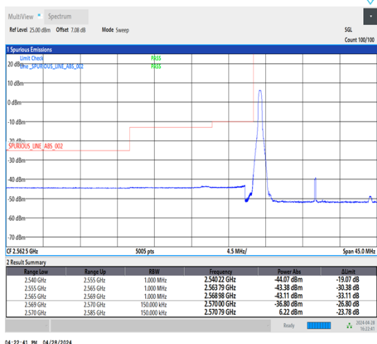
1-N38-30-15-L-4-CP-QPSK-Edge_1RB_Left-1@0-Ant1-1--PASS-see graph
