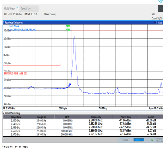
1-N38-30-40-L-1-DFT-PI2BPSK-Edge_1RB_Left-1@0-Ant1-1--PASS-see graph
