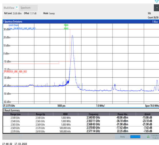
1-N38-30-40-L-4-CP-QPSK-Edge_1RB_Left-1@0-Ant1-1--PASS-see graph
