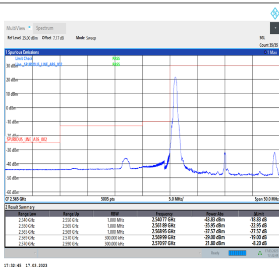
1-N38-30-20-L-1-DFT-PI2BPSK-Edge_1RB_Left-1@0-Ant1-1--PASS-see graph
