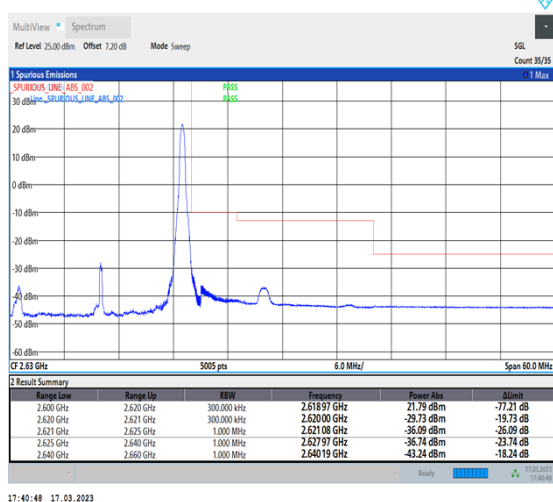
1-N38-30-20-H-5-CP-QPSK-Edge_1RB_Right-1@50-Ant1-1--PASS-see graph
