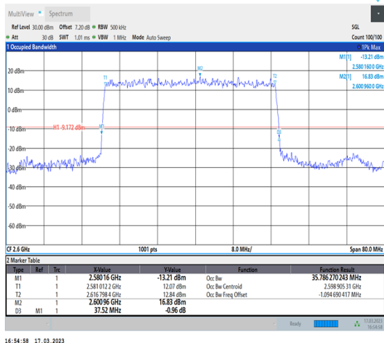
1-N38-30-40-H-2-DFT-PI2BPSK-Outer_Full-100@0-Ant1-35.786-37.520-≤40-PASS
