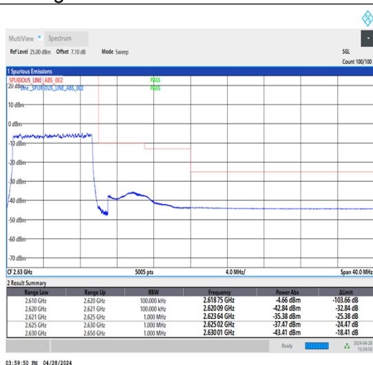
1-N38-30-10-H-3-DFT-PI2BPSK-Outer_Full-24@0-Ant1-1--PASS-see graph
