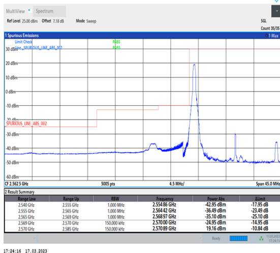
1-N38-30-15-L-4-CP-QPSK-Edge_1RB_Left-1@0-Ant1-1--PASS-see graph
