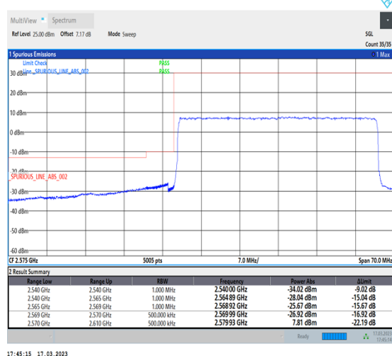
1-N38-30-40-L-3-DFT-PI2BPSK-Outer_Full-100@0-Ant1-1--PASS-see graph
