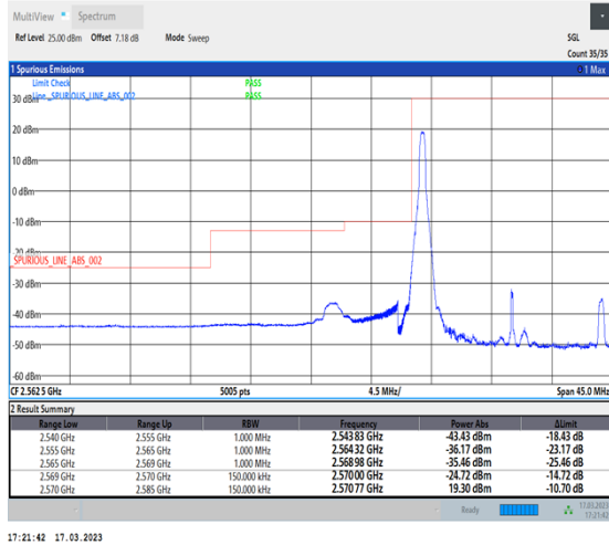
1-N38-30-15-L-1-DFT-PI2BPSK-Edge_1RB_Left-1@0-Ant1-1--PASS-see graph
