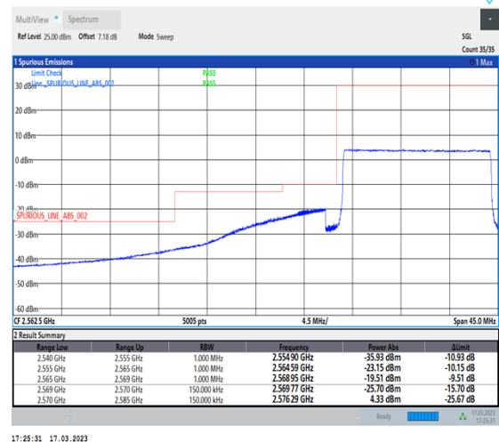
1-N38-30-15-L-6-CP-QPSK-Outer_Full-38@0-Ant1-1--PASS-see graph
