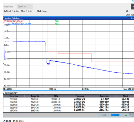
1-N38-30-20-H-6-CP-QPSK-Outer_Full-51@0-Ant1-1--PASS-see graph
