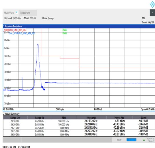
1-N38-30-10-H-5-CP-QPSK-Edge_1RB_Right-1@23-Ant1-1--PASS-see graph
