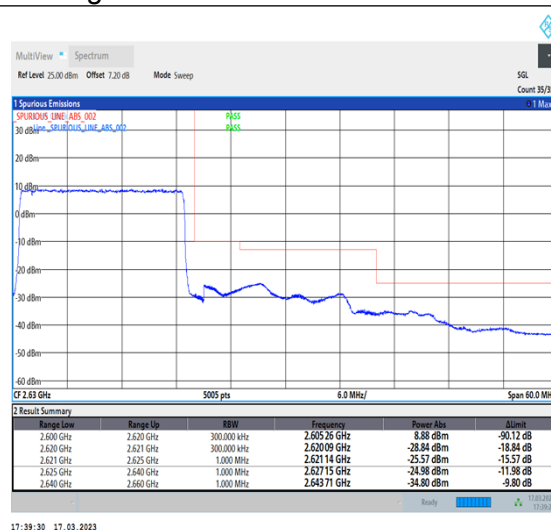
1-N38-30-20-H-3-DFT-PI2BPSK-Outer_Full-50@0-Ant1-1--PASS-see graph
