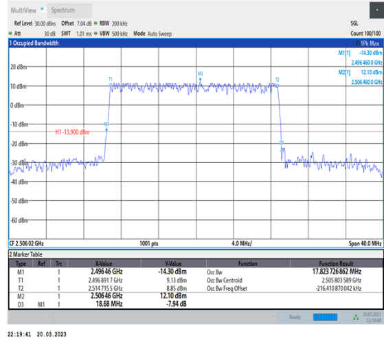
1-N41-30-20-L-4-DFT-64QAM-Outer_Full-50@0-Ant1-17.824-18.680-≤20-PASS
