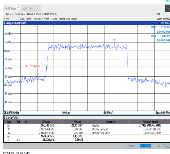
1-N41-30-30-H-9-CP-256QAM-Outer_Full-78@0- Ant1-27.829-28.920-≤30-PASS
