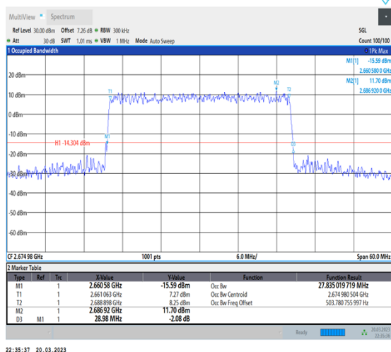
1-N41-30-30-H-6-CP-QPSK-Outer_Full-78@0-Ant1- 27.835-28.980-≤30-PASS
