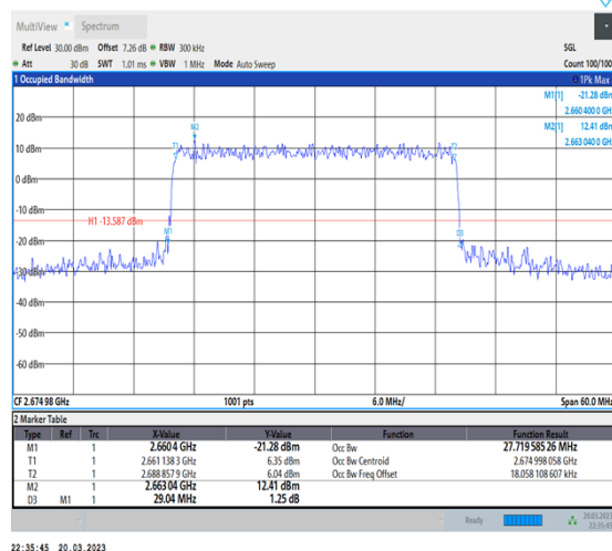
1-N41-30-30-H-7-CP-16QAM-Outer_Full-78@0- Ant1-27.72-29.040-≤30-PASS
