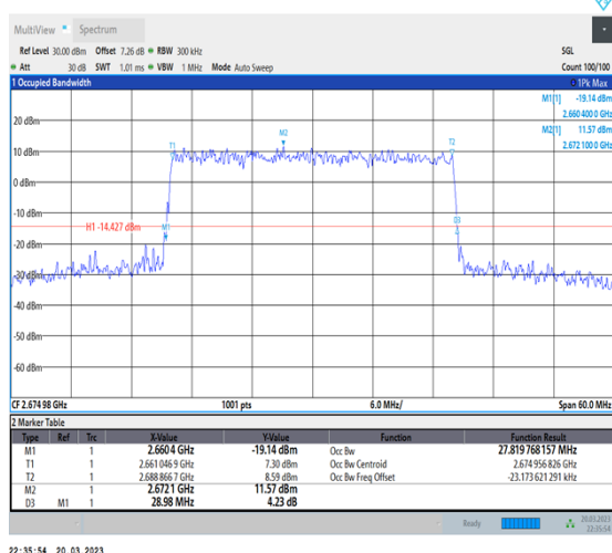
1-N41-30-30-H-8-CP-64QAM-Outer_Full-78@0- Ant1-27.82-28.980-≤30-PASS
