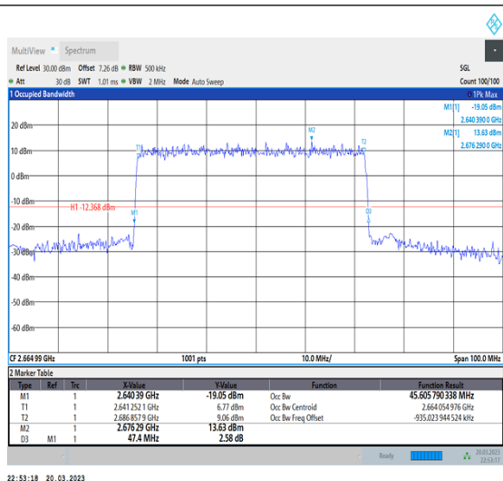
1-N41-30-50-H-4-DFT-64QAM-Outer_Full-128@0- Ant1-45.606-47.400-≤50-PASS
