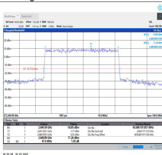
1-N41-30-50-H-5-DFT-256QAM-Outer_Full-128@0- Ant1-45.696-47.400-≤50-PASS
