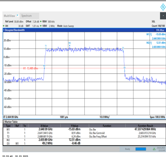
1-N41-30-50-H-6-CP-QPSK-Outer_Full-133@0- Ant1-47.337-49.200-≤50-PASS
