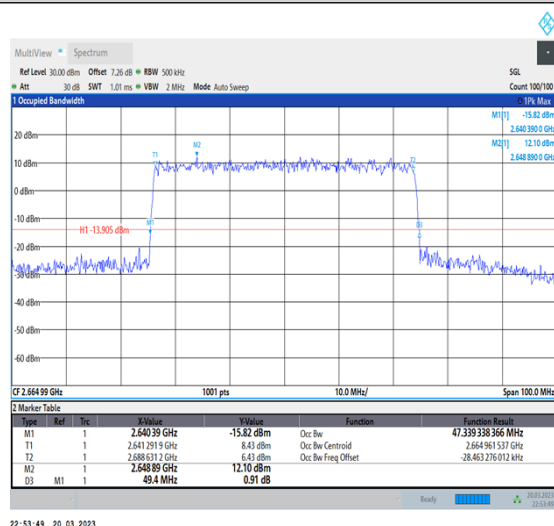
1-N41-30-50-H-7-CP-16QAM-Outer_Full-133@0- Ant1-47.339-49.400-≤50-PASS
