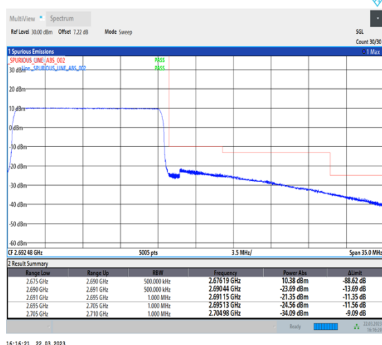
1-N41-30-15-H-6-CP-QPSK-Outer_Full-38@0-Ant1-1--PASS-see graph
