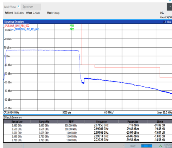
1-N41-30-30-H-6-CP-QPSK-Outer_Full-78@0-Ant1-1--PASS-see graph
