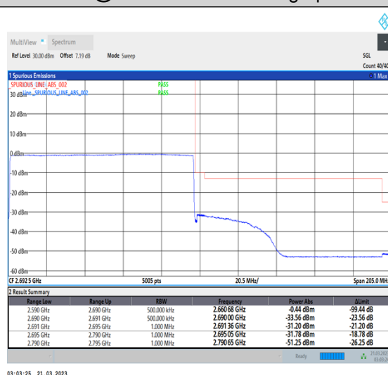
1-N41-30-100-H-6-CP-QPSK-Outer_Full-273@0-Ant1-1--PASS-see graph
