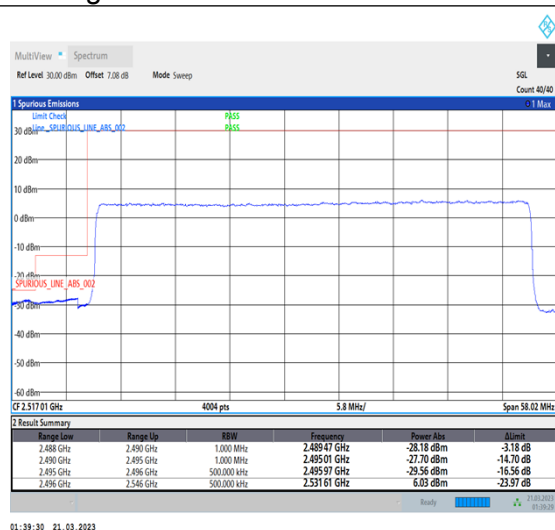
1-N41-30-50-L-3-DFT-PI2BPSK-Outer_Full-128@0-Ant1-1--PASS-see graph
