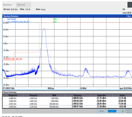
1-N41-30-20-L-4-CP-QPSK-Edge_1RB_Left-1@0-Ant1-1--PASS-see graph
