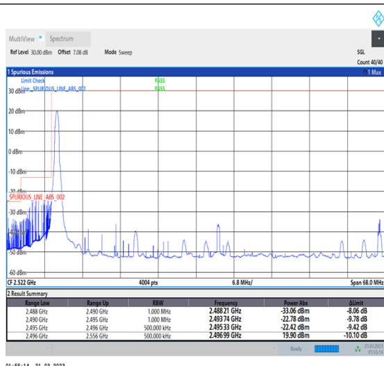
1-N41-30-60-L-1-DFT-PI2BPSK-Edge_1RB_Left-1@0-Ant1-1--PASS-see graph
