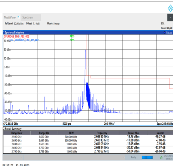
1-N41-30-100-H-2-DFT-PI2BPSK-Edge_1RB_Right-1@272-Ant1-1--PASS-see graph
