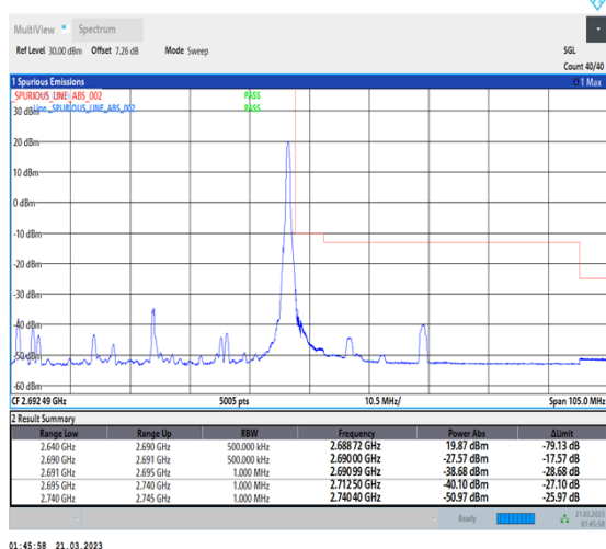
1-N41-30-50-H-2-DFT-PI2BPSK-Edge_1RB_Right-1@132-Ant1-1--PASS-see graph
