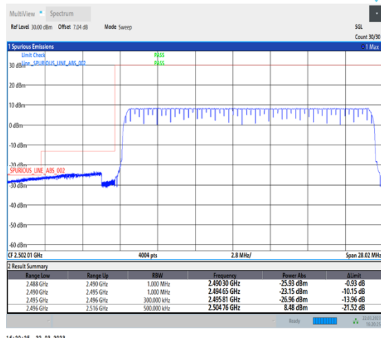
1-N41-30-20-L-6-CP-QPSK-Outer_Full-51@0-Ant1-1--PASS-see graph
