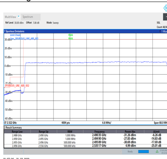
1-N41-30-60-L-3-DFT-PI2BPSK-Outer_Full-162@0-Ant1-1--PASS-see graph
