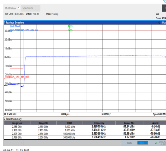
1-N41-30-60-L-6-CP-QPSK-Outer_Full-162@0-Ant1-1--PASS-see graph
