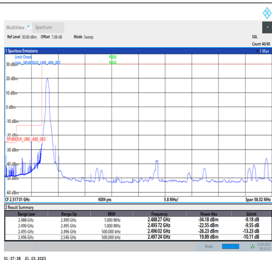
1-N41-30-50-L-1-DFT-PI2BPSK-Edge_1RB_Left-1@0-Ant1-1--PASS-see graph
