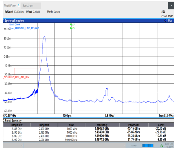
1-N41-30-30-L-4-CP-QPSK-Edge_1RB_Left-1@0-Ant1-1--PASS-see graph
