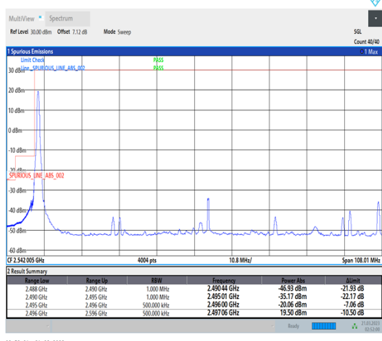
1-N41-30-100-L-4-CP-QPSK-Edge_1RB_Left-1@0-Ant1-1--PASS-see graph
