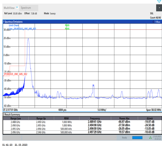
1-N41-30-50-L-4-CP-QPSK-Edge_1RB_Left-1@0-Ant1-1--PASS-see graph
