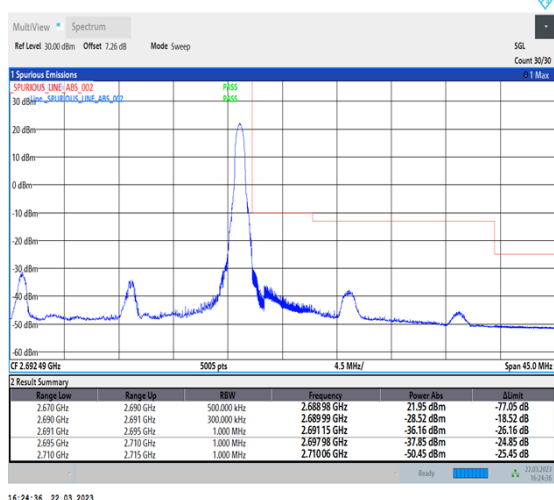
1-N41-30-20-H-5-CP-QPSK-Edge_1RB_Right-1@50-Ant1-1--PASS-see graph
