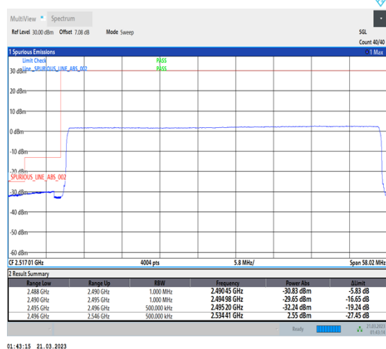
1-N41-30-50-L-6-CP-QPSK-Outer_Full-133@0-Ant1-1--PASS-see graph
