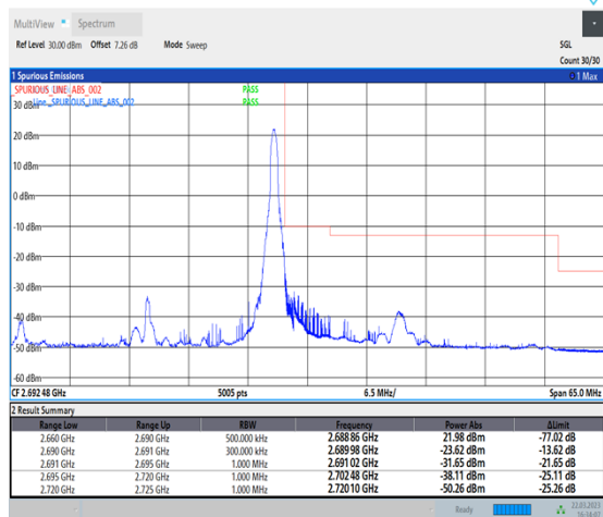
1-N41-30-30-H-5-CP-QPSK-Edge_1RB_Right-1@77-Ant1-1--PASS-see graph
