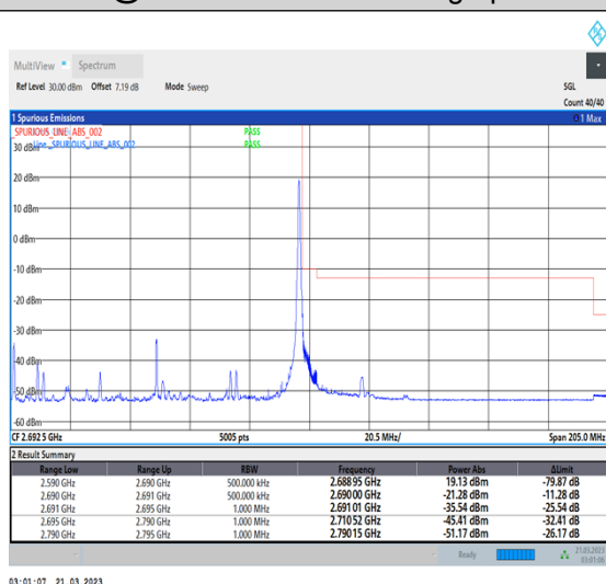
1-N41-30-100-H-5-CP-QPSK-Edge_1RB_Right-1@272-Ant1-1--PASS-see graph
