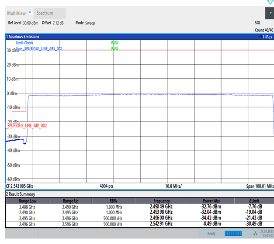
1-N41-30-100-L-6-CP-QPSK-Outer_Full-273@0-Ant1-1--PASS-see graph
