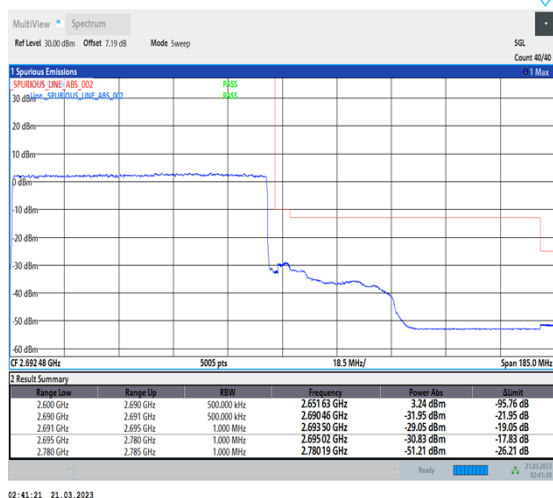
1-N41-30-90-H-3-DFT-PI2BPSK-Outer_Full-240@0-Ant1-1--PASS-see graph
