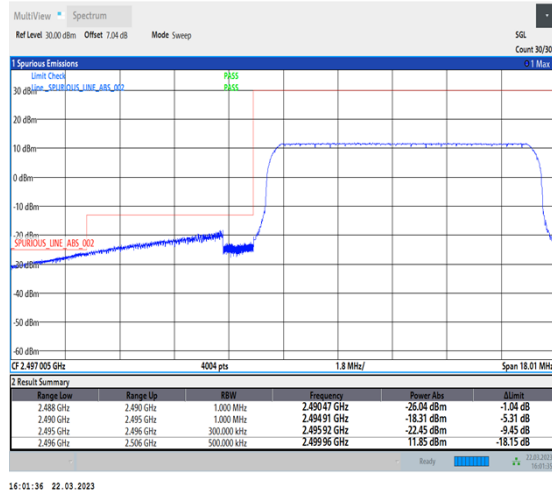
1-N41-30-10-L-6-CP-QPSK-Outer_Full-24@0-Ant1-1--PASS-see graph
