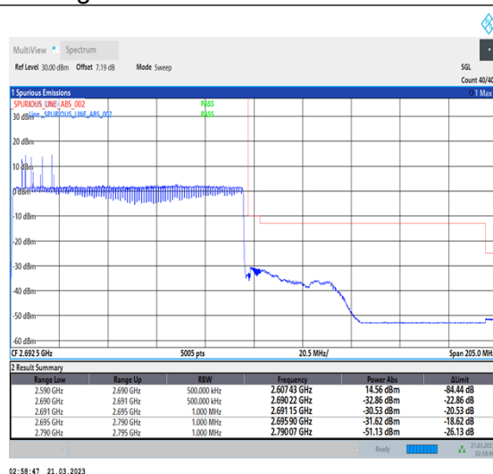
1-N41-30-100-H-3-DFT-PI2BPSK-Outer_Full-270@0-Ant1-1--PASS-see graph
