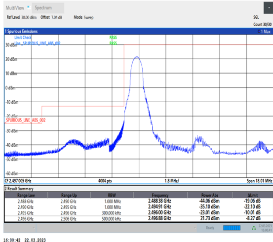
1-N41-30-10-L-4-CP-QPSK-Edge_1RB_Left-1@0-Ant1-1--PASS-see graph
