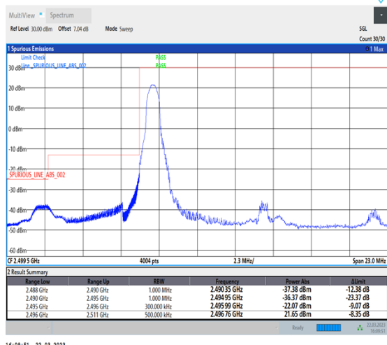
1-N41-30-15-L-4-CP-QPSK-Edge_1RB_Left-1@0-Ant1-1--PASS-see graph
