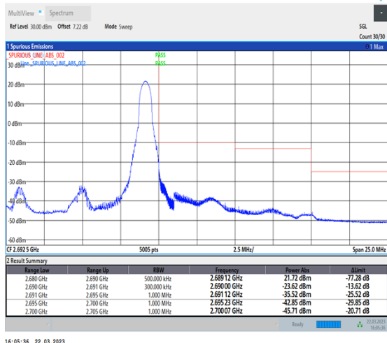
1-N41-30-10-H-5-CP-QPSK-Edge_1RB_Right-1@23-Ant1-1--PASS-see graph
