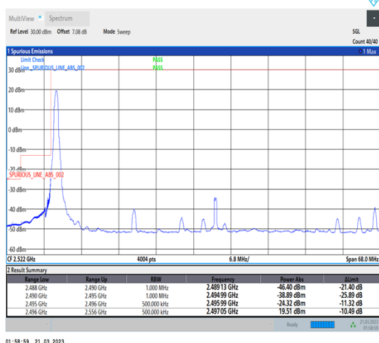
1-N41-30-60-L-4-CP-QPSK-Edge_1RB_Left-1@0-Ant1-1--PASS-see graph
