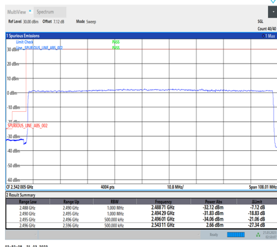
1-N41-30-100-L-3-DFT-PI2BPSK-Outer_Full-270@0-Ant1-1--PASS-see graph
