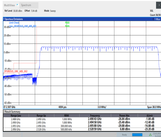
1-N41-30-30-L-6-CP-QPSK-Outer_Full-78@0-Ant1-1--PASS-see graph
