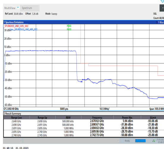
1-N41-30-50-H-3-DFT-PI2BPSK-Outer_Full-128@0-Ant1-1--PASS-see graph
