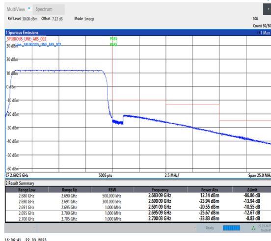
1-N41-30-10-H-6-CP-QPSK-Outer_Full-24@0-Ant1-1--PASS-see graph
