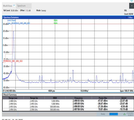
1-N41-30-100-L-1-DFT-PI2BPSK-Edge_1RB_Left-1@0-Ant1-1--PASS-see graph
