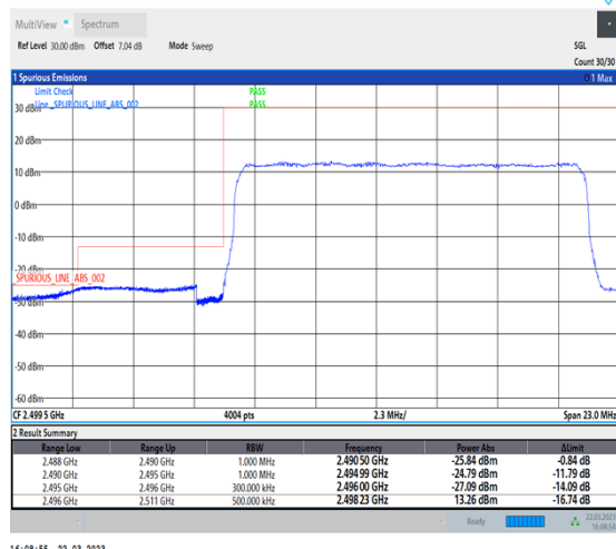
1-N41-30-15-L-6-CP-QPSK-Outer_Full-38@0-Ant1-1--PASS-see graph
