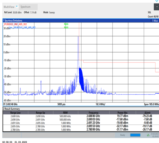
1-N41-30-90-H-2-DFT-PI2BPSK-Edge_1RB_Right-1@244-Ant1-1--PASS-see graph
