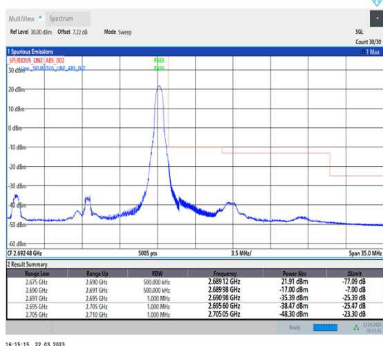
1-N41-30-15-H-5-CP-QPSK-Edge_1RB_Right-1@37-Ant1-1--PASS-see graph
