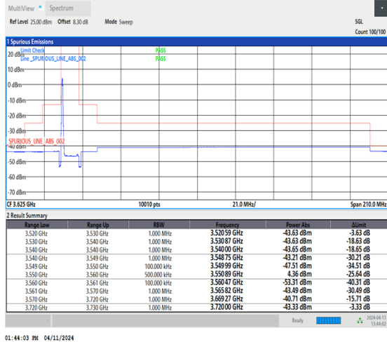
1-N48-30-10-L-1-DFT-PI2BPSK-Edge_1RB_Left-1@0-Ant0-1--PASS-see graph
