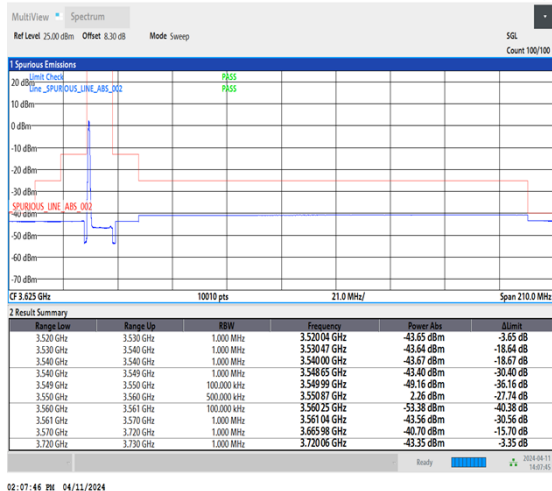
1-N48-30-10-L-4-CP-QPSK-Edge_1RB_Left-1@0-Ant0-1--PASS-see graph
