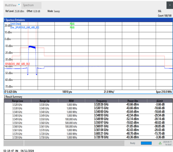
1-N48-30-10-L-6-CP-QPSK-Outer_Full-24@0-Ant0-1--PASS-see graph
