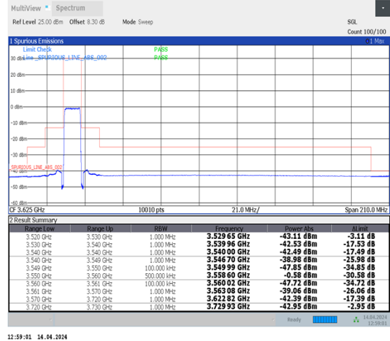
1-N48-30-10-L-3-DFT-PI2BPSK-Outer_Full-24@0-Ant0-1--PASS-see graph
