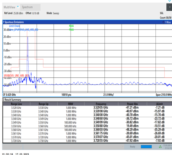
1-N48-PC3-30-10-L-4-CP-QPSK-Edge_1RB_Left-1@0-Ant0-1--PASS-see graph
