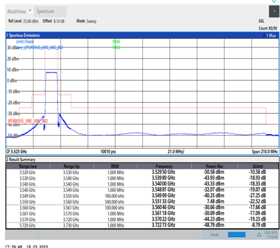
1-N48-PC3-30-10-L-6-CP-QPSK-Outer_Full-24@0-Ant0-1--PASS-see graph
