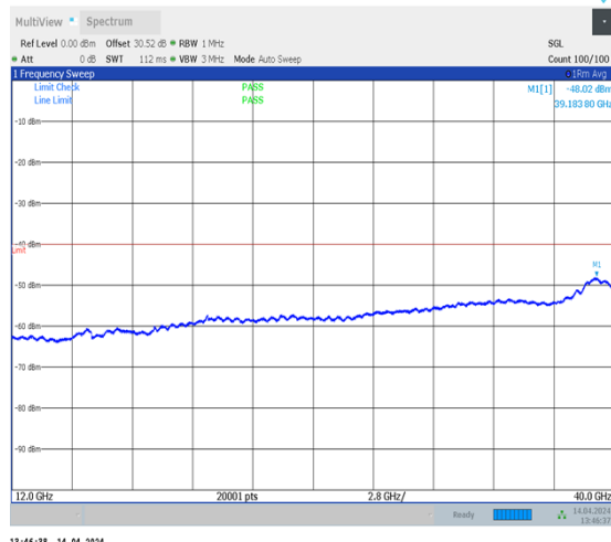
1-N48-PC3-30-40-H-1-DFT-PI2BPSK-Inner_1RB_Left- 1@1-12000-40000-Ant0-12000.00--48.00--40-PASS
