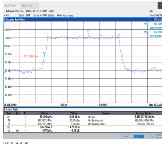
1-N5-PC3-15-5-L-2-DFT-PI2BPSK-Outer_Full- 25@0-Ant1-4.48-4.870-≤5-PASS
