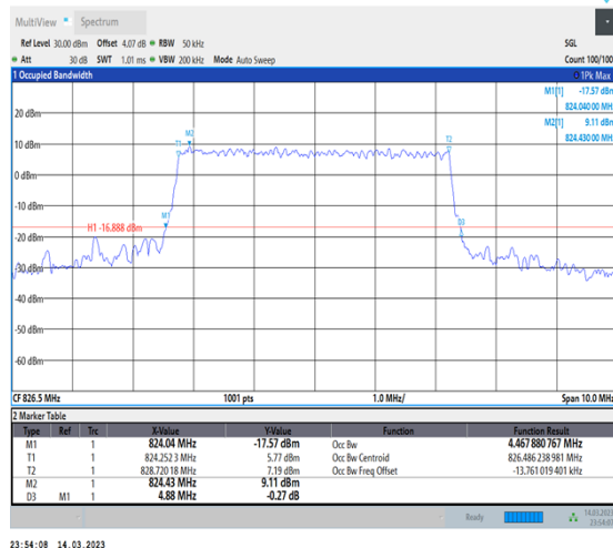
1-N5-PC3-15-5-L-6-CP-QPSK-Outer_Full-25@0- Ant1-4.468-4.880-≤5-PASS
