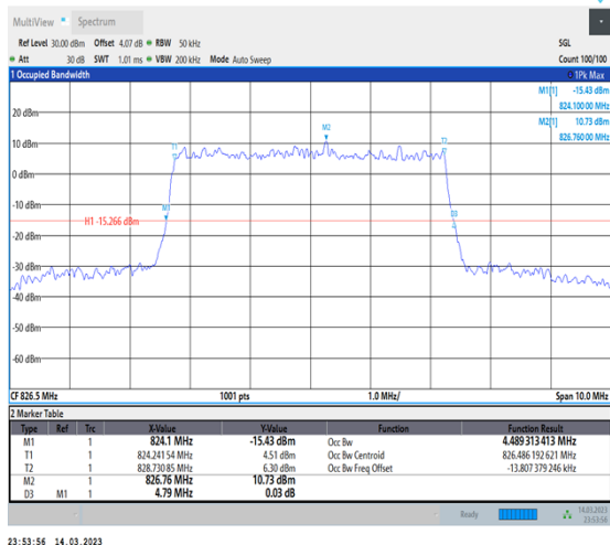
1-N5-PC3-15-5-L-5-DFT-256QAM-Outer_Full-25@0- Ant1-4.489-4.790-≤5-PASS
