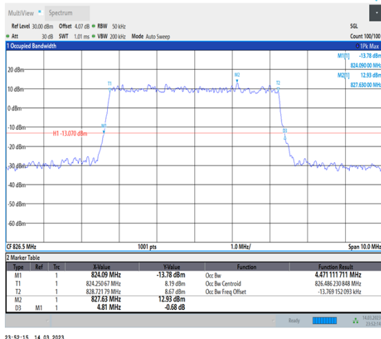
1-N5-PC3-15-5-L-1-DFT-QPSK-Outer_Full-25@0- Ant1-4.471-4.810-≤5-PASS
