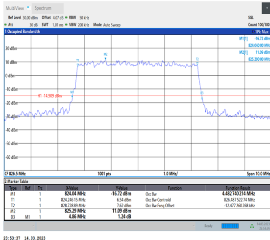
1-N5-PC3-15-5-L-3-DFT-16QAM-Outer_Full-25@0- Ant1-4.483-4.860-≤5-PASS
