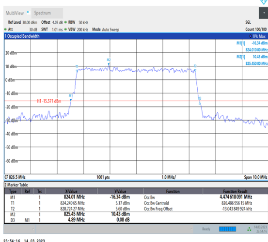
1-N5-PC3-15-5-L-7-CP-16QAM-Outer_Full-25@0- Ant1-4.475-4.890-≤5-PASS
