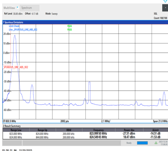
1-N515-20-L-4-CP-QPSK-Edge_1RB_Left-1@0-Ant1-1-seegraph-PASS-see graph
