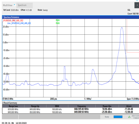
1-N515-10-H-2-DFT-PI2BPSK-Edge_1RB_Right-1@51-Ant1-1-seegraph-PASS-see graph
