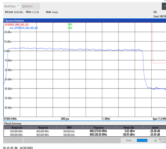
1-N515-10-H-3-DFT-PI2BPSK-Outer_Full-50@0-Ant1-1-seegraph-PASS-see graph
