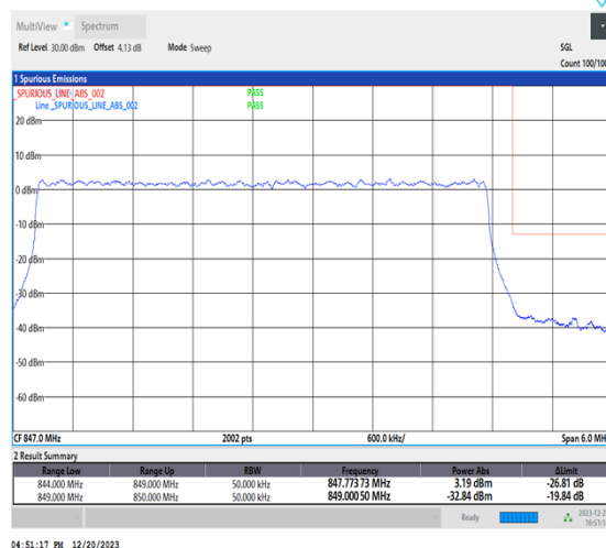
1-N515-5-H-3-DFT-PI2BPSK-Outer_Full-25@0-Ant1-1-seegraph-PASS-see graph
