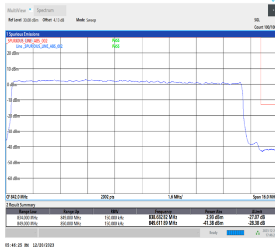
1-N515-15-H-3-DFT-PI2BPSK-Outer_Full-75@0-Ant1-1-seegraph-PASS-see graph
