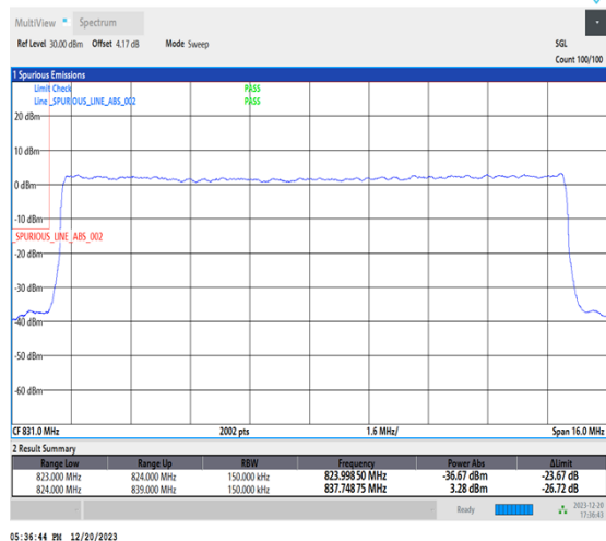
1-N515-15-L-3-DFT-PI2BPSK-Outer_Full-75@0-Ant1-1-seegraph-PASS-see graph
