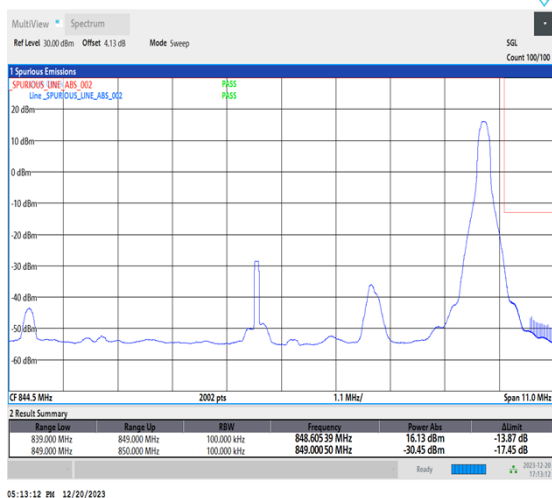
1-N515-10-H-5-CP-QPSK-Edge_1RB_Right-1@51-Ant1-1-seegraph-PASS-see graph
