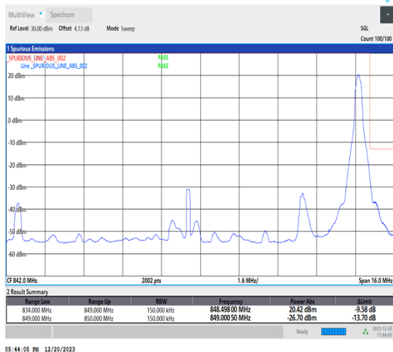
1-N515-15-H-2-DFT-PI2BPSK-Edge_1RB_Right-1@78-Ant1-1-seegraph-PASS-see graph
