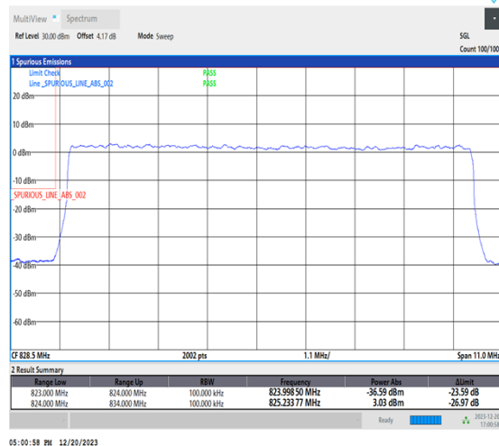
1-N515-10-L-3-DFT-PI2BPSK-Outer_Full-50@0-Ant1-1-seegraph-PASS-see graph
