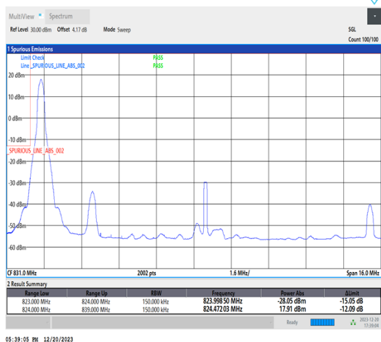
1-N515-15-L-4-CP-QPSK-Edge_1RB_Left-1@0-Ant1-1-seegraph-PASS-see graph
