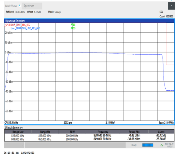
1-N515-20-H-6-CP-QPSK-Outer_Full-106@0-Ant1-1-seegraph-PASS-see graph
