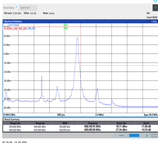
1-N5-PC3-15-10-H-5-CP-QPSK-Edge_1RB_Right-1@51-Ant1-1-seegraph-PASS-see graph
