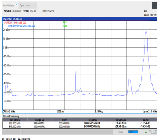
1-N515-20-H-5-CP-QPSK-Edge_1RB_Right-1@105-Ant1-1-seegraph-PASS-see graph
