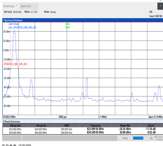
1-N515-20-L-1-DFT-PI2BPSK-Edge_1RB_Left-1@0-Ant1-1-seegraph-PASS-see graph
