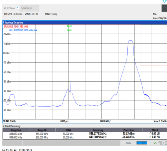
1-N515-5-H-5-CP-QPSK-Edge_1RB_Right-1@24-Ant1-1-seegraph-PASS-see graph
