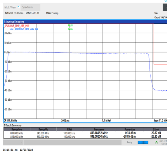
1-N515-10-H-6-CP-QPSK-Outer_Full-52@0-Ant1-1-seegraph-PASS-see graph
