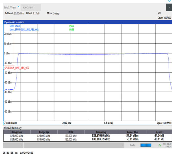
1-N515-15-L-6-CP-QPSK-Outer_Full-79@0-Ant1-1-seegraph-PASS-see graph
