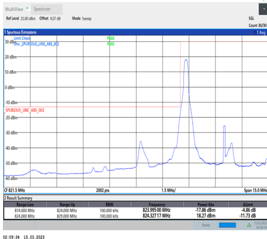
1-N5-PC3-15-5-L-4-CP-QPSK-Edge_1RB_Left-1@0-Ant1-1-seegraph-PASS-see graph
