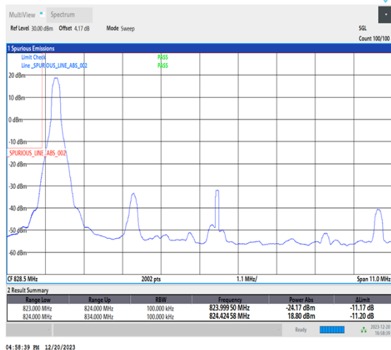
1-N515-10-L-1-DFT-PI2BPSK-Edge_1RB_Left-1@0-Ant1-1-seegraph-PASS-see graph
