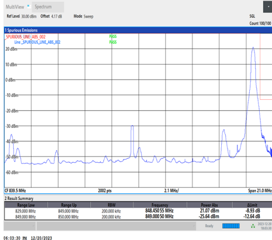
1-N515-20-H-2-DFT-PI2BPSK-Edge_1RB_Right-1@105-Ant1-1-seegraph-PASS-see graph
