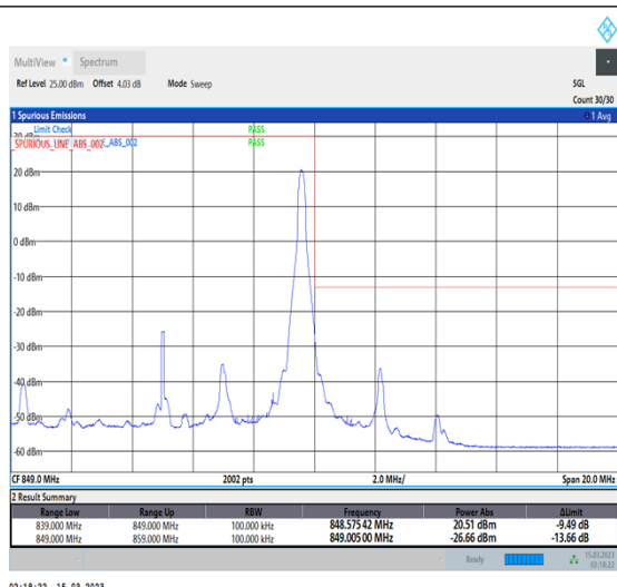
1-N5-PC3-15-10-H-2-DFT-PI2BPSK-Edge_1RB_Right-1@51-Ant1-1-seegraph-PASS-see graph
