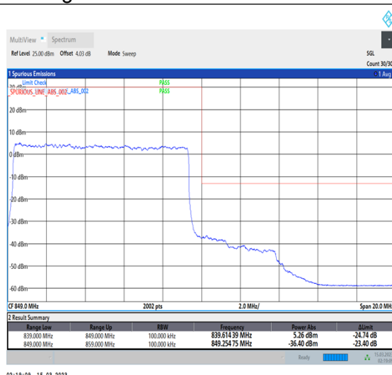
1-N5-PC3-15-10-H-3-DFT-PI2BPSK-Outer_Full-50@0-Ant1-1-seegraph-PASS-see graph
