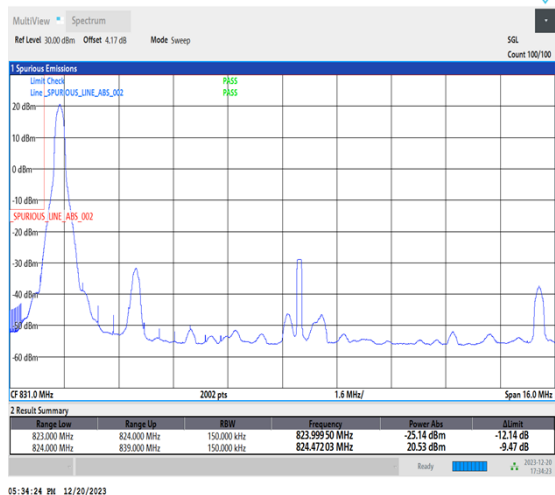
1-N515-15-L-1-DFT-PI2BPSK-Edge_1RB_Left-1@0-Ant1-1-seegraph-PASS-see graph
