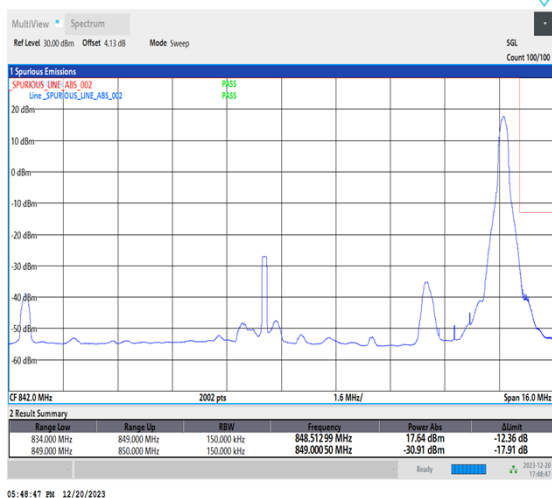
1-N515-15-H-5-CP-QPSK-Edge_1RB_Right-1@78-Ant1-1-seegraph-PASS-see graph
