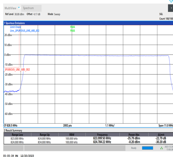
1-N515-10-L-6-CP-QPSK-Outer_Full-52@0-Ant1-1-seegraph-PASS-see graph
