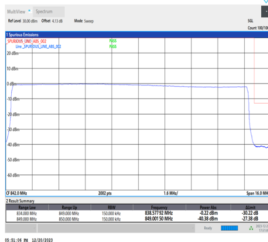
1-N515-15-H-6-CP-QPSK-Outer_Full-79@0-Ant1-1-seegraph-PASS-see graph
