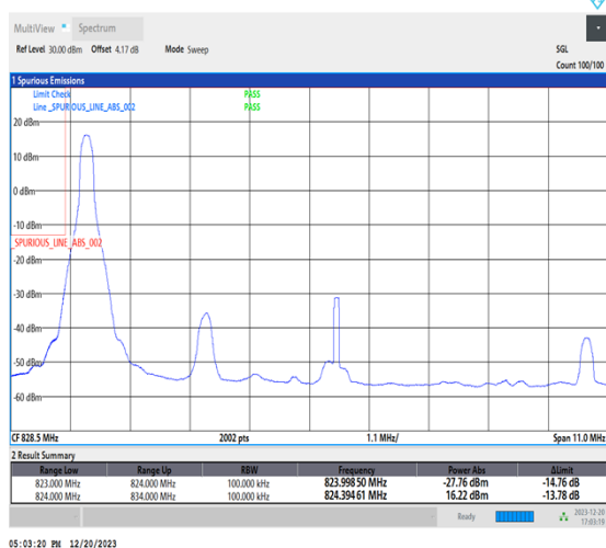
1-N515-10-L-4-CP-QPSK-Edge_1RB_Left-1@0-Ant1-1-seegraph-PASS-see graph
