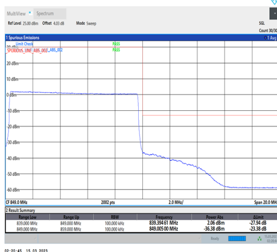
1-N5-PC3-15-10-H-6-CP-QPSK-Outer_Full-52@0-Ant1-1-seegraph-PASS-see graph
