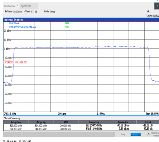
1-N515-20-L-3-DFT-PI2BPSK-Outer_Full-100@0-Ant1-1-seegraph-PASS-see graph
