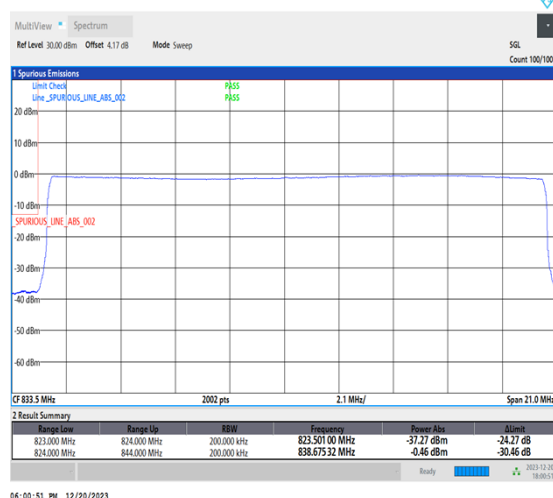
1-N515-20-L-6-CP-QPSK-Outer_Full-106@0-Ant1-1-seegraph-PASS-see graph
