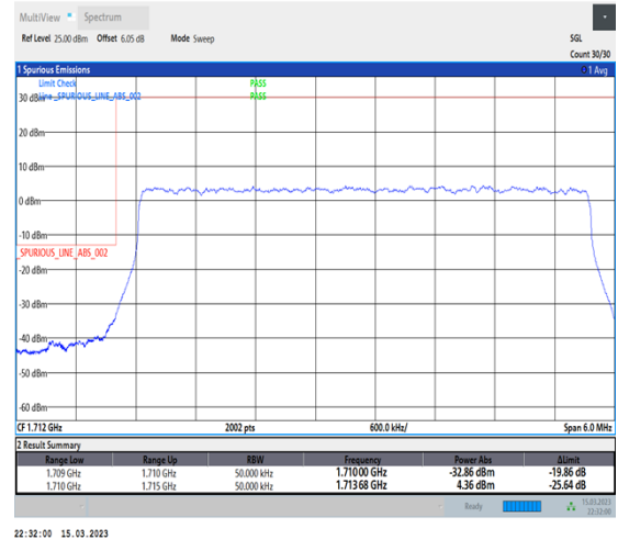
1-N66-PC3-15-5-L-3-DFT-PI2BPSK-Outer_Full-25@0-Ant1-1-seegraph-PASS-see graph
