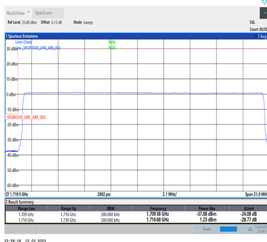
1-N66-PC3-15-20-L-6-CP-QPSK-Outer_Full-106@0-Ant1-1-seegraph-PASS-see graph
