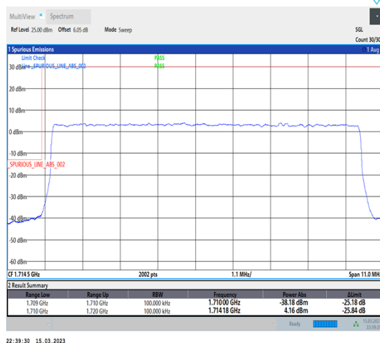
1-N66-PC3-15-10-L-3-DFT-PI2BPSK-Outer_Full-50@0-Ant1-1-seegraph-PASS-see graph
