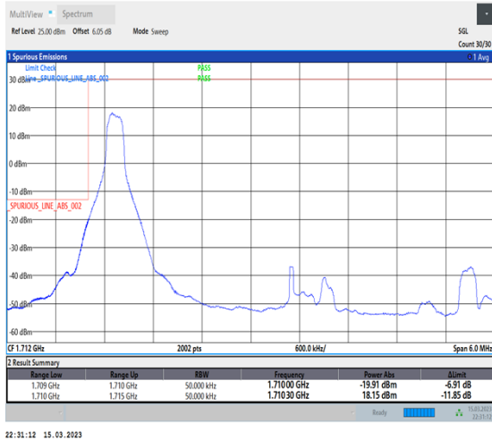
1-N66-PC3-15-5-L-1-DFT-PI2BPSK-Edge_1RB_Left-1@0-Ant1-1-seegraph-PASS-see graph
