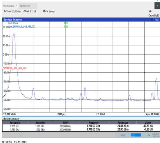
1-N66-PC3-15-20-L-1-DFT-PI2BPSK-Edge_1RB_Left-1@0-Ant1-1-seegraph-PASS-see graph
