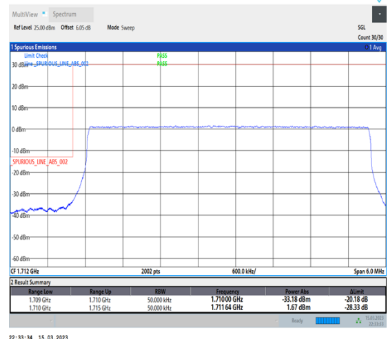
1-N66-PC3-15-5-L-6-CP-QPSK-Outer_Full-25@0-Ant1-1-seegraph-PASS-see graph
