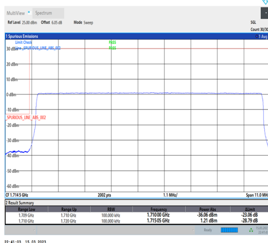
1-N66-PC3-15-10-L-6-CP-QPSK-Outer_Full-52@0-Ant1-1-seegraph-PASS-see graph
