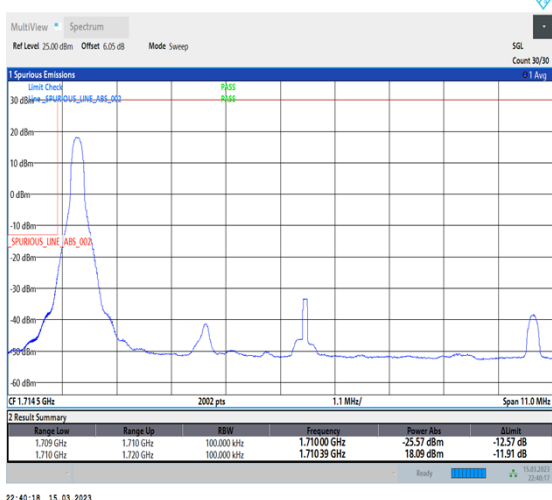
1-N66-PC3-15-10-L-4-CP-QPSK-Edge_1RB_Left-1@0-Ant1-1-seegraph-PASS-see graph
