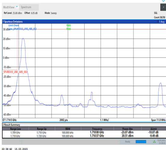
1-N66-PC3-15-10-L-1-DFT-PI2BPSK-Edge_1RB_Left-1@0-Ant1-1-seegraph-PASS-see graph
