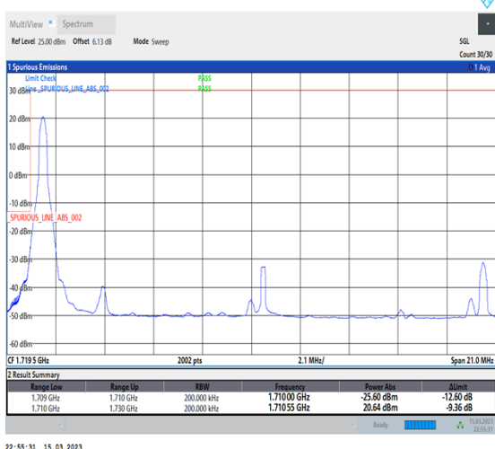
1-N66-PC3-15-20-L-4-CP-QPSK-Edge_1RB_Left-1@0-Ant1-1-seegraph-PASS-see graph
