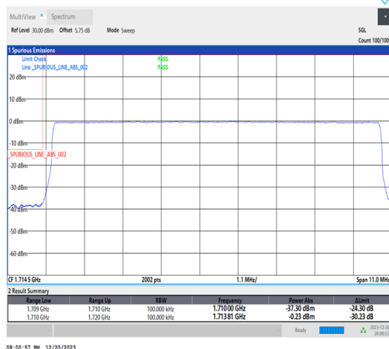
1-N66-15-10-L-6-CP-QPSK-Outer_Full-52@0-Ant1-1-seegraph-PASS-see graph
