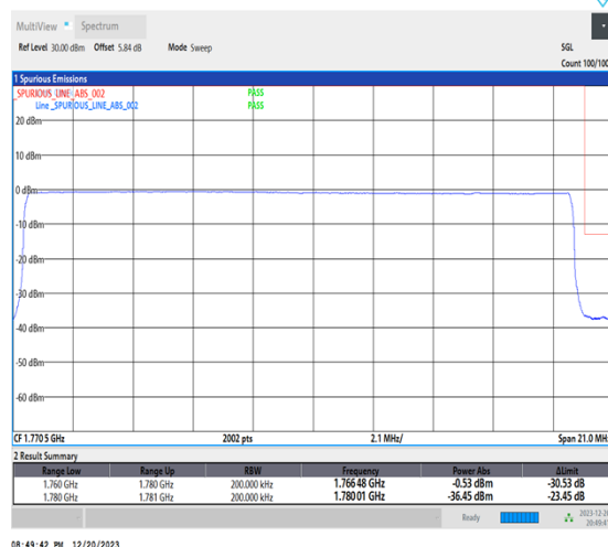
1-N66-15-20-H-6-CP-QPSK-Outer_Full-106@0-Ant1-1-seegraph-PASS-see graph
