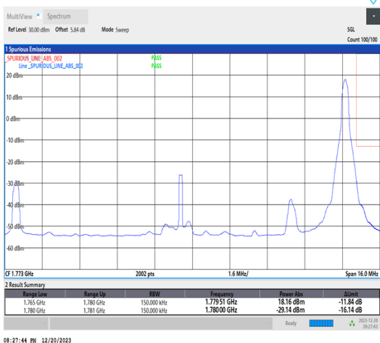
1-N66-15-15-H-5-CP-QPSK-Edge_1RB_Right-1@78-Ant1-1-seegraph-PASS-see graph
