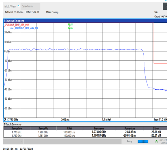
1-N66-15-10-H-3-DFT-PI2BPSK-Outer_Full-50@0-Ant1-1-seegraph-PASS-see graph
