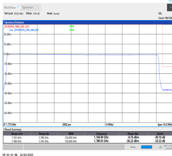
1-N66-15-15-H-6-CP-QPSK-Outer_Full-79@0-Ant1-1-seegraph-PASS-see graph
