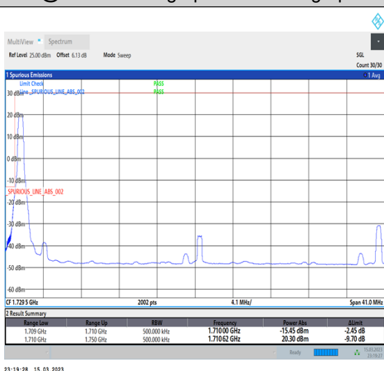
1-N66-PC3-15-40-L-4-CP-QPSK-Edge_1RB_Left-1@0-Ant1-1-seegraph-PASS-see graph
