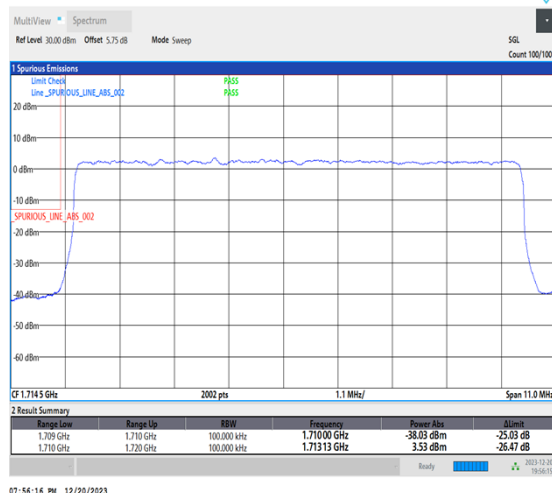
1-N66-15-10-L-3-DFT-PI2BPSK-Outer_Full-50@0-Ant1-1-seegraph-PASS-see graph
