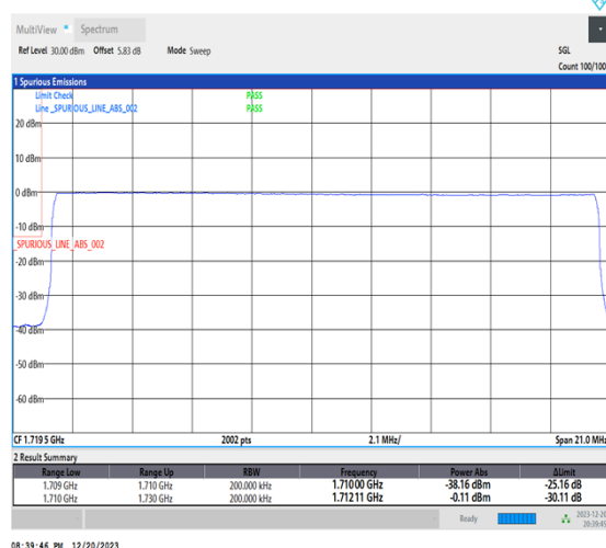
1-N66-15-20-L-6-CP-QPSK-Outer_Full-106@0-Ant1-1-seegraph-PASS-see graph
