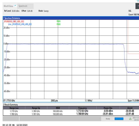
1-N66-15-10-H-6-CP-QPSK-Outer_Full-52@0-Ant1-1-seegraph-PASS-see graph
