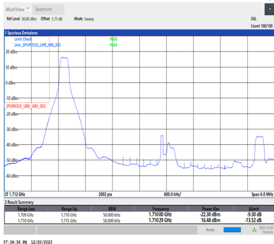
1-N66-15-5-L-1-DFT-PI2BPSK-Edge_1RB_Left-1@0-Ant1-1-seegraph-PASS-see graph
