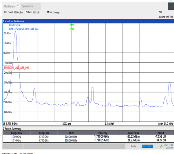
1-N66-15-20-L-1-DFT-PI2BPSK-Edge_1RB_Left-1@0-Ant1-1-seegraph-PASS-see graph
