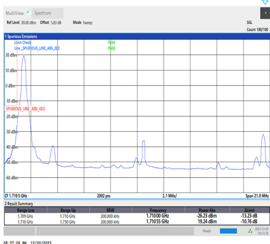
1-N66-15-20-L-4-CP-QPSK-Edge_1RB_Left-1@0-Ant1-1-seegraph-PASS-see graph
