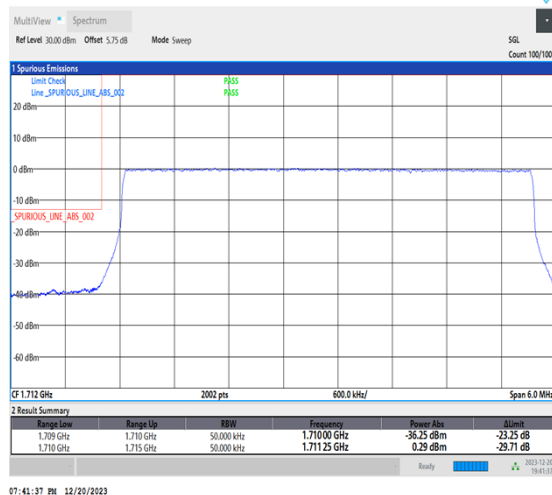
1-N66-15-5-L-6-CP-QPSK-Outer_Full-25@0-Ant1-1-seegraph-PASS-see graph
