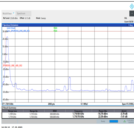
1-N66-PC3-15-40-L-1-DFT-PI2BPSK-Edge_1RB_Left-1@0-Ant1-1-seegraph-PASS-see graph
