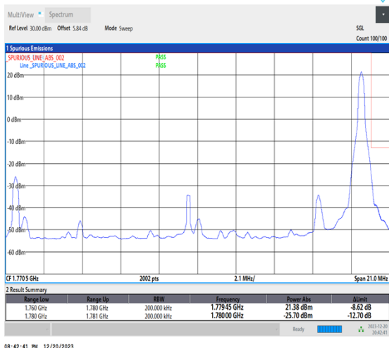
1-N66-15-20-H-2-DFT-PI2BPSK-Edge_1RB_Right-1@105-Ant1-1-seegraph-PASS-see graph
