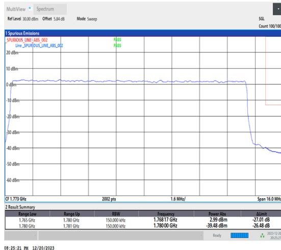
1-N66-15-15-H-3-DFT-PI2BPSK-Outer_Full-75@0-Ant1-1-seegraph-PASS-see graph
