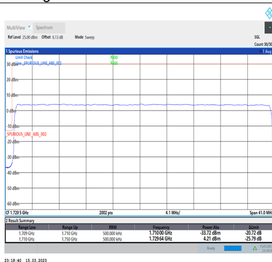
1-N66-PC3-15-40-L-3-DFT-PI2BPSK-Outer_Full-216@0-Ant1-1-seegraph-PASS-see graph
