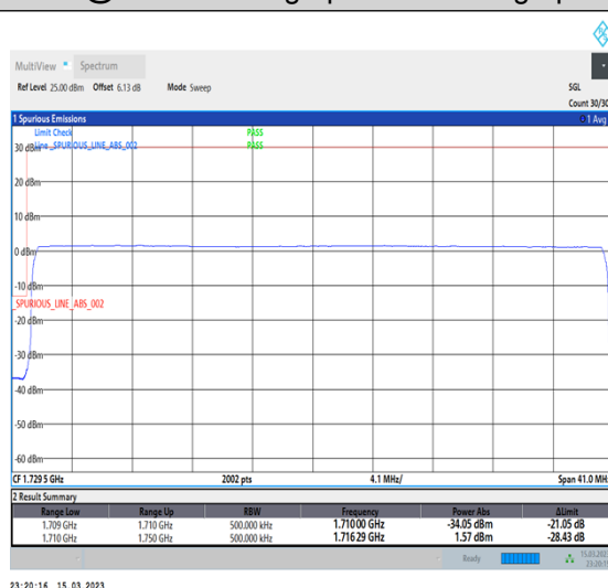
1-N66-PC3-15-40-L-6-CP-QPSK-Outer_Full-216@0-Ant1-1-seegraph-PASS-see graph
