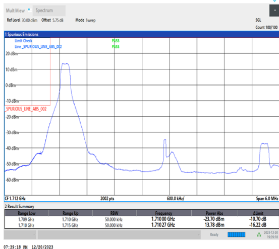
1-N66-15-5-L-4-CP-QPSK-Edge_1RB_Left-1@0-Ant1-1-seegraph-PASS-see graph
