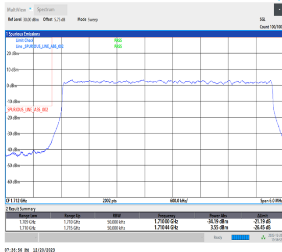
1-N66-15-5-L-3-DFT-PI2BPSK-Outer_Full-25@0-Ant1-1-seegraph-PASS-see graph
