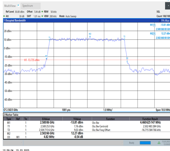
1-N7-PC3-15-5-L-2-DFT-PI2BPSK-Outer_Full- 25@0-Ant1-4.461-4.820-≤5-PASS
