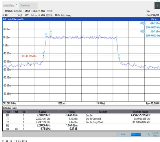
1-N7-PC3-15-5-L-1-DFT-QPSK-Outer_Full-25@0- Ant1-4.458-4.780-≤5-PASS
