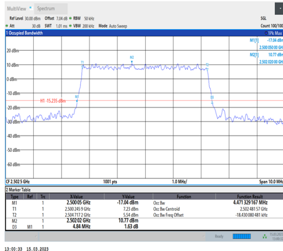
1-N7-PC3-15-5-L-4-DFT-64QAM-Outer_Full-25@0- Ant1-4.471-4.840-≤5-PASS
