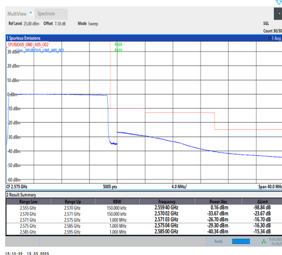
1-N7-PC3-15-15-H-6-CP-QPSK-Outer_Full-79@0-Ant1-1--PASS-see graph
