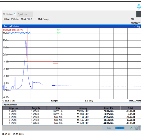
1-N7-PC3-15-5-H-2-DFT-PI2BPSK-Edge_1RB_Right-1@24-Ant1-1--PASS-see graph
