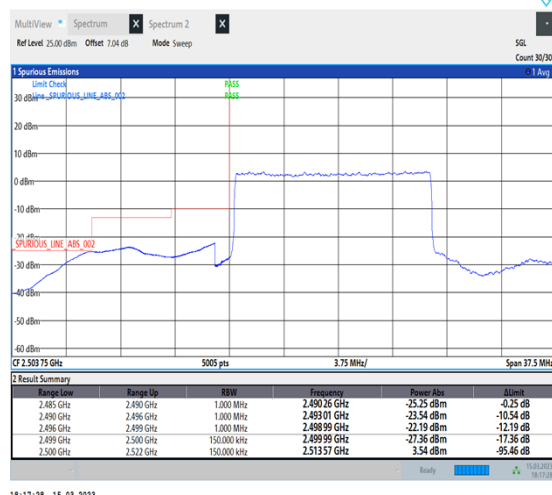
1-N7-PC3-15-15-L-3-DFT-PI2BPSK-Outer_Full-75@0-Ant1-1--PASS-see graph
