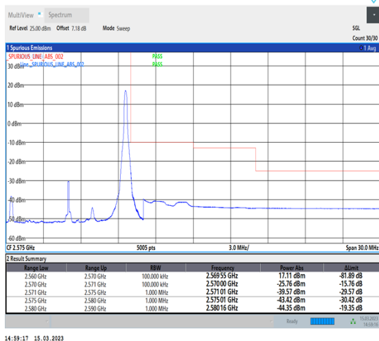
1-N7-PC3-15-10-H-5-CP-QPSK-Edge_1RB_Right-1@51-Ant1-1--PASS-see graph
