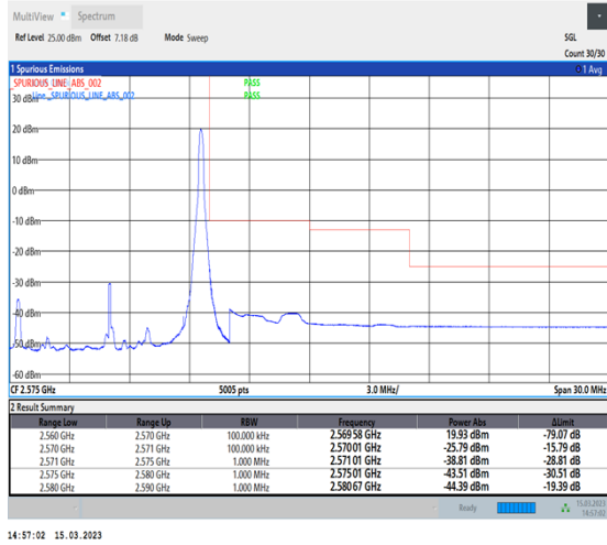
1-N7-PC3-15-10-H-2-DFT-PI2BPSK-Edge_1RB_Right-1@51-Ant1-1--PASS-see graph
