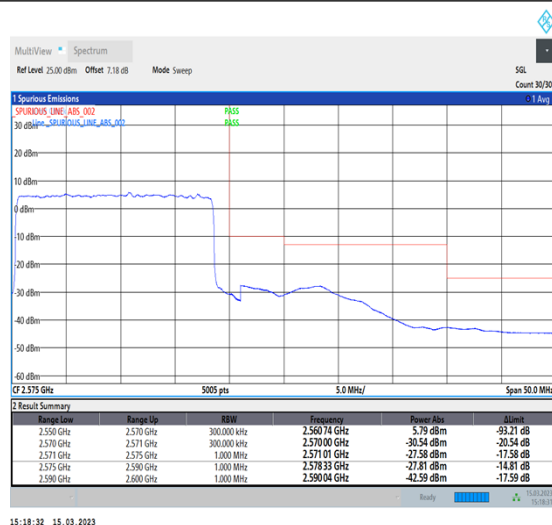
1-N7-PC3-15-20-H-3-DFT-PI2BPSK-Outer_Full-100@0-Ant1-1--PASS-see graph
