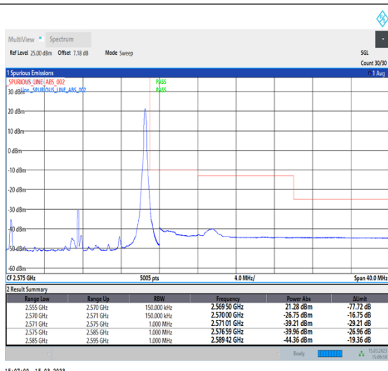
1-N7-PC3-15-15-H-2-DFT-PI2BPSK-Edge_1RB_Right-1@78-Ant1-1--PASS-see graph
