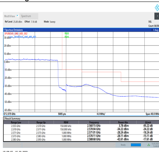
1-N7-PC3-15-15-H-3-DFT-PI2BPSK-Outer_Full-75@0-Ant1-1--PASS-see graph
