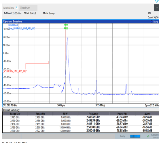
1-N7-PC3-15-15-L-4-CP-QPSK-Edge_1RB_Left-1@0-Ant1-1--PASS-see graph
