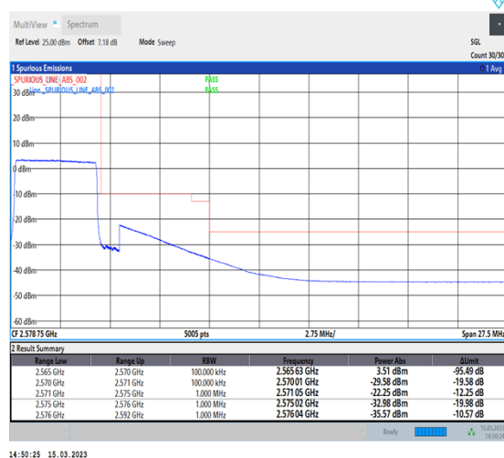
1-N7-PC3-15-5-H-6-CP-QPSK-Outer_Full-25@0-Ant1-1--PASS-see graph
