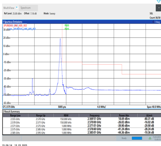
1-N7-PC3-15-15-H-5-CP-QPSK-Edge_1RB_Right-1@78-Ant1-1--PASS-see graph
