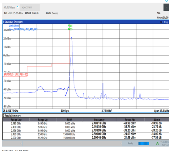
1-N7-PC3-15-15-L-1-DFT-PI2BPSK-Edge_1RB_Left-1@0-Ant1-1--PASS-see graph
