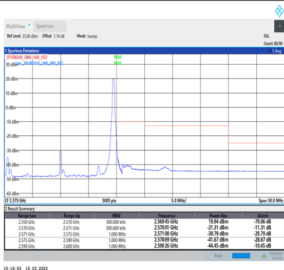
1-N7-PC3-15-20-H-2-DFT-PI2BPSK-Edge_1RB_Right-1@105-Ant1-1--PASS-see graph
