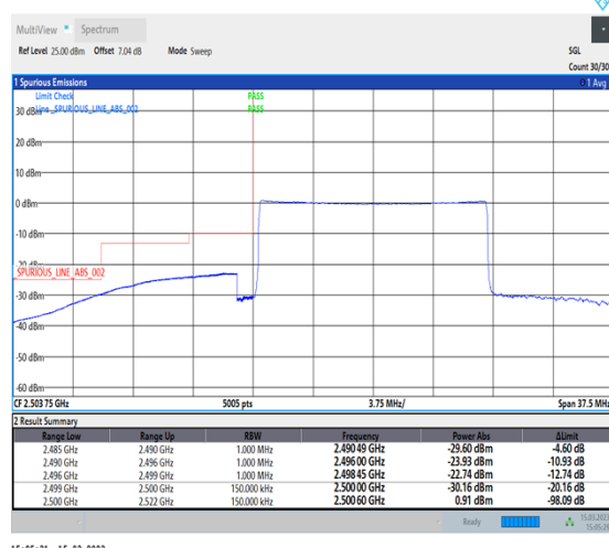
1-N7-PC3-15-15-L-6-CP-QPSK-Outer_Full-79@0-Ant1-1--PASS-see graph
