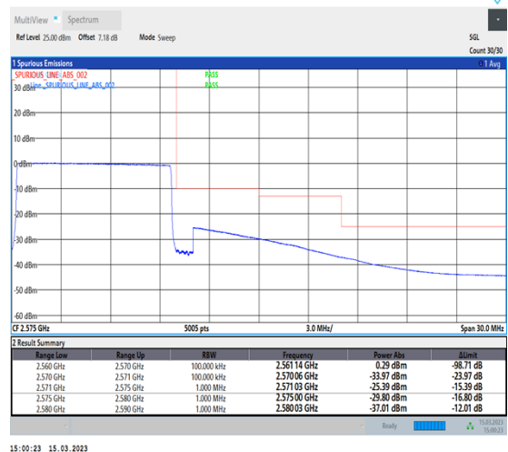
1-N7-PC3-15-10-H-6-CP-QPSK-Outer_Full-52@0-Ant1-1--PASS-see graph
