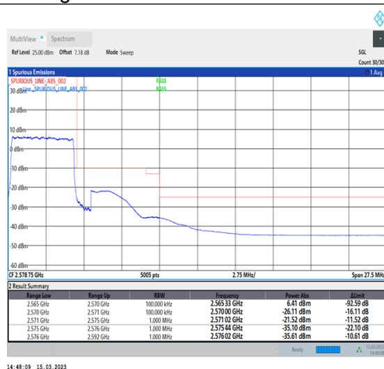
1-N7-PC3-15-5-H-3-DFT-PI2BPSK-Outer_Full-25@0-Ant1-1--PASS-see graph
