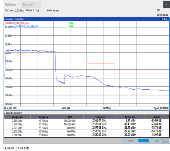
1-N7-PC3-15-10-H-3-DFT-PI2BPSK-Outer_Full-50@0-Ant1-1--PASS-see graph
