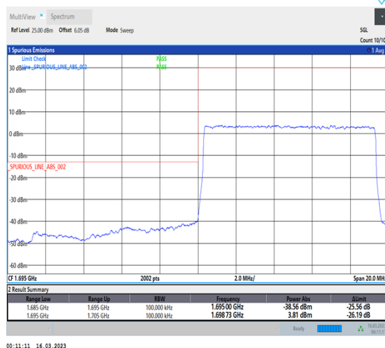
1-N70-PC3-15-10-L-3-DFT-PI2BPSK-Outer_Full-50@0-Ant7-1-seegraph-PASS-see graph
