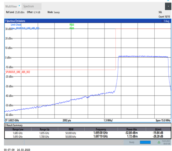
1-N70-PC3-15-5-L-6-CP-QPSK-Outer_Full-25@0-Ant7-1-seegraph-PASS-see graph
