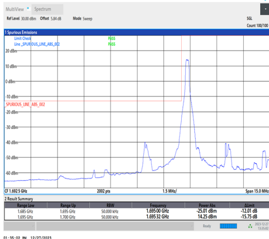
1-N70-15-5-L-1-DFT-PI2BPSK-Edge_1RB_Left-1@0-Ant7-1-seegraph-PASS-see graph
