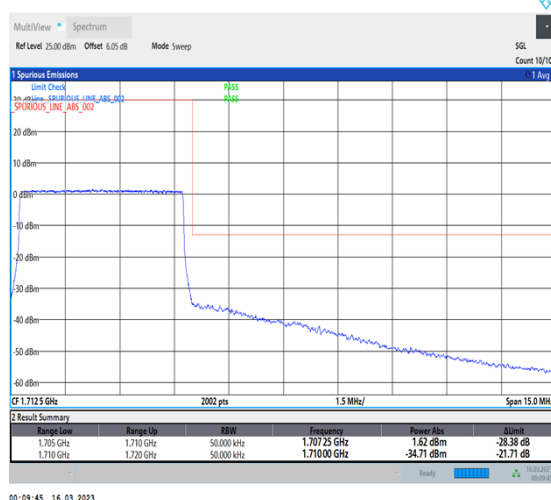
1-N70-PC3-15-5-H-6-CP-QPSK-Outer_Full-25@0-Ant7-1-seegraph-PASS-see graph
