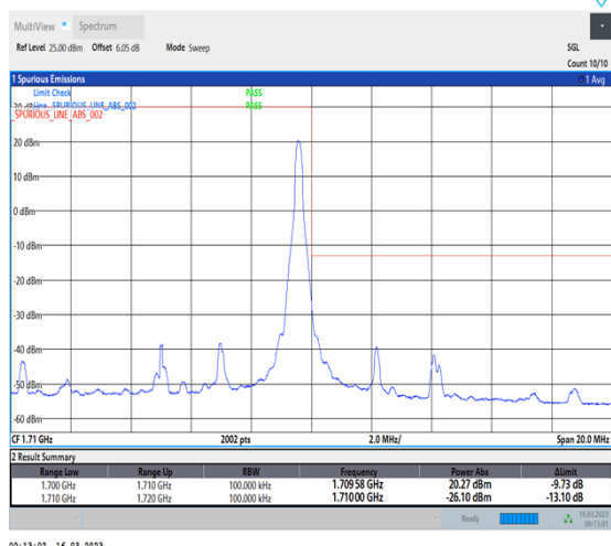
1-N70-PC3-15-10-H-2-DFT-PI2BPSK-Edge_1RB_Right-1@51-Ant7-1-seegraph-PASS-see graph
