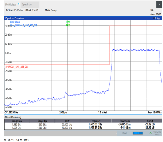
1-N70-PC3-15-5-L-3-DFT-PI2BPSK-Outer_Full-25@0-Ant7-1-seegraph-PASS-see graph
