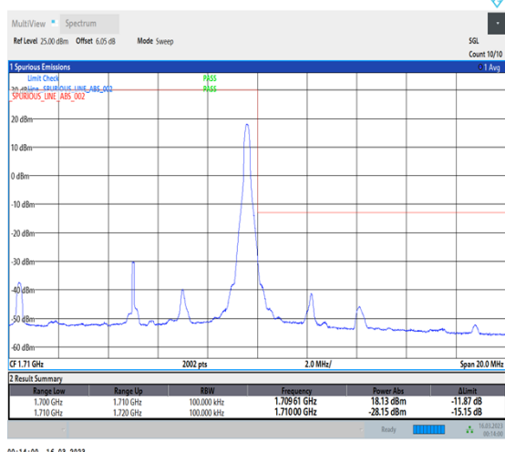
1-N70-PC3-15-10-H-5-CP-QPSK-Edge_1RB_Right-1@51-Ant7-1-seegraph-PASS-see graph
