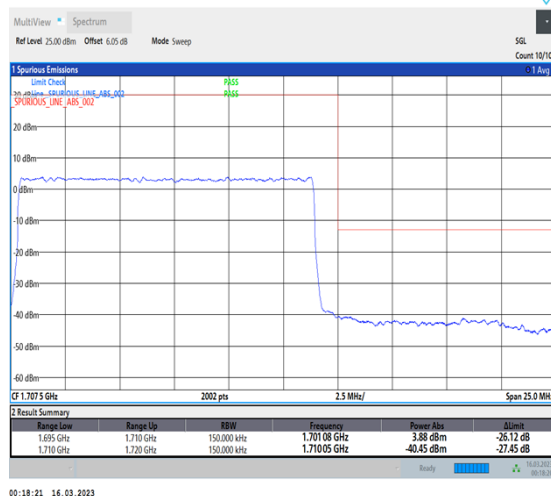
1-N70-PC3-15-15-H-3-DFT-PI2BPSK-Outer_Full-75@0-Ant7-1-seegraph-PASS-see graph
