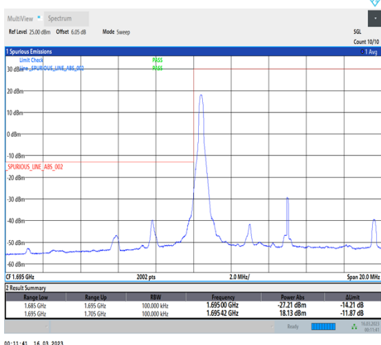
1-N70-PC3-15-10-L-4-CP-QPSK-Edge_1RB_Left-1@0-Ant7-1-seegraph-PASS-see graph
