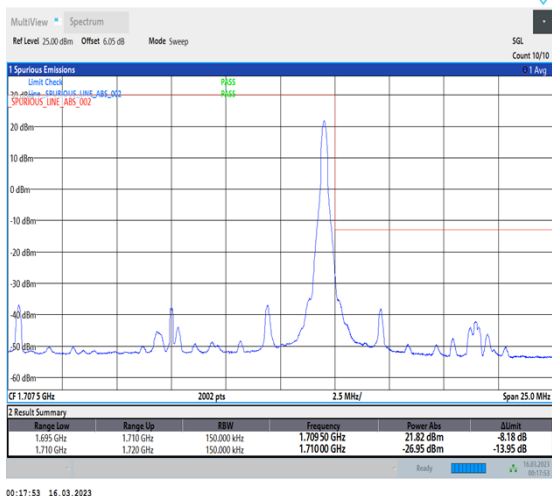
1-N70-PC3-15-15-H-2-DFT-PI2BPSK-Edge_1RB_Right-1@78-Ant7-1-seegraph-PASS-see graph
