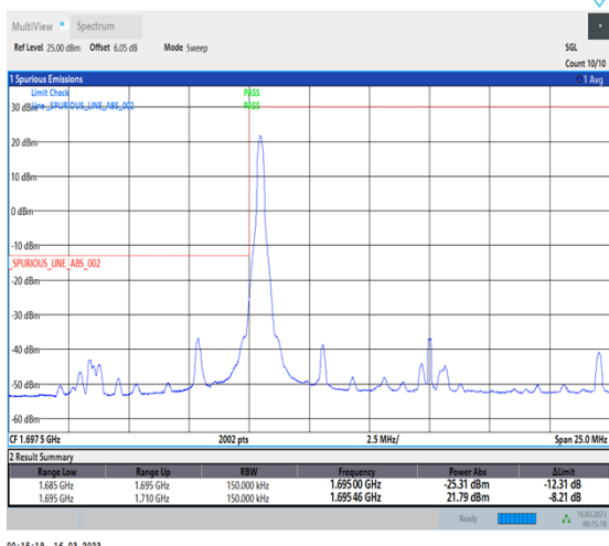
1-N70-PC3-15-15-L-1-DFT-PI2BPSK-Edge_1RB_Left-1@0-Ant7-1-seegraph-PASS-see graph
