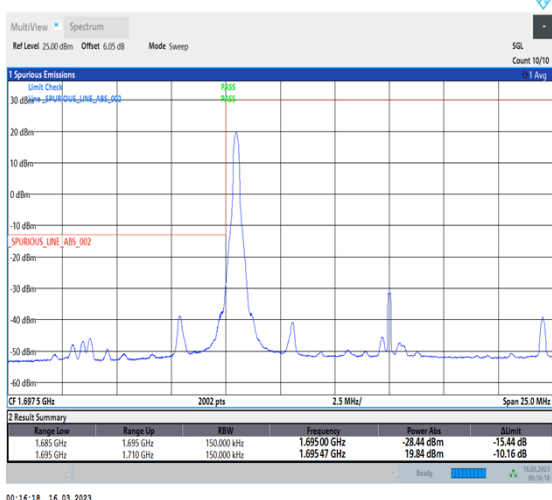
1-N70-PC3-15-15-L-4-CP-QPSK-Edge_1RB_Left-1@0-Ant7-1-seegraph-PASS-see graph
