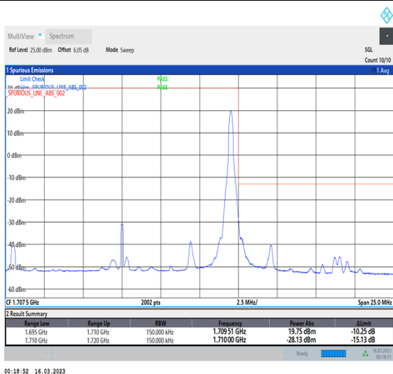
1-N70-PC3-15-15-H-5-CP-QPSK-Edge_1RB_Right-1@78-Ant7-1-seegraph-PASS-see graph
