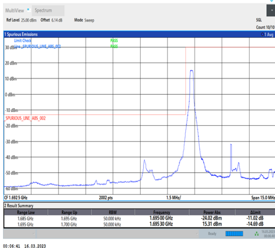
1-N70-PC3-15-5-L-4-CP-QPSK-Edge_1RB_Left-1@0-Ant7-1-seegraph-PASS-see graph
