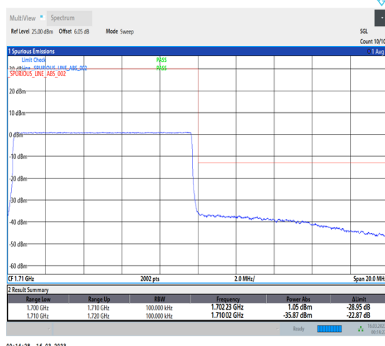
1-N70-PC3-15-10-H-6-CP-QPSK-Outer_Full-52@0-Ant7-1-seegraph-PASS-see graph
