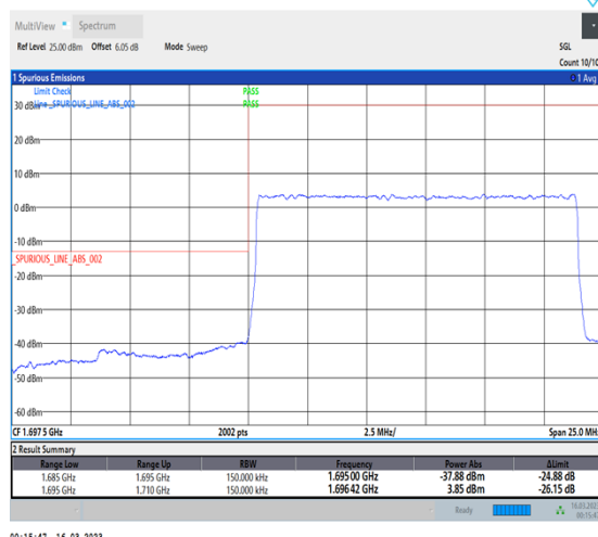
1-N70-PC3-15-15-L-3-DFT-PI2BPSK-Outer_Full-75@0-Ant7-1-seegraph-PASS-see graph
