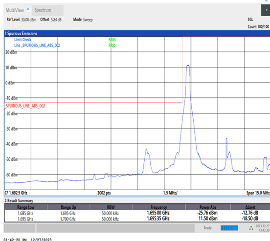
1-N70-15-5-L-4-CP-QPSK-Edge_1RB_Left-1@0-Ant7-1-seegraph-PASS-see graph
