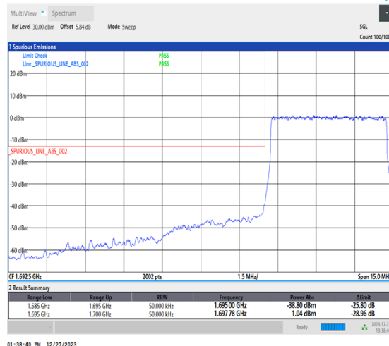
1-N70-15-5-L-3-DFT-PI2BPSK-Outer_Full-25@0-Ant7-1-seegraph-PASS-see graph
