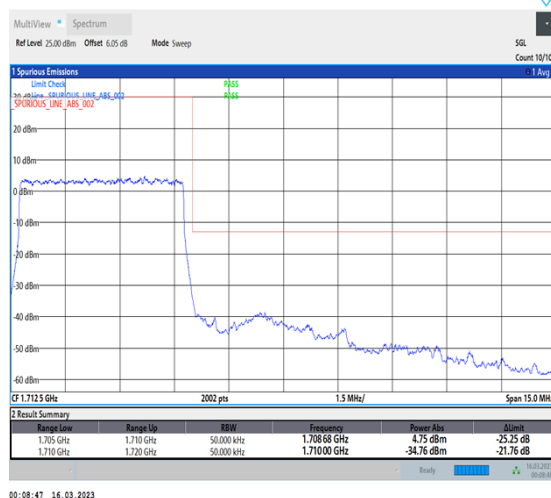
1-N70-PC3-15-5-H-3-DFT-PI2BPSK-Outer_Full-25@0-Ant7-1-seegraph-PASS-see graph
