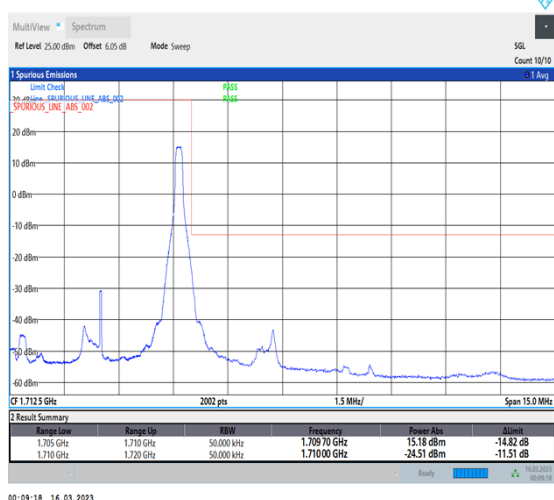
1-N70-PC3-15-5-H-5-CP-QPSK-Edge_1RB_Right-1@24-Ant7-1-seegraph-PASS-see graph
