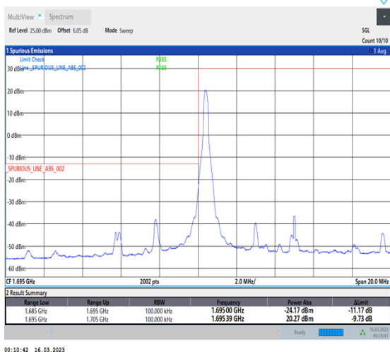
1-N70-PC3-15-10-L-1-DFT-PI2BPSK-Edge_1RB_Left-1@0-Ant7-1-seegraph-PASS-see graph
