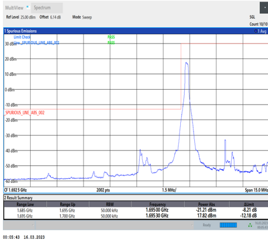
1-N70-PC3-15-5-L-1-DFT-PI2BPSK-Edge_1RB_Left-1@0-Ant7-1-seegraph-PASS-see graph
