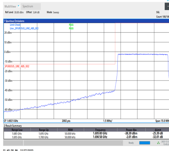
1-N70-15-5-L-6-CP-QPSK-Outer_Full-25@0-Ant7-1-seegraph-PASS-see graph
