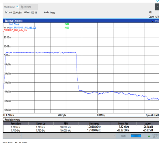
1-N70-PC3-15-10-H-3-DFT-PI2BPSK-Outer_Full-50@0-Ant7-1-seegraph-PASS-see graph
