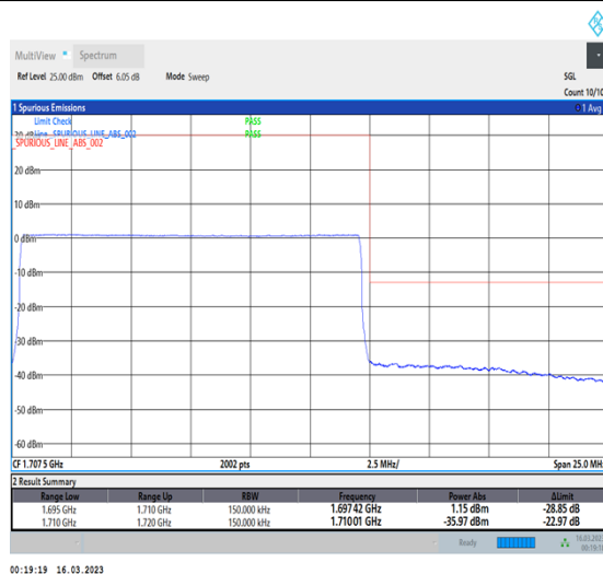
1-N70-PC3-15-15-H-6-CP-QPSK-Outer_Full-79@0-Ant7-1-seegraph-PASS-see graph
