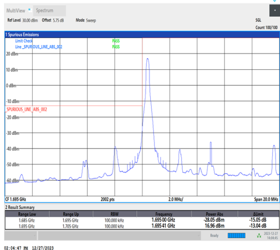
1-N70-15-10-L-1-DFT-PI2BPSK-Edge_1RB_Left-1@0-Ant7-1-seegraph-PASS-see graph
