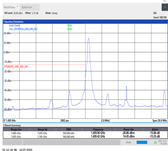
1-N70-15-10-L-4-CP-QPSK-Edge_1RB_Left-1@0-Ant7-1-seegraph-PASS-see graph
