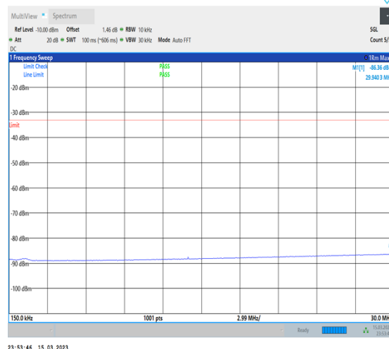
1-N70-PC3-15-15-L-1-DFT-PI2BPSK- Inner_1RB_Left-1@1-0.15-30-Ant7-29.94--86.36-- 33-PASS
