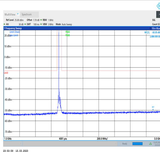
1-N70-PC3-15-15-L-1-DFT-PI2BPSK- Inner_1RB_Left-1@1-1000-3000-Ant7-2886.50-- 50.35--13-PASS
