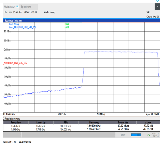
1-N70-15-10-L-6-CP-QPSK-Outer_Full-52@0-Ant7-1-seegraph-PASS-see graph
