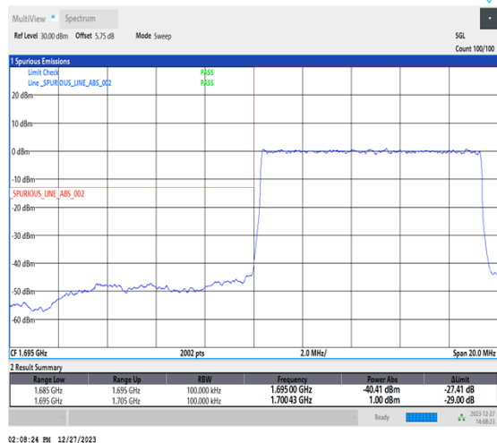
1-N70-15-10-L-3-DFT-PI2BPSK-Outer_Full-50@0-Ant7-1-seegraph-PASS-see graph
